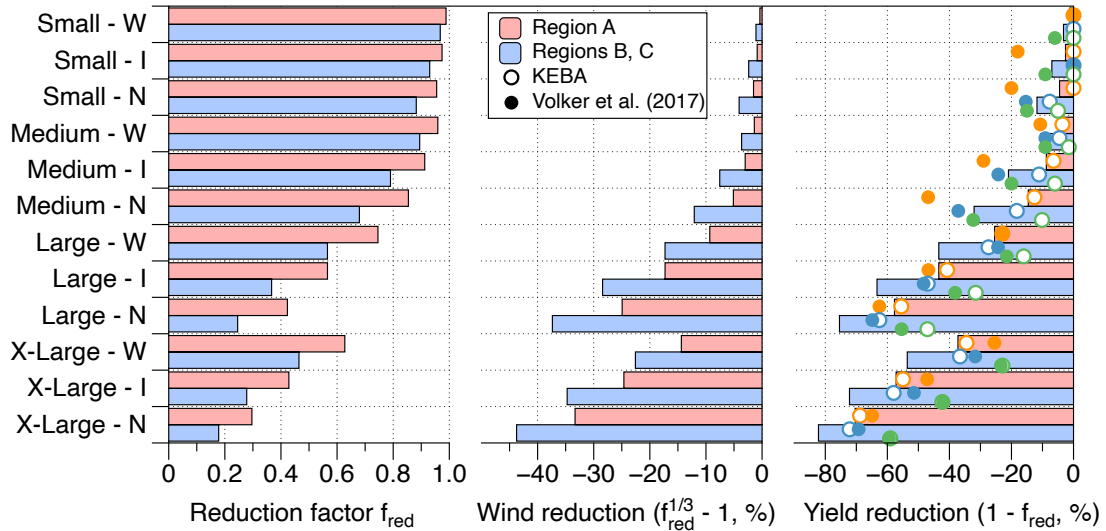
Figure 4. The value of the reduction factor f_{red} for the case in which v < v_{rated} (Eq. 9) for the different scenarios as well as the implied relative reduction in wind speed, f_{red}^{1/3} - 1 , and the relative reduction of yield, 1 - f_{red} , derived directly from the value of f_{red} . The circles in the right panel refer to the actual estimates that include the information of the wind speed histograms (open circles: KEBA; full circles: Volker et al. (2017)), with the color coding as in Fig. 3.
