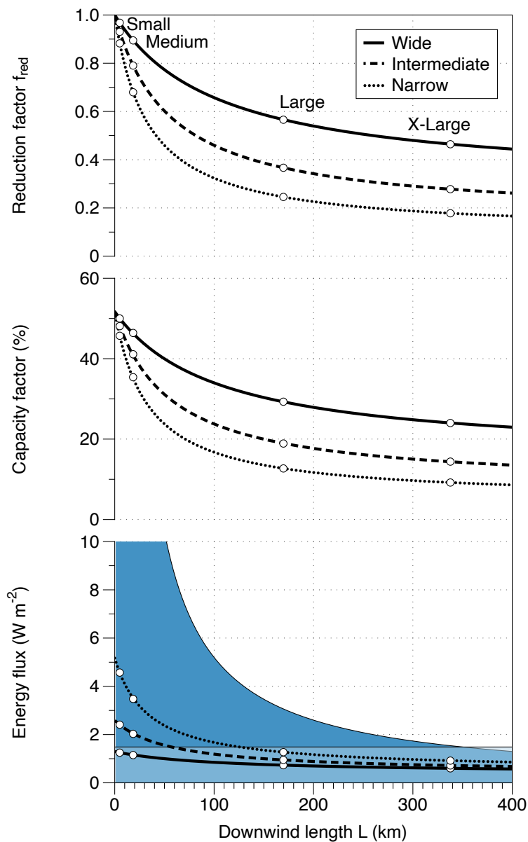
Figure 6. KEBA sensitivity to downwind length L for Region B (North Sea). The panels show the KEBA reduction factor f_{red} as a function of downwind length for three turbine spacings, the associated reduction in capacity factor ( P_{el}/NP_{el,max} ), and the supply of kinetic energy by the horizontal influx from upwind areas (dark blue) and by vertical mixing (light blue) as well as the yields by the wind farms (lines). The circles represent the different sizes of wind farms considered in the comparison with Volker et al. (2017).
