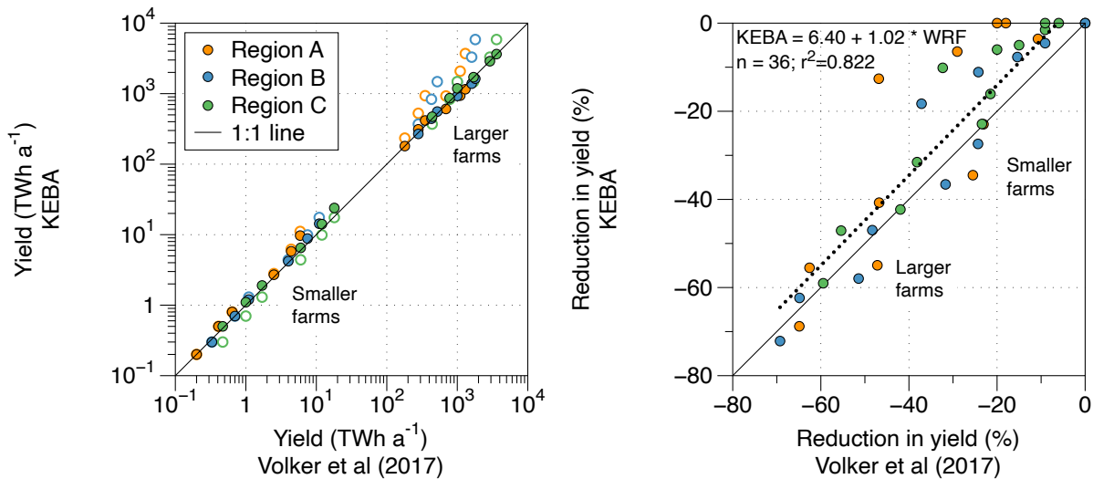
Figure 3. a. Comparison of yields for the scenarios of Table 2 estimated by KEBA and as reported by Volker et al. (2017). The open circles represent wind energy estimates that do not take wind speed reductions into account ("isolated", with f_{red} = 1 ). b. Relative yield reductions compared to the case of isolated turbines without the wind speed reduction effect. The dotted line reflects a linear regression between the two estimates, with the regression equation provided in the figure.
