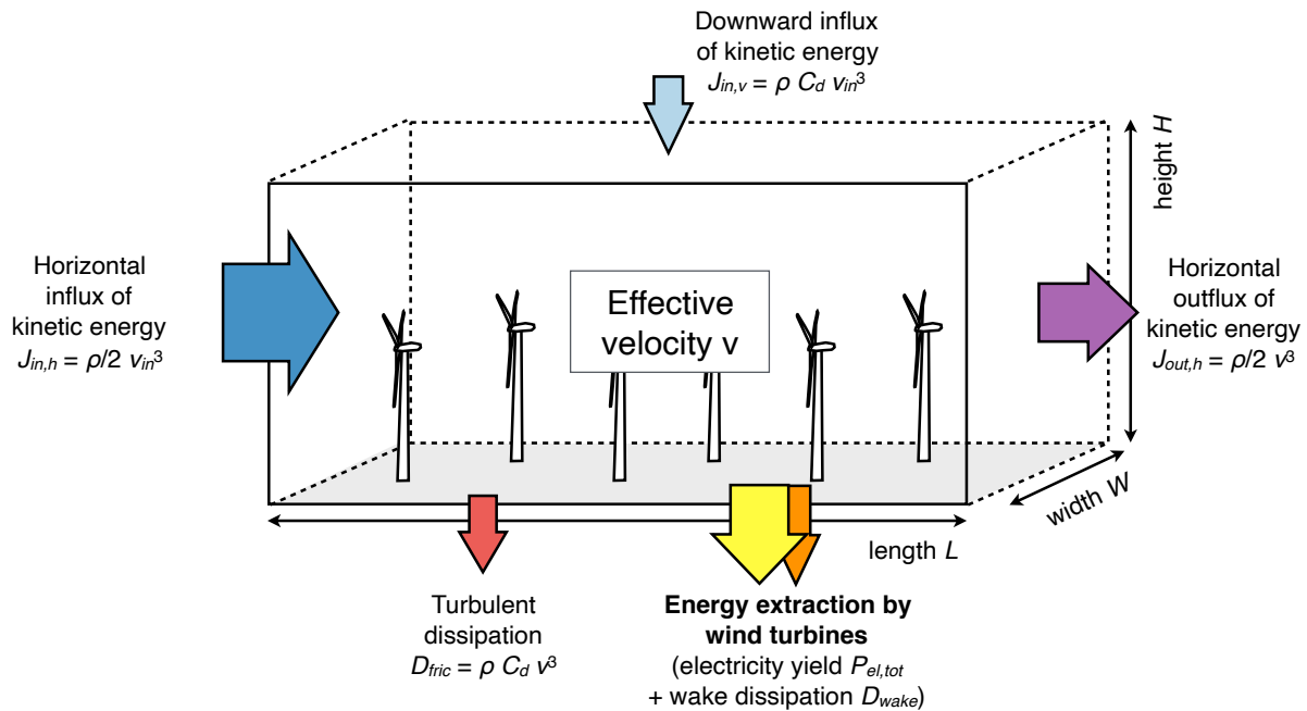
Figure 1. Illustration of the Kinetic Energy Budget of the Atmosphere (KEBA) approach to estimate regional wind energy potentials, which considers the fluxes of kinetic energy in and out of a virtual volume that encloses a given region of dimensions L \cdot W \cdot H to infer limits to electricity generation as well as wind speed reductions. The mathematical formulations of the fluxes are indicated at the arrows.
