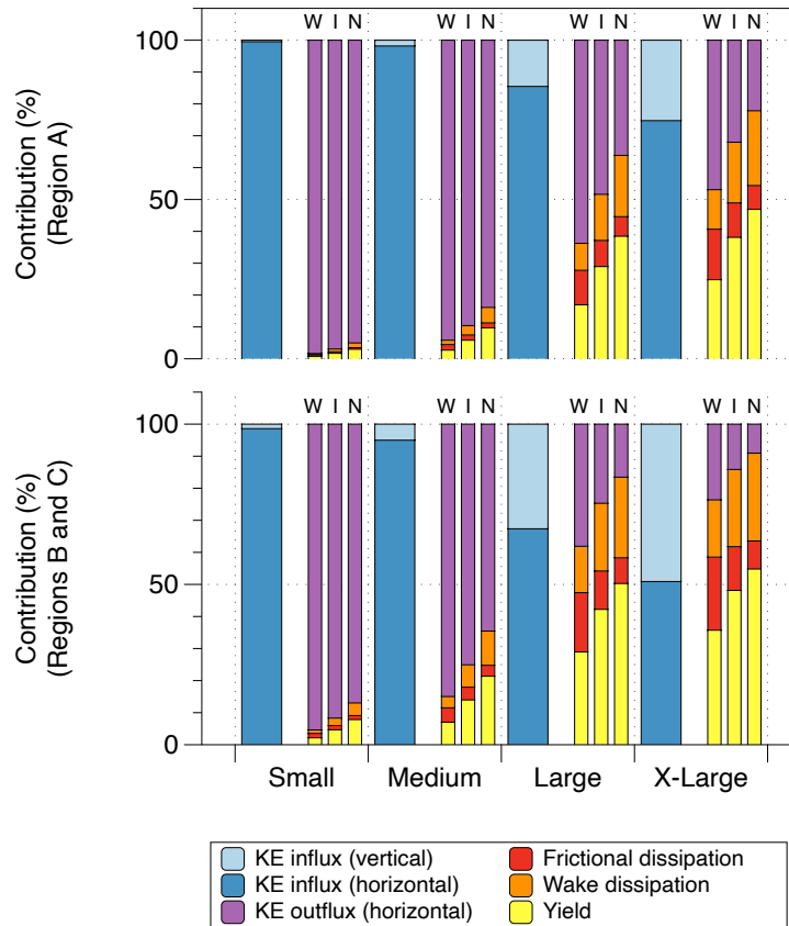
Figure 5. Diagnosed terms of the kinetic energy budget, with the relative contributions to the influxes of kinetic energy (KE) shown by the left column and the conversion to electricity, dissipation and outflux of kinetic energy shown by the three right columns (for three different turbine spacings: W: Wide; I: Intermediate; N: Narrow). The horizontal and vertical contributions to the KE influx are shown by dark and light blue respectively. The yield (conversion to electricity) is shown in yellow and the dissipation by surface friction (red) and wake turbulence (orange) and outflux of kinetic energy (purple). The plots show the KE budgets for the scenarios of wind farms of four different areas (S, M, L, and XL) for region A (Central US, land, a. ), and for regions B and C (North Sea and Strait of Magellan, ocean, b. ). The colors of the bars match the arrows shown in Fig. 1.
