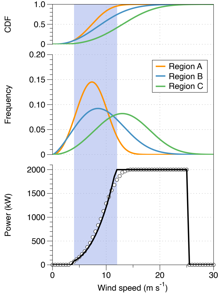
Figure 2. Wind forcing and turbine power curve used for the evaluation of KEBA. The top two panels show the frequency distribution of wind speeds for the three regions (A: Iowa, US (orange); B: North Sea (blue); C: Strait of Magellan (green)) considered here including their cumulative probability function (CDF) at the top. The lower panel shows the power curve used here for the Vestas V-80 2 MW wind turbines with a power coefficient of \eta = 0.44 , with the circles representing the actual power curve of the turbine (obtained from http://www.windpower.net ). Both form the inputs of the KEBA evaluation and are based on the data provided in Volker et al. (2017). The blue shaded region reflects wind speeds at which the turbine operates above its cut-in, but below its rated velocity.
