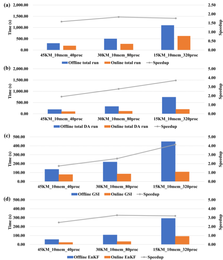
Figure 164. As in Fig. 13, but from experiment set 4 in Table 2.
