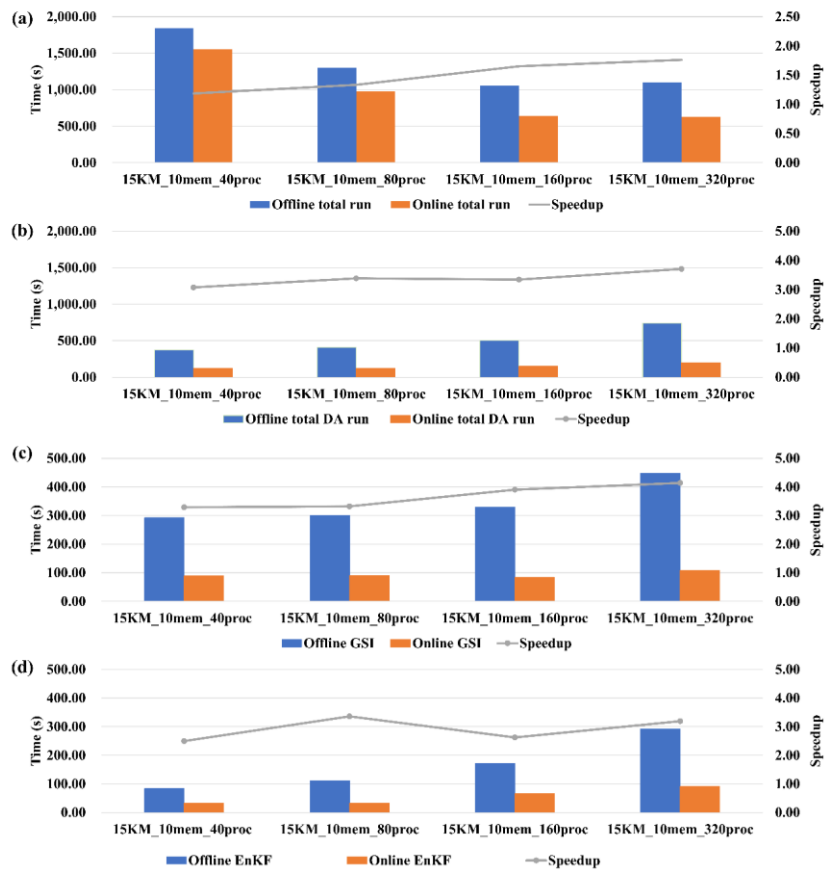
Figure 142. As in Fig-14Fig. 13, but from experiment set 2 in Table 2.
