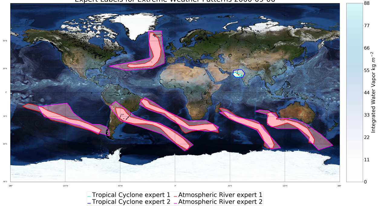
Figure 6. Comparison of two different expert labelings with an IoU of 0.59. Note that even though, visually, the experts appear to agree to a large extent on their labels of AR and TC events in this snapshot, the quantitative IoU metric is only 0.59. Hence we emphasize that IoU not be confused with accuracy; good agreement even amongst expert labelers can result in IoU values far from unity. A perfect match, i.e. \text{IoU} = 1 only results when two labelers agree on every single pixel of the image. As is apparent from this figure, even relatively minor differences in the labels for TCs can disproportionately impact the mean IoU. The “blumarble” map in the background included via Matplotlib’s Basemap library is ©NASA.
