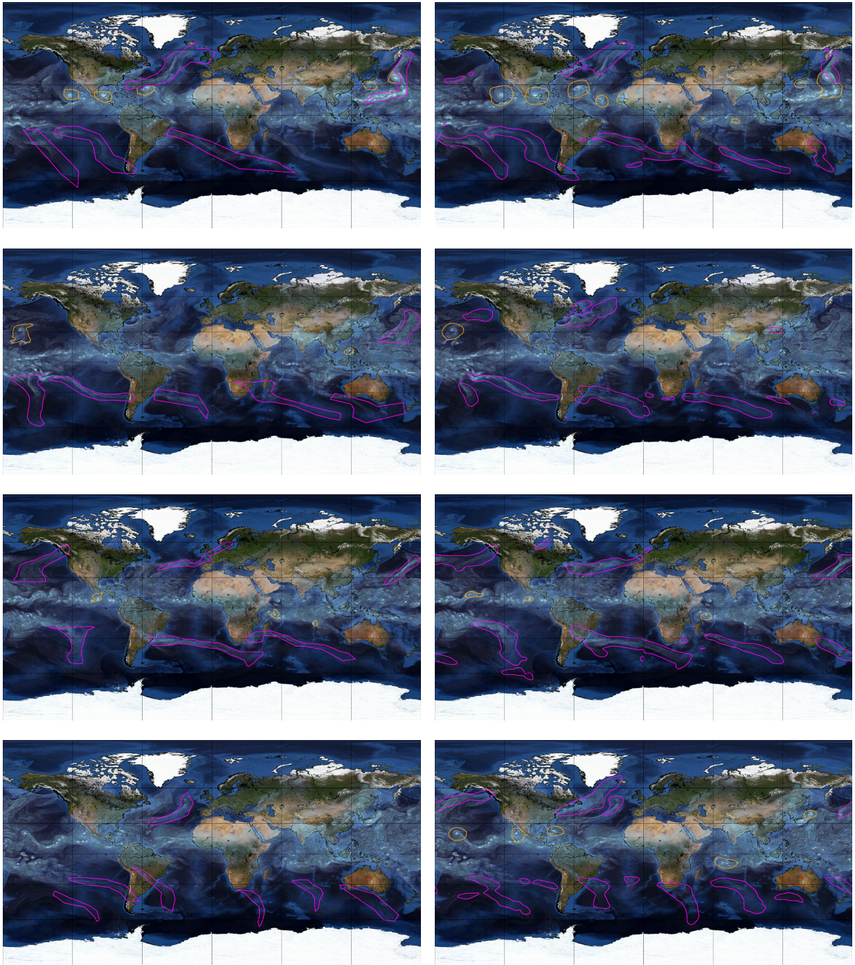
Figure 4. Comparison of expert labels from the ClimateNet dataset (left column) and DL segmentation model predictions (right column). The “bluemarble” map in the background included via Matplotlib’s Basemap library is ©NASA.
