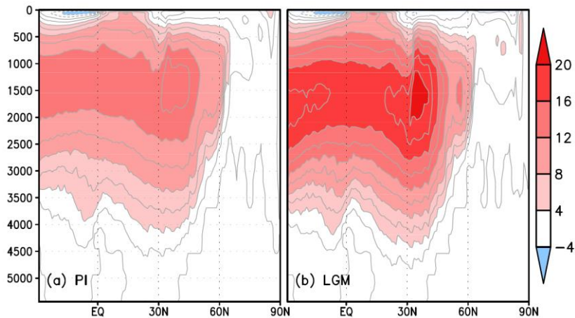
Figure 7: Meridional overturning streamfunction for the Atlantic Basin (unit: \text{Sv} ) for (a) PI and (b) LGM.
