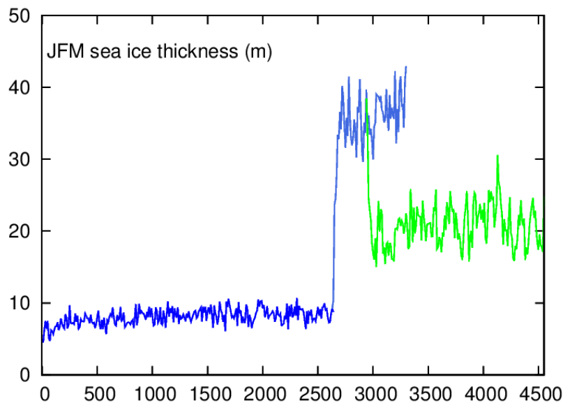
Figure A1: Average sea ice thickness (m) from January to March for the first half of the spin-up of the LGM experiment, averaged 150^{\circ} - 180^{\circ}\text{E} , 70^{\circ} - 75^{\circ}\text{N} . The blue line: step 1, light blue: step 2, and yellow-green: step 3 in Figure 5, respectively. For simplicity, data for one year for every 10 years are plotted.
