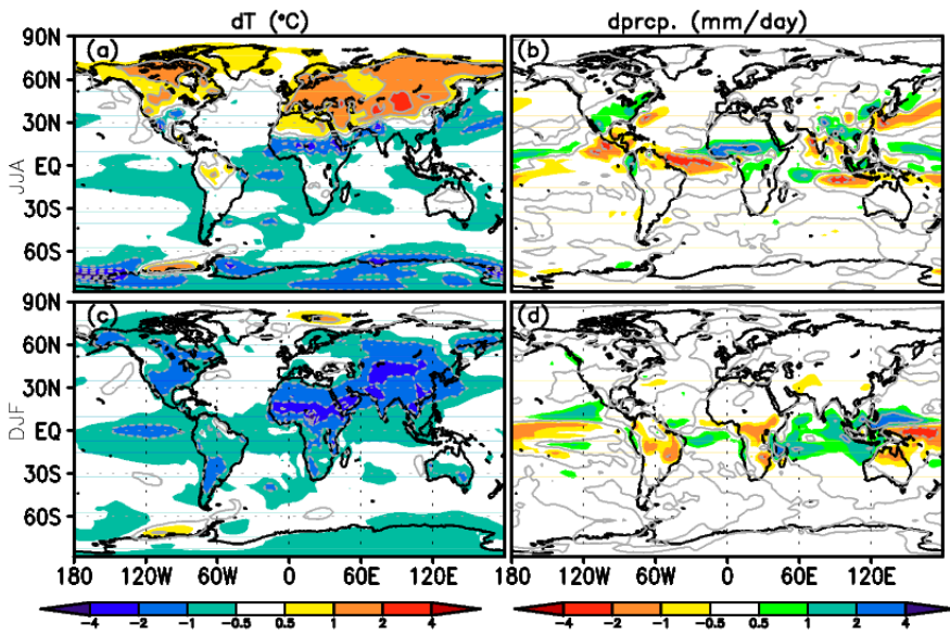
840 Figure 10: Seasonal temperature anomaly for (a) JJA and (c) DJF. Seasonal precipitation anomaly for (b) JJA and (d) DJF. Anomalies are calculated as 6ka relative to PI values. Calendar adjustments are applied.
