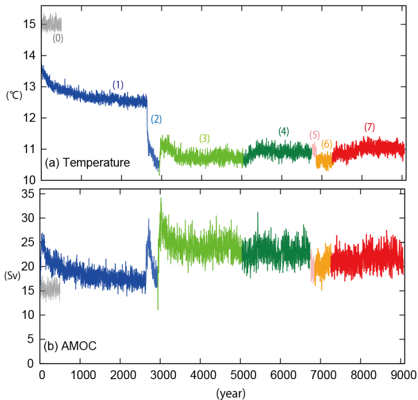
805 Figure 5: Time series for spin-up and submitted period (final 100 years) of LGM experiment and PI as a reference for (a) global mean air temperature at 2 m height and (b) peak values of annual mean AMOC. Gray line (0) denotes PI value. Blue line (1): the experiment with only GHG levels set to LGM values. Light blue line (2): with the land–sea distribution and land PFTs hanged to the LGM states. Light green line (3): with altitude set to the LGM state. Dark green line (4): with orbit of the Earth set to the LGM value. Pink line (5): spin-up experiment using MIROC-ES2L after VISIT-e offline spin-up. Orange line (6): with erodibility map and offset of ocean salinity applied. Red line (7): final spin-up after offline spin-up experiments by VISIT-e and OECO2.
