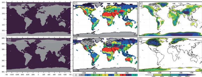
785 Figure 2: Left panels: Land–sea distribution converted to 1^\circ \times 1^\circ ocean grids for (a) PI, 6ka, and 127ka and (b) LGM. Middle panels: Distribution of land vegetation types for (c) PI, 6ka, and 127ka and (d) LGM. Numbers in color bar represent vegetation types: 1) ice sheets, 2) broadleaf evergreen forest, 3) broadleaf deciduous forest and woodland, 4) mixed coniferous and broadleaf deciduous forest and woodland, 5) coniferous forest and woodland, 6) high-latitude deciduous forest and woodland, 7) wooded C4 grassland, 8) shrubs and bare ground, 9) tundra, and 10) C3 grassland. Right panels: (e) Altitude for PI, 6ka, and 127ka and LM (unit: m) and 790 (f) altitude anomaly (unit: m) given for the LGM experiment based on ICE-6G_C (Peltier, 2015).
