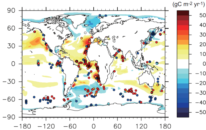
820 Figure 9: Primary production anomaly of the oceanic ecosystem (unit: \text{gC m}^{-2} \text{yr}^{-1} ). Anomalies are calculated as LGM relative to PI values. Circles denote qualitative changes in primary production derived from proxy data (Kohfeld et al., 2013).
