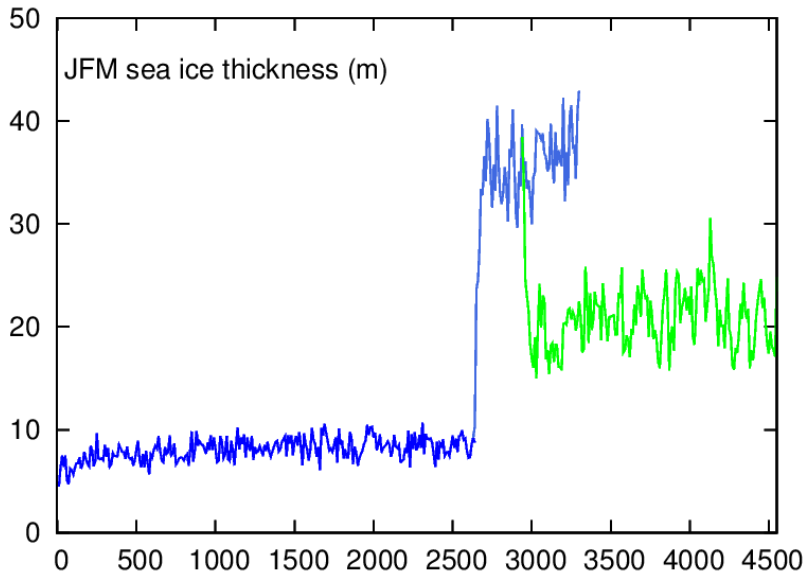
845 Figure A1: Average sea ice thickness (m) from January to March for the first half of the spin-up of the LGM experiment, averaged 150° - 180° E, 70° -75° N. The blue line: step 1, light blue: step 2, and yellow-green: step 3 in Figure 5, respectively. For simplicity, data for one year for every 10 years are plotted.
