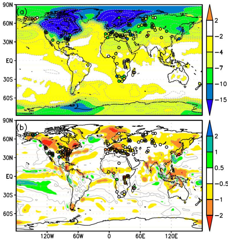
810 Figure 6: (a) Air temperature anomaly at 2 m height (unit: °C) and (b) precipitation anomaly (unit: mm d -1 ). Anomalies are calculated as LGM relative to PI values. Circles denote values derived from proxy data (Bartlein et al., 2011).
