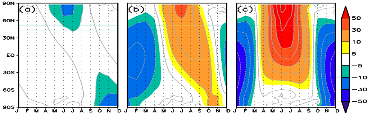
Figure 3: Variation of incoming shortwave solar radiation anomaly relative to PI (unit: \text{W m}^{-2} ) with season and latitude for (a) LGM, (b) 6ka, and (c) 127ka.
