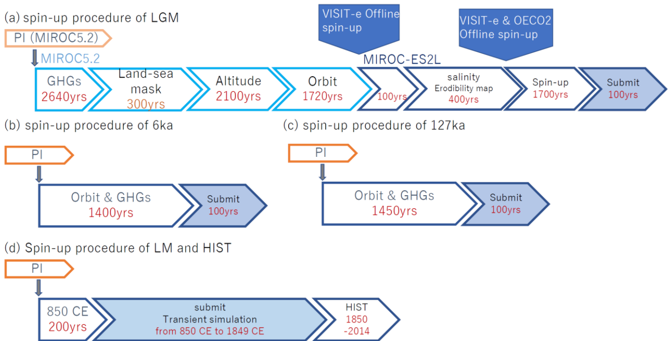
865 Figure 4: Schematic showing spin-up procedures of the following experiments: (a) LGM, (b) 6ka, (c) 127ka, and (d) LM and HIST. Shapes with dark orange or dark blue outlines represent experiments using MIROC-ES2L. Shapes with light orange or light blue outlines represent experiments using MIROC5.2. Shapes filled in pale blue represent model output submitted to PMIP4–CMIP6.
