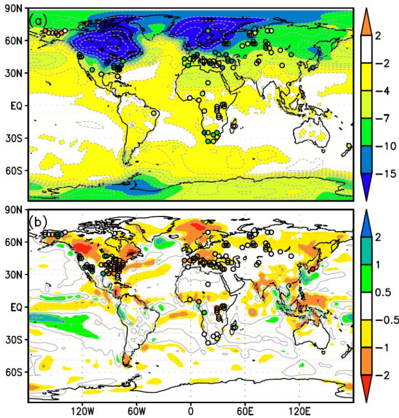
880 Figure 6: (a) Air temperature anomaly at 2 m height (unit: °C) and (b) precipitation anomaly (unit: mm d -1 ). Anomalies are calculated as LGM relative to PI values. Circles denote values derived from proxy data (Bartlein et al., 2011).
