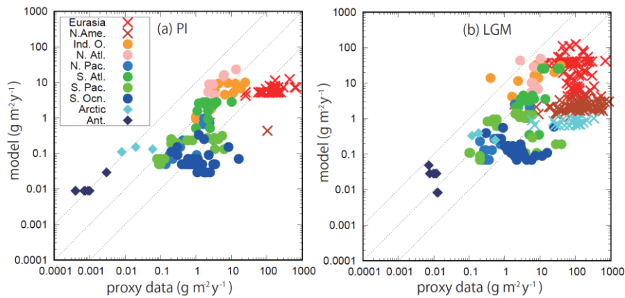
885 Figure 8: Dust deposition from model output and derived from proxy archives (Kohfeld et al., 2013; Albani et al., 2014) for (a) PI and (b) LGM ( \text{g m}^{-2} \text{yr}^{-1} ). Colors represent the locations of the proxy data, as explained in the legend in the figure. Crosses, circles, and diamonds represent terrestrial, marine, and ice core data.
