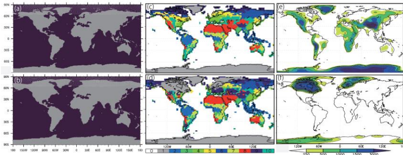
855 Figure 2: Left panels: Land–sea distribution converted to 1^\circ \times 1^\circ ocean grids for (a) PI, 6ka, and 127ka and (b) LGM. Middle panels: Distribution of land vegetation types for (c) PI, 6ka, and 127ka and (d) LGM. Numbers in color bar represent vegetation types: 1) ice sheets, 2) broadleaf evergreen forest, 3) broadleaf deciduous forest and woodland, 4) mixed coniferous and broadleaf deciduous forest and woodland, 5) coniferous forest and woodland, 6) high-latitude deciduous forest and woodland, 7) wooded C4 grassland, 8) shrubs and bare ground, 9) tundra, and 10) C3 grassland. Right panels: (e) Altitude for PI, 6ka, and 127ka and LM (unit: m) and (f) altitude anomaly (unit: m) given for the LGM experiment based on ICE-6G_C (Peltier, 2015).
