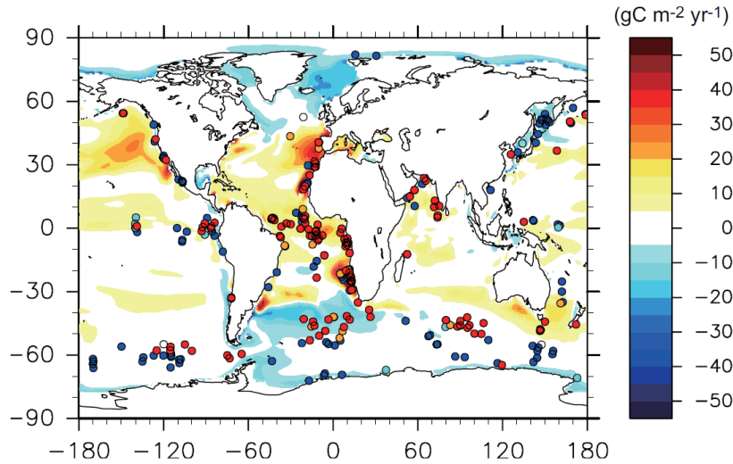
890 Figure 9: Primary production anomaly of the oceanic ecosystem (unit: \text{gC m}^{-2} \text{yr}^{-1} ). Anomalies are calculated as LGM relative to PI values. Circles denote qualitative changes in primary production derived from proxy data (Kohfeld et al., 2013).
