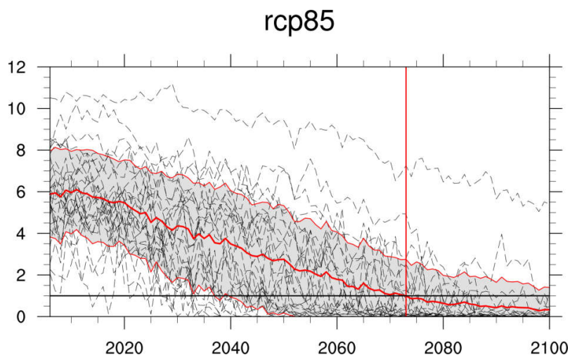
Figure 20 Time series of September Arctic sea ice extent for individual CMIP5 models (gray dashed lines), multi-model mean (thick red line) and multi-model standard deviation (area shaded between thin red lines) for scenario RCP8.5. The year of disappearance (sea ice extent below 1 million km 2 ) obtained from the CMIP5 multi-model mean is indicated by the vertical red line (similar to Collins et al. (2013), figure 12.31e). Produced with recipe_seaice.yml , for details see Section 3.4.4.
