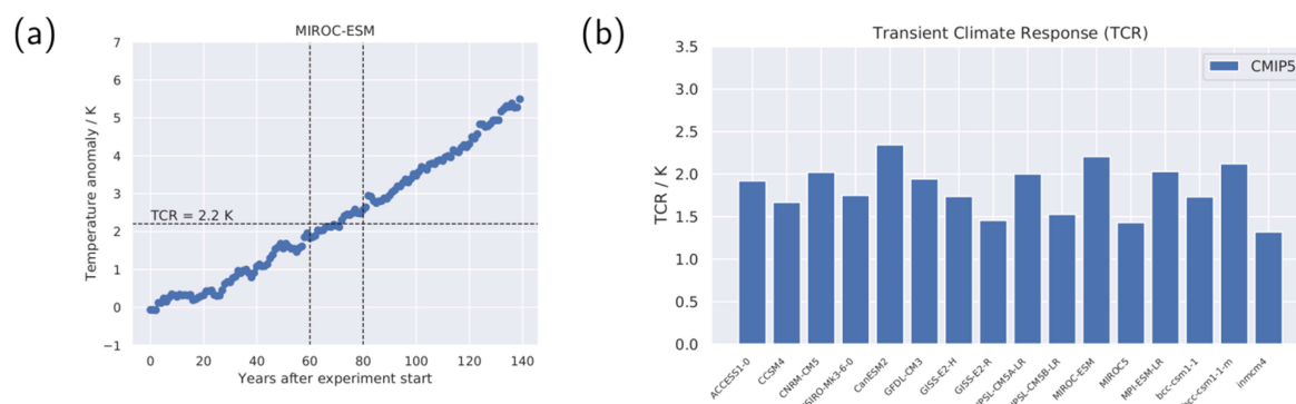
Figure 5 (a) Time series of temperature anomalies from MIROC-ESM experiment 1pctCO2 (1% increase in CO 2 per year) compared to the piControl simulation. (b) Transient climate response (in K) for CMIP5 models calculated with the method by Gregory and Forster (2008). For details on recipe_tcr.yml see Section 3.2.
