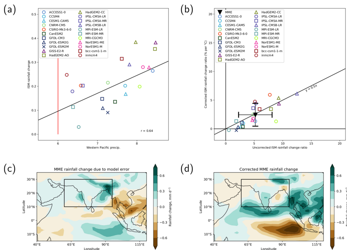
Figure 14 Correction of the Indian Summer Monsoon (ISM, 60°–95°E, 10°–30°N) rainfall projected by models for the RCP8.5 scenario based on the bias in present-day precipitation over the tropical western Pacific (140°E–170°W, 12°S–12°N). (a) Scatter plot and the linear regression (black line, with the correlation coefficient r ) of the western Pacific precipitation (mm day -1 ) from the CMIP5 historical simulations (1980–2005) and the ISM rainfall change between historical and the RCP8.5 for the years 2070–2099 for different CMIP5 models. The red line indicates the present-day value for the western Pacific precipitation from observations as used in Li et al. (2017) estimated from the Global Precipitation Climatology Project (GPCP) dataset for 1980–1999 (Adler et al., 2003). (b) Uncorrected ISM rainfall change ratio (% per °C) vs. the corrected ratio from CMIP5 models and the multi-model mean (MME) with the standard deviations shown as error bars. The rain data are normalized by the global mean near-surface temperature change. (c) Projected multi-model mean rainfall change errors and (d) corrected multi-model mean rainfall change over the Indian Ocean. Similar to figure 2 of Li et al. (2017) and produced with recipe_li2017natcc.yml (see details in Section 3.3.5).
