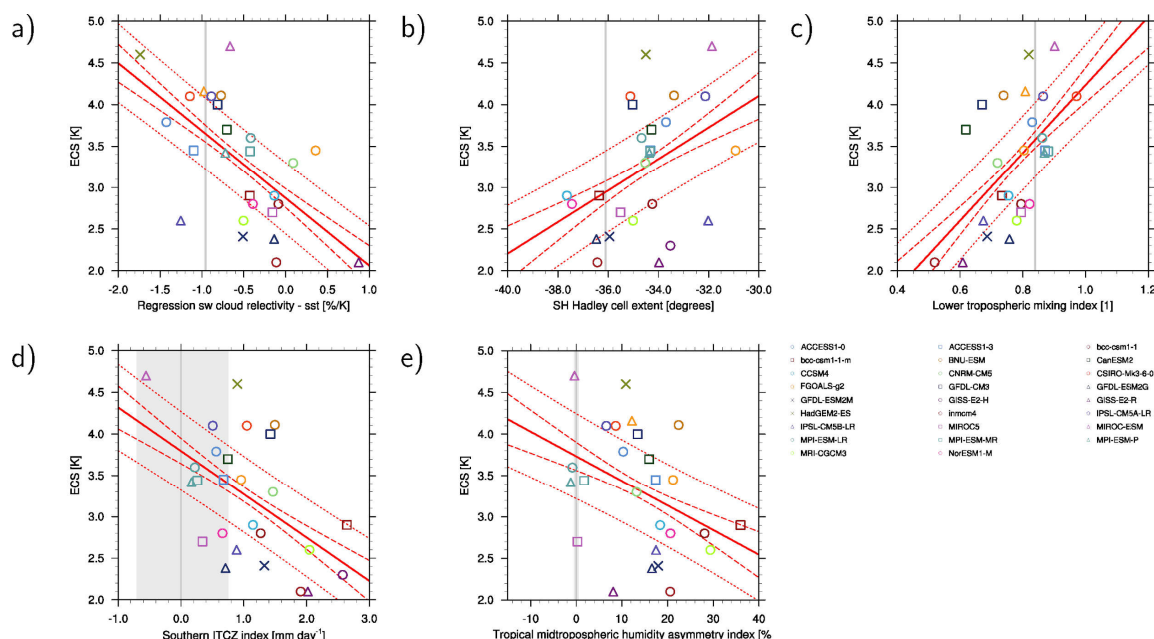
Figure 6 Scatterplots of effective climate sensitivity (ECS) vs. (a) covariance of shortwave cloud reflection (Brient and Schneider, 2016), (b) Southern Hemisphere (SH) climatological Hadley cell extent (Lipat et al., 2017), (c) lower tropospheric mixing index (LTMI) (Sherwood et al., 2014), (d) southern ITCZ index (Tian, 2015), and (e) tropical mid-tropospheric humidity asymmetry index (Tian, 2015) for CMIP5 models (symbols). The vertical gray lines represent the observations, the shaded areas in light-gray observational uncertainties (if available). The solid red lines represent the regression lines, the dashed red lines the 25% / 75% confidence intervals of the regression and the red dotted lines the 25% / 75% prediction intervals of the regression. Similar to (a) figure 6 of Brient and Schneider (2016), (b) figure 4 of Lipat et al. (2017), (c) figure 5c of Sherwood et al. (2014), (d) figure 2 of Tian (2015), and (e) figure 4c of Tian (2015). For details on recipe_ecs_scatter.yml see Section 3.3.1.
