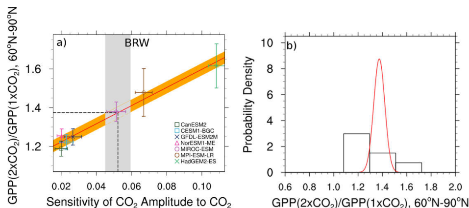
Figure 10 (a) Correlations between the sensitivity of the CO 2 amplitude to annual mean CO 2 increases at Point Barrow, Alaska (abscissa) and the high-latitude (60°N-90°N) CO 2 fertilization on gpp at 2 × CO 2 . The gray shading shows the range of the observed sensitivity. The red line shows the linear best fit across the CMIP5 ensemble together with the prediction error (orange) and error bars show the standard deviation for each data point. (b) The probability density histogram for the unconstrained CO 2 fertilization of gpp (black) and the conditional probability density function arising from the emergent constraint (red). Produced with recipe_wenzel16nat.yml, similar to figure 3 of Wenzel et al. (2016a) (for details see Section 3.3.2).
