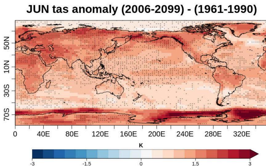
Figure 1 Multi-model mean of projected future June near-surface air temperature anomalies (2006-2099) compared with the period 1961-1990 (colors). Crosses indicate that the 80% of models agree with the sign of the multi-model mean anomaly. The models used in this example are BCC-CSM1-1, MPI-ESM-MR and MIROC5 (r11p1 ensembles) for the RCP2.6 scenario. All models have been regridded to the BCC-CSM1-1 grid using a linear interpolation scheme. See Section 3.4.2 for details on recipe_multimodel_products.yml .
