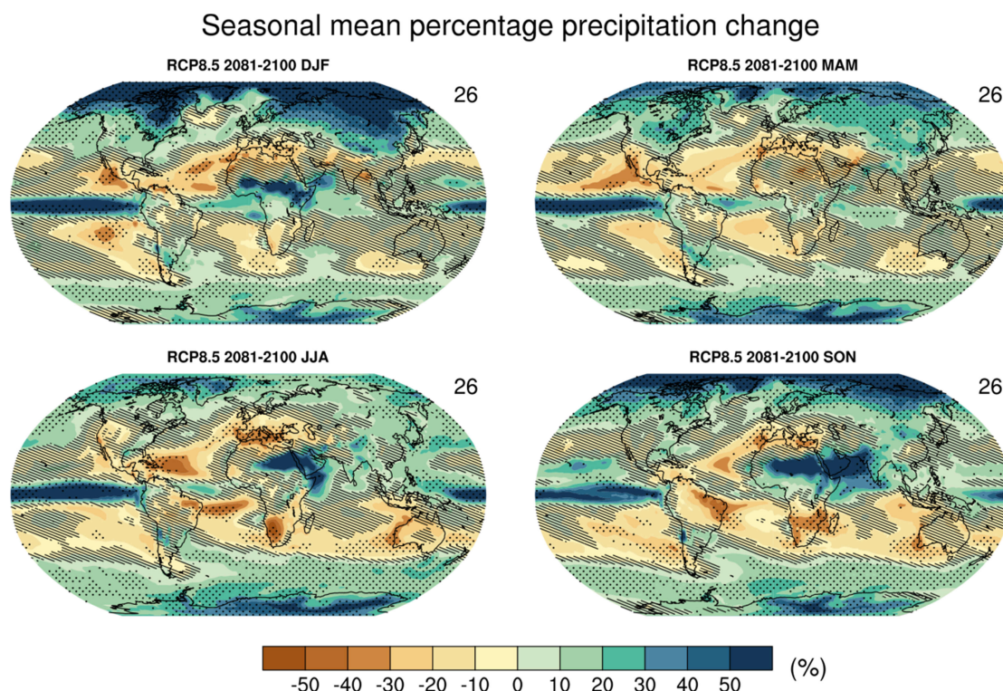
Figure 18 Global maps of seasonal mean change in precipitation from 1986-2005 (reference period) to 2081-2100 for the RCP8.5 scenario. Hatching indicates regions where the multi-model mean change is less than one standard deviation of the internal variability estimated from piControl simulations. Stippling indicates regions where the multi-model mean change is greater than two standard deviations of the internal variability and where at least 90% of models agree on the sign of the change. The numbers in the upper right of each panel indicate the number of models used. Similar to Collins et al. (2013) figure 12.22 but only for one future time period. Produced with recipe_collins13ipcc.yml (see Section 3.4.3 for details).
