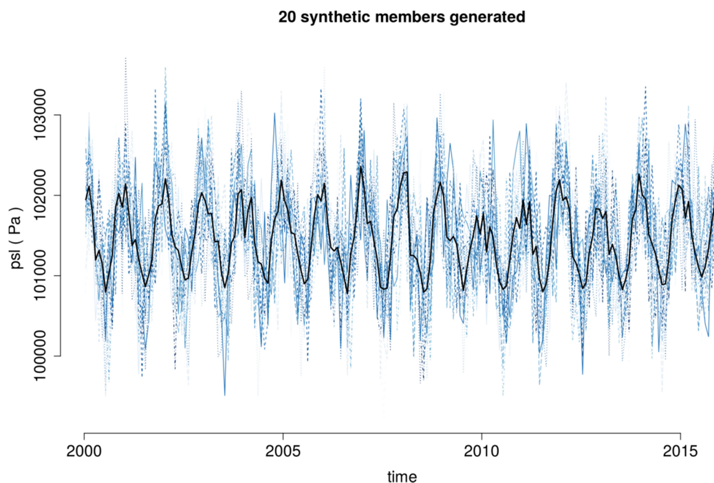
860 Figure 16 Example of 20 synthetic members of a single dataset ensemble generated by recipe_toymodel.yml . Shown are time series of surface-level pressure (psl) averaged over the region 40°E-40°W, 30°N-50°N from 2000-2015 created from monthly mean data from ERA-Interim (Dee et al., 2011). With the user providing an estimate for the standard error e.g. from differences between different observational datasets, this diagnostic can be used to investigate the effect of observational uncertainty. For details see Section 3.4.2.
