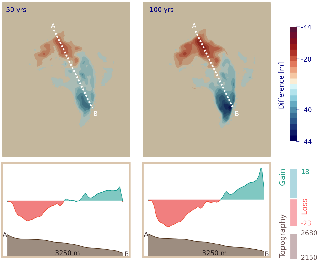
Figure 8. Test 1 (zero mass balance rate) Zero Mass Balance : top view of difference between initial surface elevation and simulation results at time steps 50 years and 100 years and corresponding profiles with shaded surface topography in brown in the lower panels.
