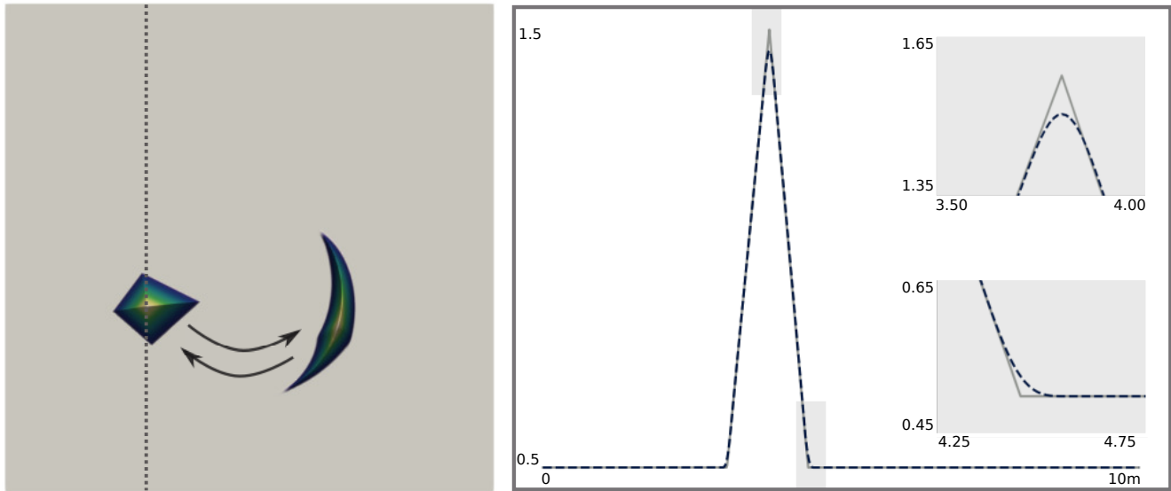
Figure 7. Test BSwirling Flow : Left panel shows top view of simulation results for the 10 m x 10 m domain at time steps 0 s and 0.75 s. The dashed vertical line indicates the location of the respective profiles of the simulation results (dashed blue line) and the analytical solution (grey line) at the final time step of 1.5 s shown in the right panel. The two small inserts show zooms of the grey rectangles on the main panel.
