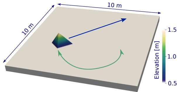
Figure 2. Initial 3D geometry for benchmark tests with surface elevation in colour and arrows indicating the direction of movement for Test A-Pyramid Translation in blue and for Test B-Swirling Flow in green.
