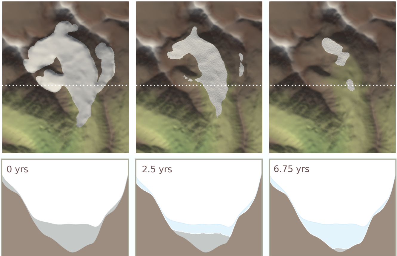
Figure 10. Test 3 ( random mass balance rate ) Random Input Fields : top view of surface elevation that exceeds the bed constraint in white and bed constraint in colour at the start of the simulation, at 2.5 years and 6.75 years. Corresponding profiles of surface elevation (silver), bed constraint (brown) and initial surface elevation (light blue) in the lower panels. The elevation on the y-axis is shown on a 4:1 scale, thus quite exaggerated.
