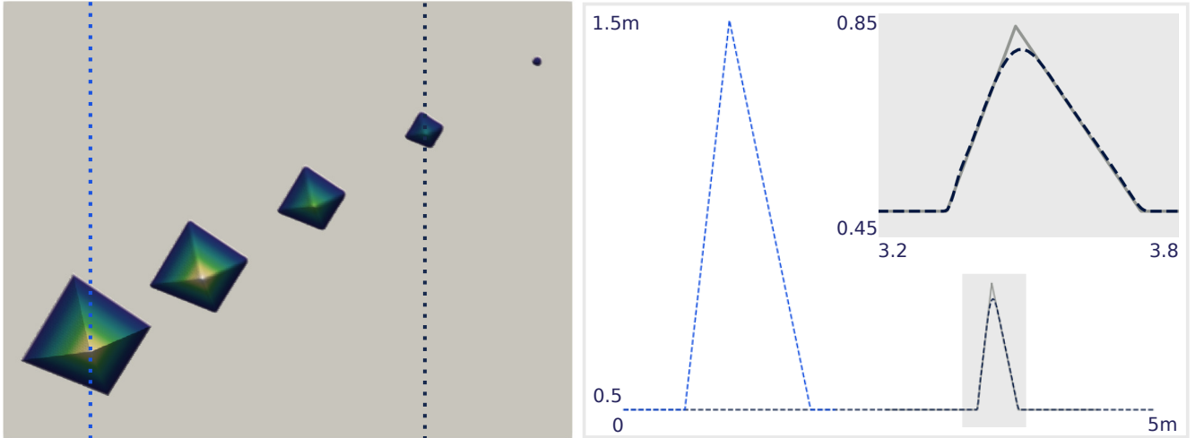
Figure 6. Test A-Pyramid Translation : Left panel shows top view of simulation results for N = 1000 at times t = 0, 1.5, 3.0, 4.5, 6.0 s. Dashed vertical lines indicate the location of the respective profiles in the right panel with the dashed light blue line displaying the profile at time 0 s. In the right panel, simulation results are shown by the dashed dark blue line and compared to the analytical solution (grey line) at time t = 4.5 s. The small panel on the right show a zoom of the grey rectangle on the main panel.
