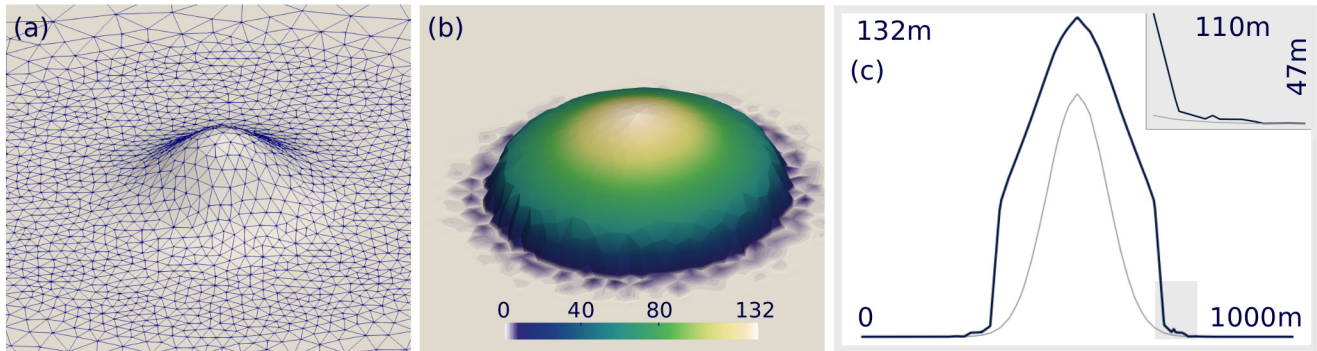
Figure 11. In (a) the ice-free geometry mesh formed by a gaussian-shaped hill in flat terrain and in (b) the simulated surface elevation after 20-24 years (standard continuous Galerkin stabilised with SUPG) is shown with a cross-profile of surface (blue) and bed (grey) elevation in (c).
