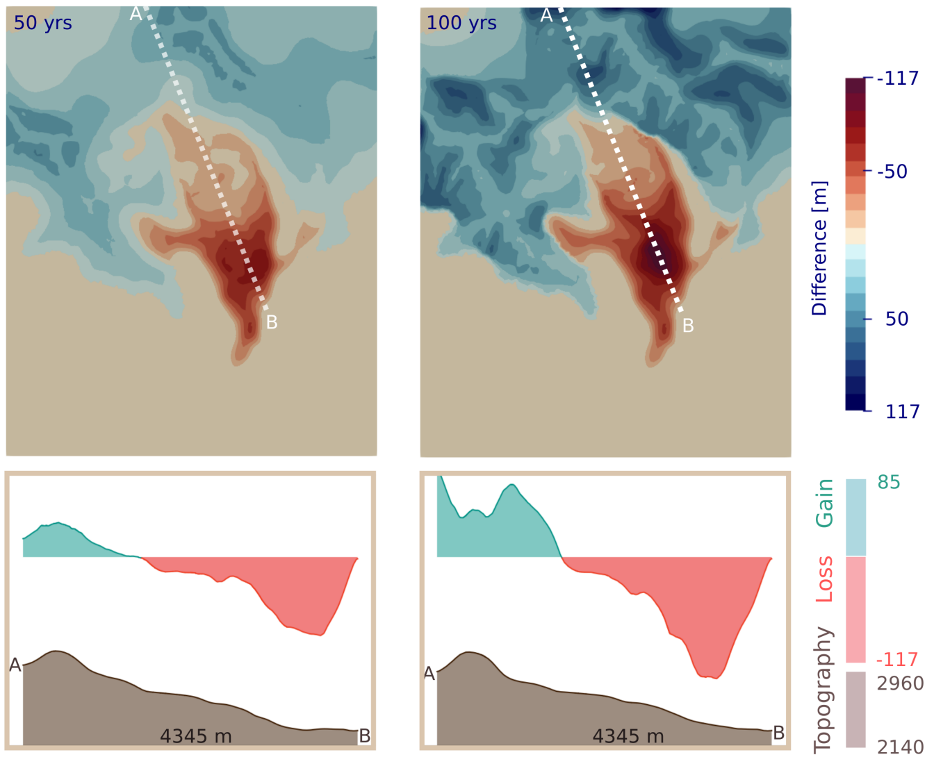
Figure 9. Test 2 ( measured mass balance rate ) Elevation-Dependent Mass Balance : top view of difference between initial surface elevation and simulation results at time steps 50 years and 100 years and corresponding profiles with shaded surface topography in brown in the lower panels.
