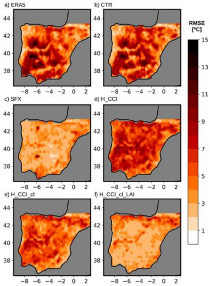
Figure 2. Same as Fig. 1 but for RMSE.
