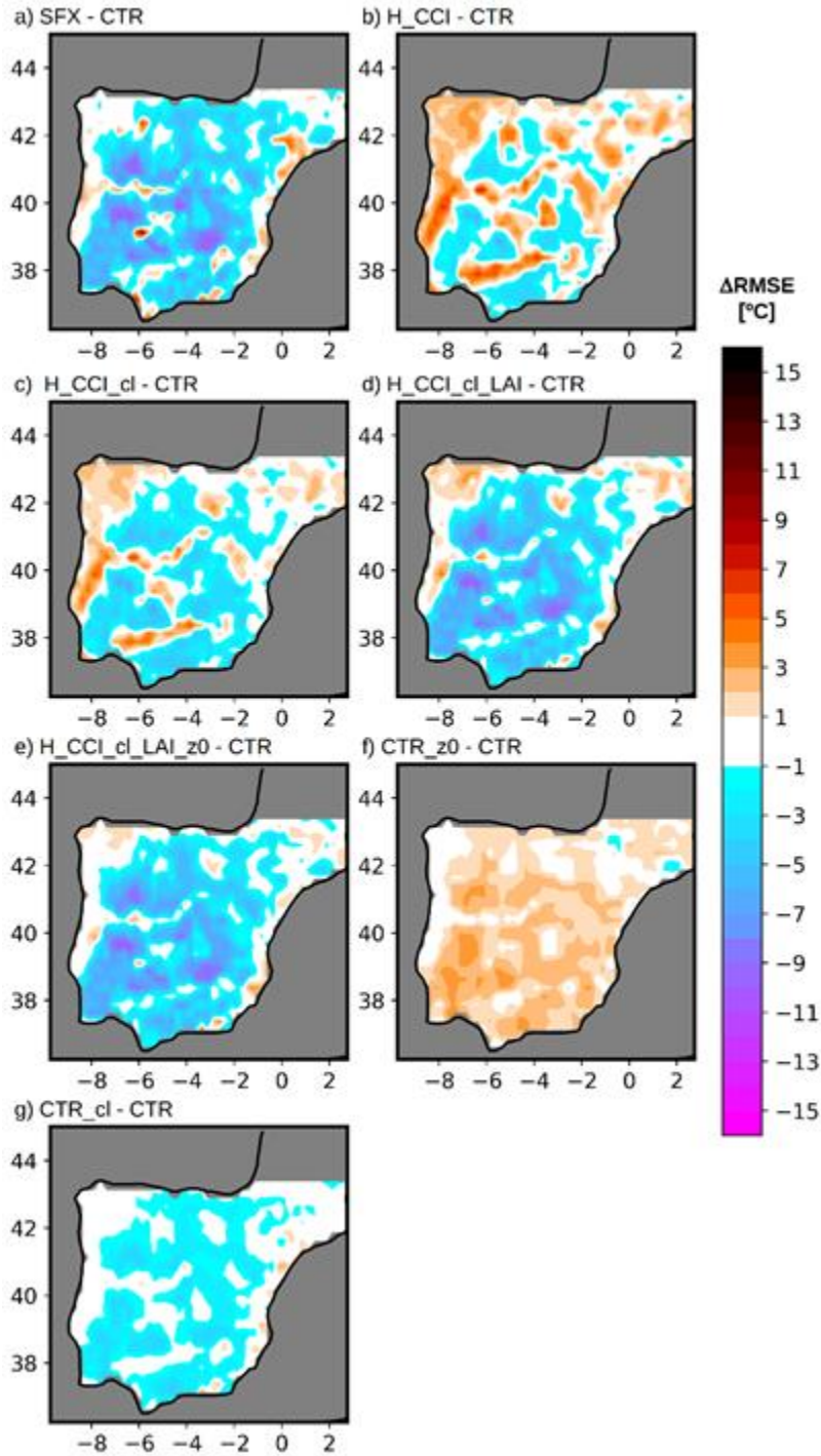
Figure 9. Difference in RMSE computed for daily maximum LST over Iberia in a) SFX minus CTR; b) H_CCI minus CTR; c) H_CCI_cl minus CTR; d) H_CCI_cl_LAI minus CTR; e) H_CCI_cl_LAI_z0 (same as H_CCI_cl_LAI but with z0h reduced by a factor of 10) minus CTR; f) CTR_z0 (same as CTR but with z0h reduced
