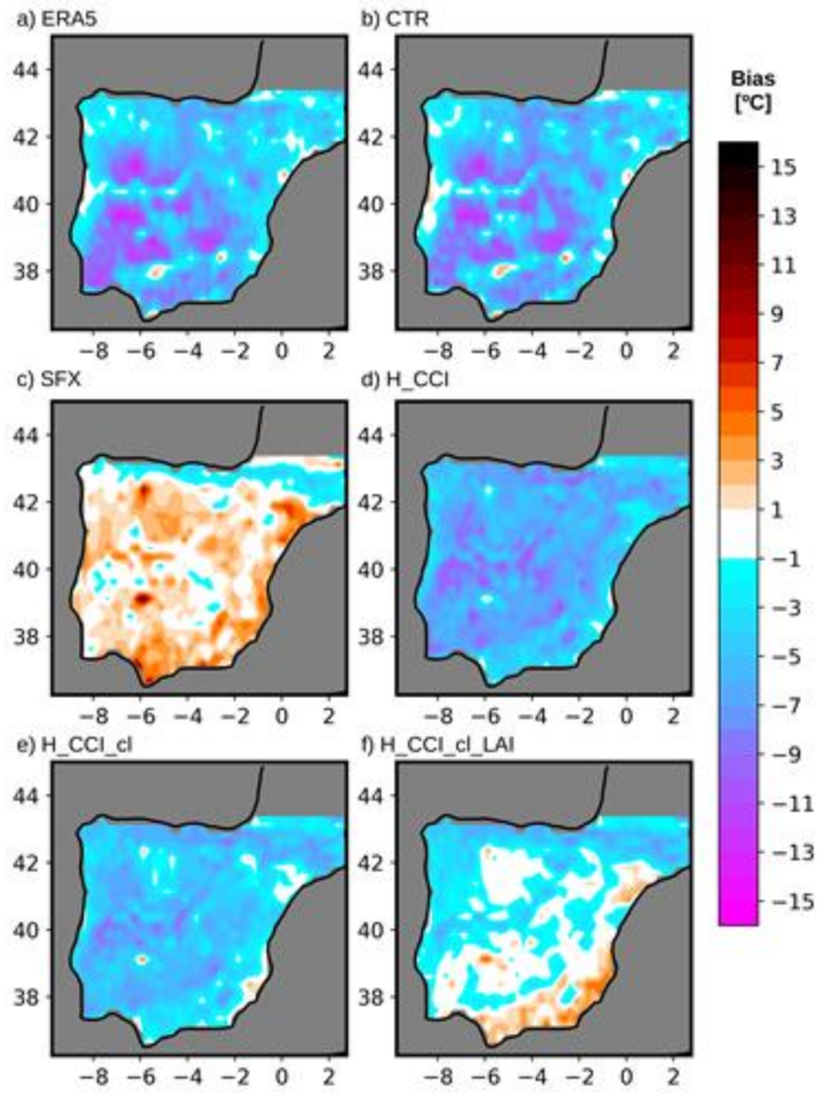
Figure 1. Maps of JJA daily maximum LST bias over Iberia under clear-sky conditions, computed for different simulations a) ERA5; b) CHTESSEL offline (CTR); c) SURFEX offline (SFX); d) H_CCI; e) H_CCI_cl; and f) H_CCI_cl_LAI. LSA-SAF LST was considered as reference for computing the simulation errors.
