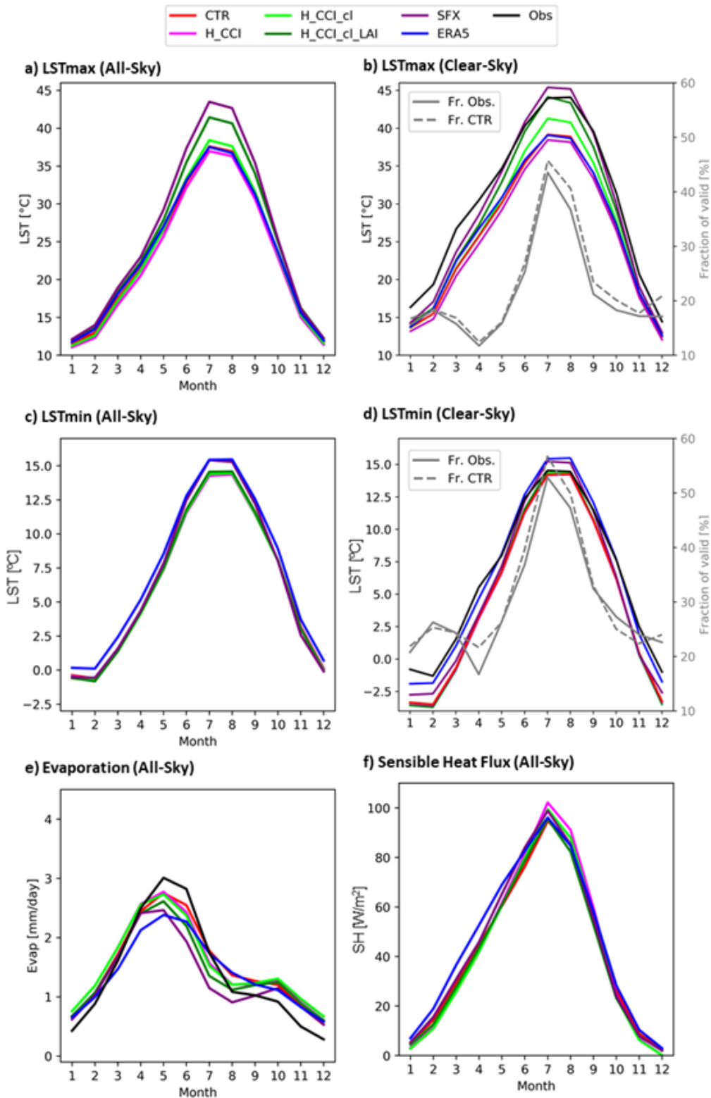
Figure 8. Seasonal cycles of daily maximum LST under all-sky (a), and clear-sky (b) conditions; daily minimum LST under all-sky (c) and clear-sky (d) conditions; daily total evaporation under all sky conditions (e), and daily mean sensible heat flux under all-sky conditions. All panels represent averages taken over all Iberia grid points considering all sky conditions, for each month during the 2004-2015 period. Observations are available for LST under clear-sky
