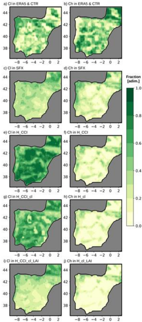
Figure 5. Fraction of low (CI, left column) and high (Ch, right column) vegetation coverage averaged over JJA. From top to bottom the panels represent CI and Ch in CTR (which is identical to ERA5), SFX, H_CCI, H_CCI_cl and H_CCI_cl_LAI.
