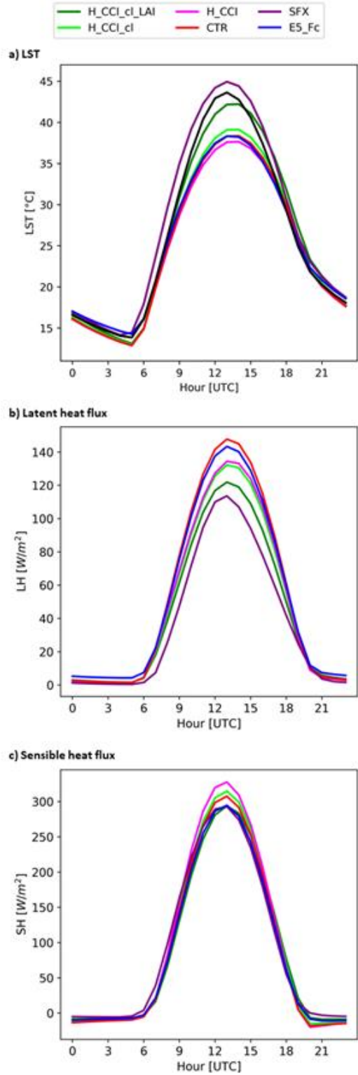
Figure 7. Diurnal cycles of JJA a) LST, b) latent heat flux and c) sensible heat flux averaged over all Iberia grid points, computed from LSA-SAF (black), ERA5 (blue), SFX (purple), CTR (red), H_CCI (pink), H_CCI_cl (light green), and H_CCI_cl_LAI (dark green). Only time instants under clear-sky conditions were considered.
