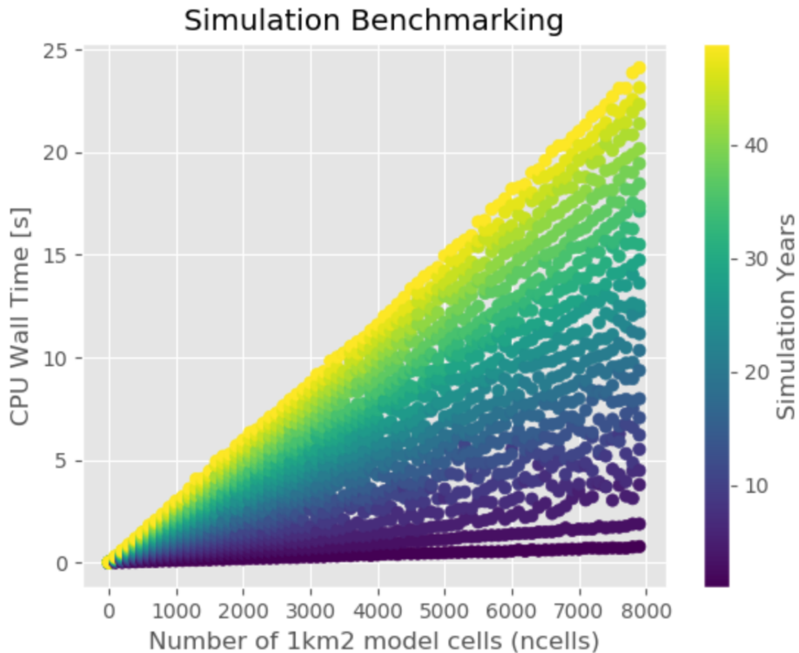
Figure 5. Benchmarking of Shyft computational performance conducted using a synthetic timeseries and regular 1km grid cells. The model was run at an hourly timestep for the purposes of testing with 3-hourly input data from the NOAA Global Ensemble Forecast System (GEFS).
