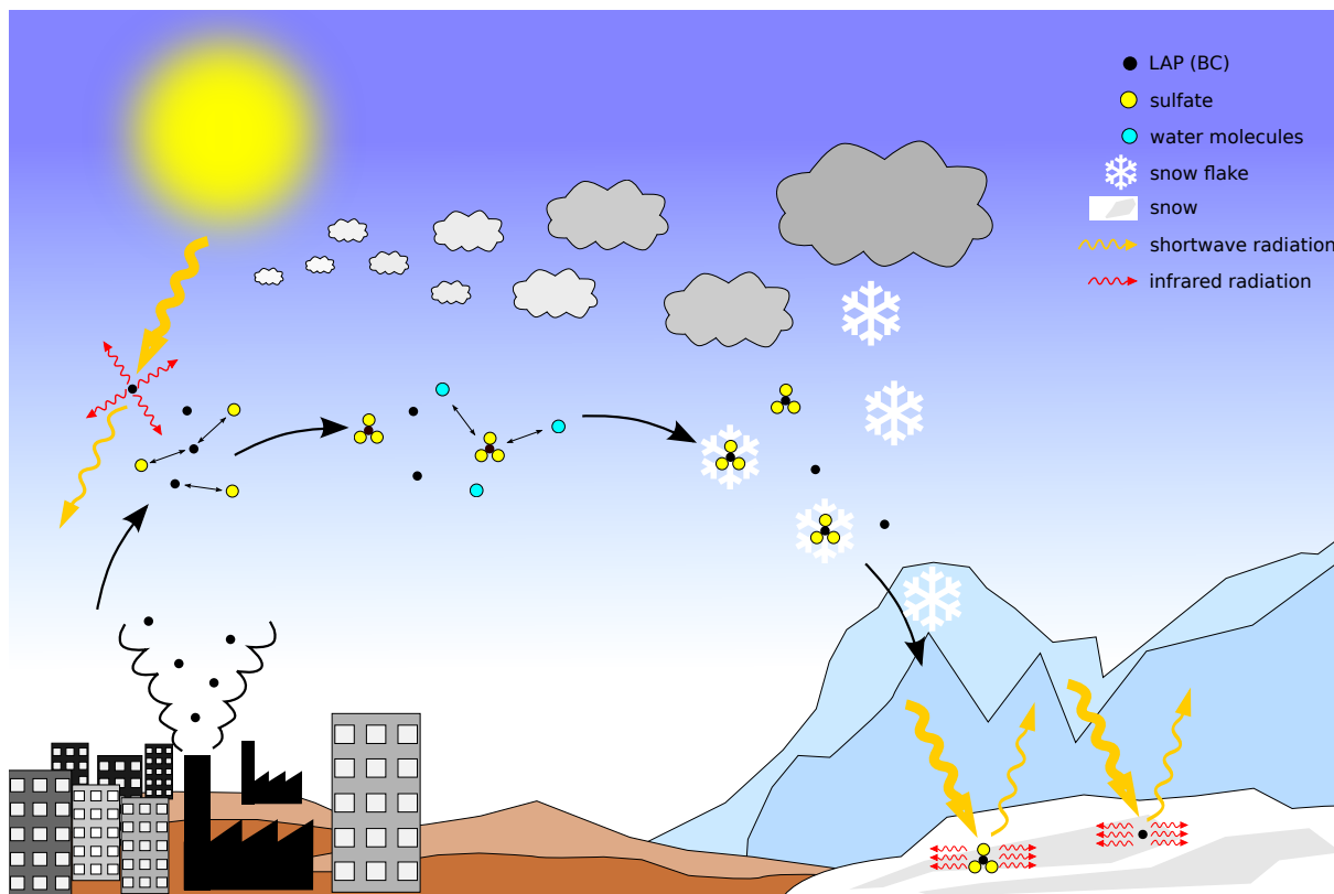
Figure 7. Schematic drawing of Black Carbon (and other light-absorbing particles) pathways and processes in atmosphere and snow.
