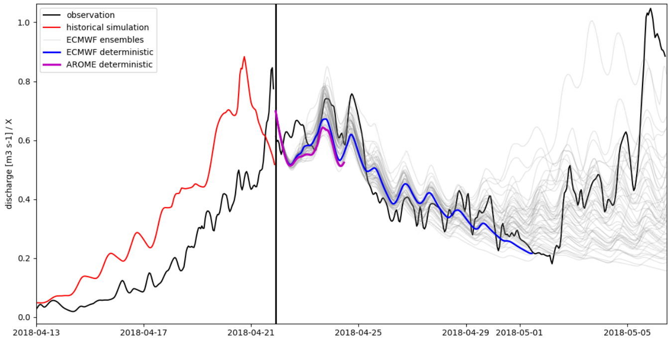
Figure 6. Example of a hydrological forecast conducted with Shyft for a subcatchment in the Nea-Nidelva basin. Shyft has been used to simulate the historical discharge (red) in order to estimate state variables at nowtime (22.04.2018, 00:00 UTC). Three different weather forecast products are then used in order to predict discharge: the operational deterministic weather prediction AROME with a forecasting horizon of 66 hours from the Norwegian Meteorological Institute (purple), ECMWF’s deterministic weather forecast with a horizon of 10 days (blue), and ECMWF’s ensemble weather prediction with a horizon of 15 days and 51 ensemble members (grey). Discharge observations (black) are shown for reference. Note: discharge are provided from Statkraft AS and are divided by a factor X in order to mask the observational data as Statkraft’s data policy considers discharge sensitive data.
