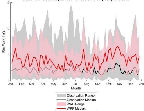
Case-NCAR Comparison of 10m Wind [m/s] at 08:00
