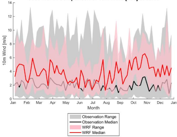
Case-NCAR Comparison of 10m Wind [m/s] at 02:00
