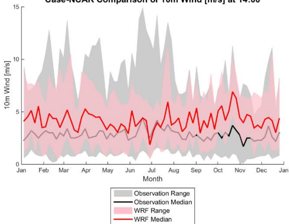
Case-NCAR Comparison of 10m Wind [m/s] at 14:00
