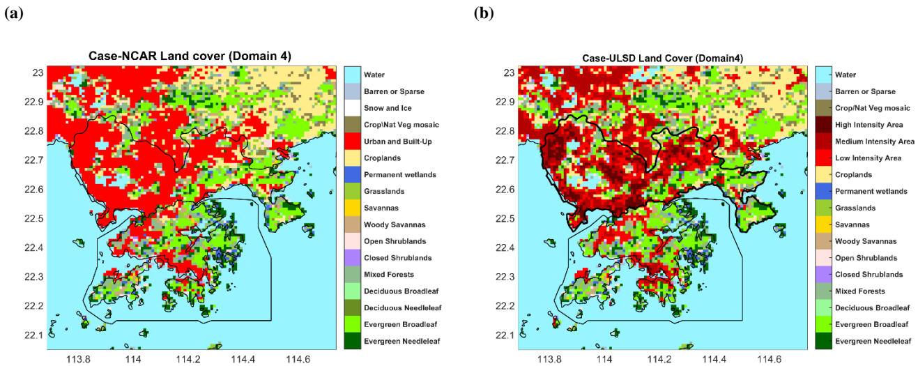
15 Figure 2: The land covers provided by NCAR originally (a), and the adjusted land covers based on the urban land surface dataset (b), data source: Li et al., 2019 a and b.
