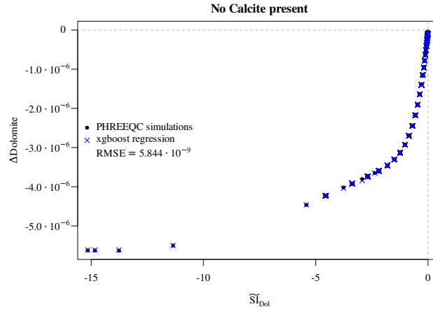
Figure 7. Regression of \Delta dolomite vs estimated \tilde{SI}_{Dol} for the cases where no calcite is initially present. The multivariate regressor makes use of the predictors \tilde{SI}_{Dol} , pH, C, Cl, Mg and dolomite.
