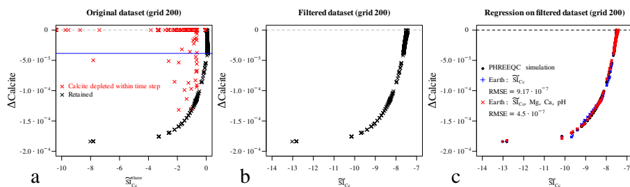
Figure 5. (a) Scatter plot of \Delta calcite vs estimated \widetilde{SI}_{Cc}^{theor} . The datapoints in red cannot be used to estimate the reaction rate from the dataset since calcite is depleted within the simulation time step. Furthermore, the retained points are not in bijective relationship with the \Delta calcite , with the blue horizontal line separating two regions where bijectivity is given. (b) \Delta calcite versus the simplified \widetilde{SI}_{Cc} : bijectivity is achieved. (c) A MARS regressor is computed for the retained data points, based solely on the estimated \widetilde{SI}_{Cc} (in blue) and using also other predictors to ameliorate the multivariate regression.
