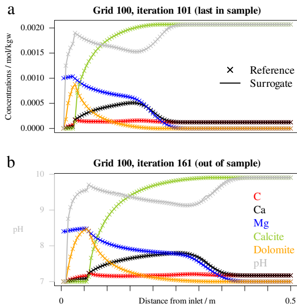
Figure 2. Profiles of total concentrations, pH and minerals for reference and hierarchical coupling 1D simulations with tolerance on mass balance error set to 10^{-6} , for grid 100. The top row displays axes are annotated in these figures: all aqueous and mineral concentrations are given in terms of mol per kg of solvent, while pH in its adimensional units. (a) here ist shown the last in sample time step; (b) the bottom the last simulated time step, after 60 iterations for which the surrogate was out of sample.
