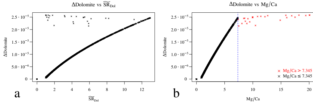
Figure 8. Precipitation of dolomite in presence of calcite. (a) the relationship between \Delta_{\text{dolomite}} and its saturation ratio is not surjective. (b) The Mg/Ca ratio perfectly discriminates two distinct regions in parameter space.
