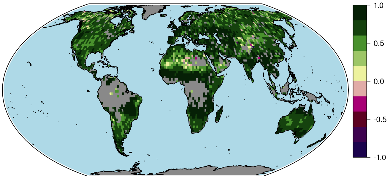
Figure 4. Correlation coefficient of the observed and predicted volumetric soil moisture time series in the individual grid cells during the test years 2014 and 2015. In the grey regions no observations are available during the this period.
