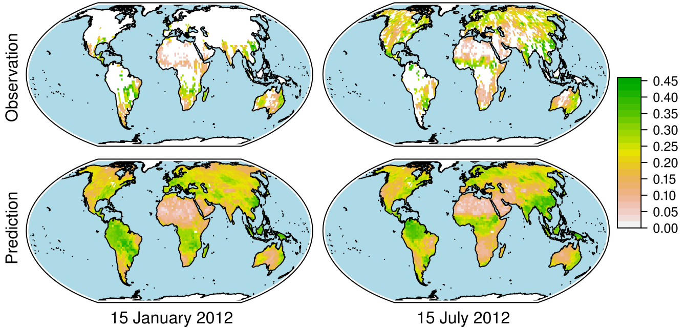
Figure 7. Global distribution of the observed and predicted volumetric soil moisture on a northern hemisphere winter (15. January 2012) and summer (15 July 2012) day in the training period.
