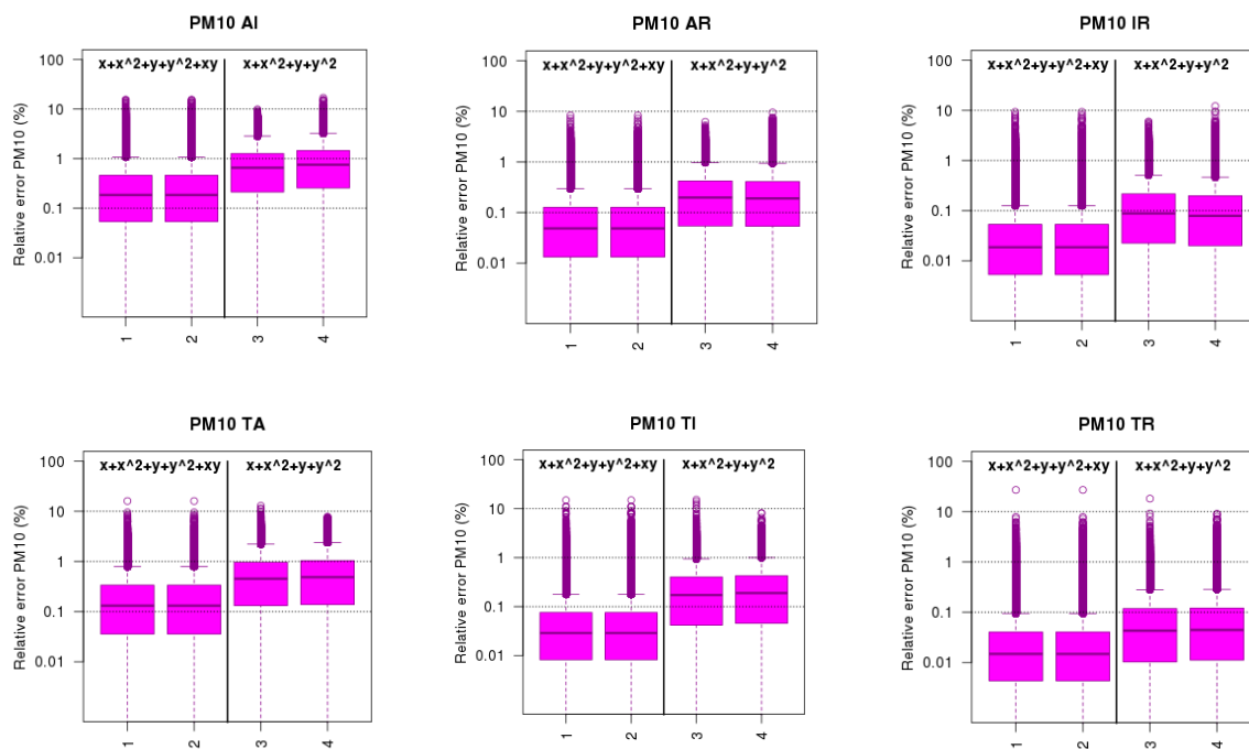
5 Figure 7: Relative error (%) of the PM 10 bivariate surrogate models (from left to right and top to bottom: AI: AGR&IND, AR: AGR&RH, IR: IND&RH, TA: TRA&AGR, TI: TRA&IND, TR: TRA&RH). For each panel, the boxplots of the distribution of errors are given for 2 models with interactions (left) and 2 models without interactions (right), where indices in the x-axis match the row of Table 2. The distributions of relative errors include each grid points in Western Europe and each day over three air pollution events (201503, 201612, 201701). The dotted horizontal lines are for 0.1%, 1%, and 10% errors.
