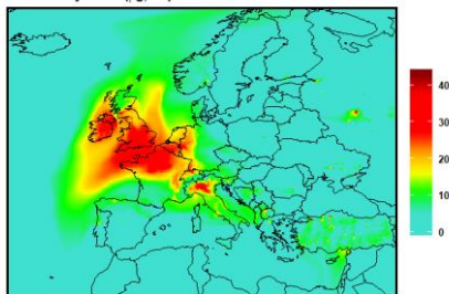
PM10 map including only the main anthropogenic sources: (agriculture, industry, traffic and residential heating; (mainly natural dust and sea salt for particulate matter) but also a few anthropogenic sectors such as shipping.
