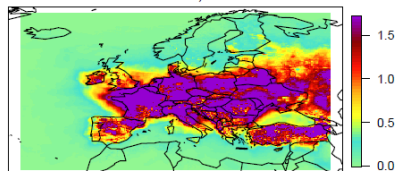
201612 PM10 AGR Err 1.63 x+x^2 / \text{AGR}90, \text{AGR}100
