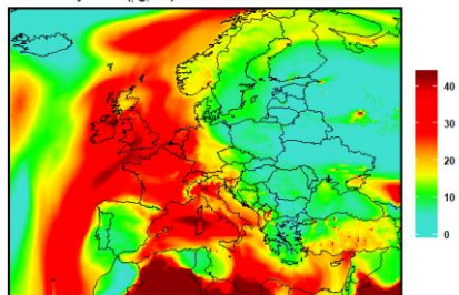
Reference PM10 map including all sources (natural and anthropogenic) and background concentrations.
