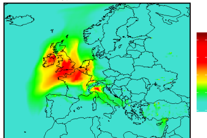
Map of PM10 for a Europe-wide uniform reduction of: Agriculture: 0 %; Traffic: 0 %; Residential: 100 %; Industry: 0 %
