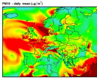
Figure 12: First row: PM 10 concentrations on 20150318 including (left) or excluding (right) natural and background concentrations. Following rows: PM 10 daily average concentrations emulated with ACT for 20150318 for a 100% reduction of traffic emissions (2 nd row, left), residential emissions (2 nd row, right), industry emissions (3 rd row, left), agriculture emissions (3 rd row, right), and both traffic and industry (4 th row, right).
