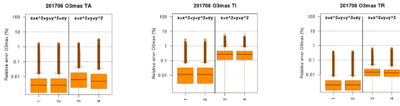
Figure 8: Same as Figure 7 for O 3max and 201706.
