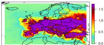
201612 PM10 AGR Err 0.654 x+x^2 / \text{AGR}30, \text{AGR}100
