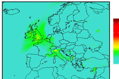
Map of PM10 for a Europe-wide uniform reduction of: Agriculture: 100 %; Traffic: 0 %; Residential: 0 %; Industry: 0 %
