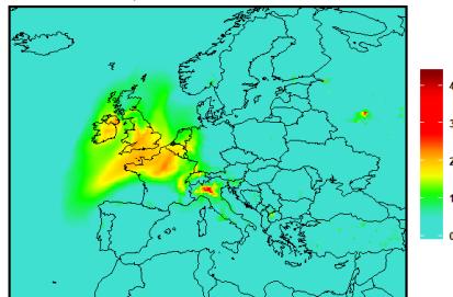
Map of PM10 for a Europe-wide uniform reduction of: Agriculture: 0 %; Traffic: 0 %; Residential: 0 %; Industry: 100 %
