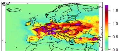
201612 PM10 AGR Err 1.9 x+x^2 / \text{AGR}30, \text{AGR}60
