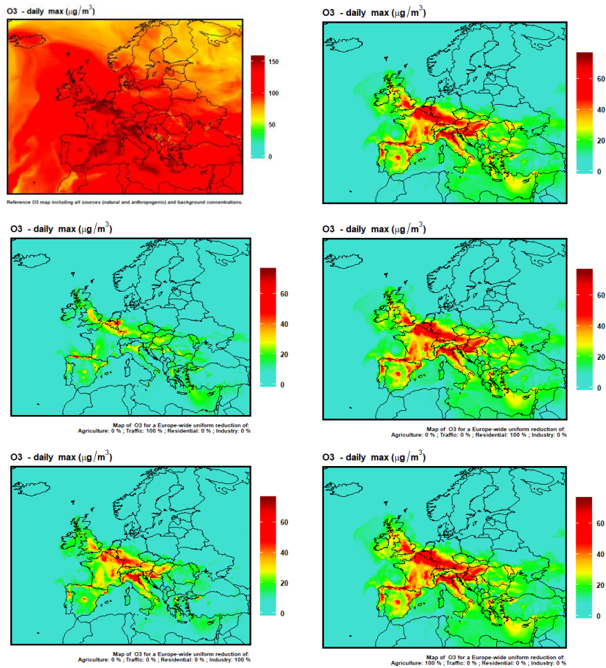
Figure 14: First row: O 3 max concentrations on 20170621 including (left) or excluding (right) natural and background concentrations. Following rows: O 3 max concentrations emulated with ACT for 20170621 for a 100% reduction of traffic
