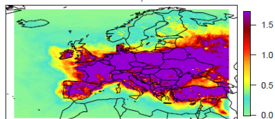
201612 PM10 AGR Err 0.869 x+x^2 / \text{AGR}10, \text{AGR}100
