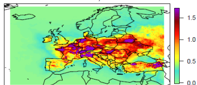
201612 PM10 AGR Err 0.674 x+x^2 / \text{AGR}30, \text{AGR}90
