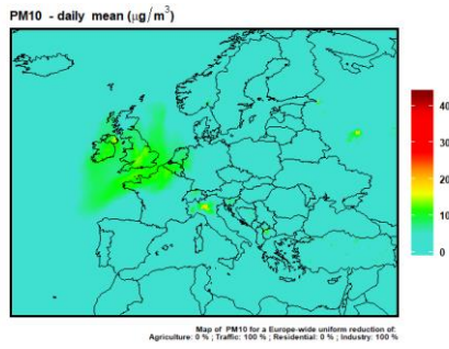
Figure 12: First row: PM 10 concentrations on 20150318 including (left) or excluding (right) natural and background concentrations. Following rows: PM 10 daily average concentrations emulated with ACT for 20150318 for a 100% reduction of traffic emissions (2 nd row, left), residential emissions (2 nd row, right), industry emissions (3 rd row, left), agriculture emissions (3 rd row, right), and both traffic and industry (4 th row, right).
