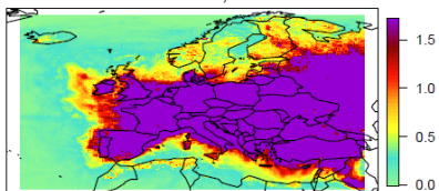
201612 PM10 AGR Err 0.847 x+x^2 / \text{AGR}10, \text{AGR}90
