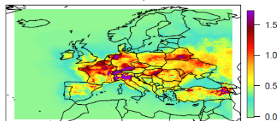
201612 PM10 AGR Err 0.717 x+x^2 / \text{AGR}60, \text{AGR}90
