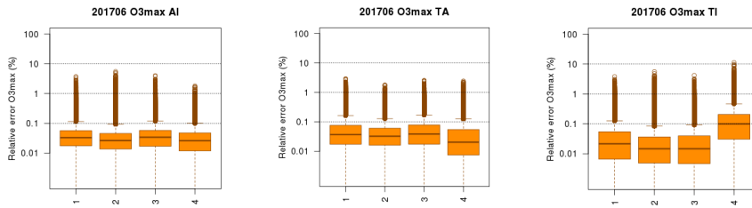
Figure 10: Same as Figure 9 for O 3 max and 201706.
