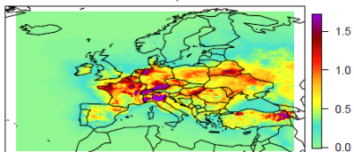
201612 PM10 AGR Err 0.646 x+x^2 / \text{AGR}60, \text{AGR}100
