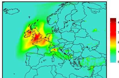
Map of PM10 for a Europe-wide uniform reduction of: Agriculture: 0 %; Traffic: 100 %; Residential: 0 %; Industry: 0 %
