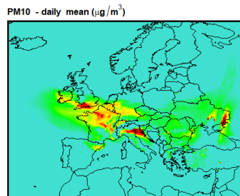
Map of PM10 for a Europe-wide uniform reduction of: Agriculture: 0 % ; Traffic: 0 % ; Residential: 100 % ; Industry: 0 %
