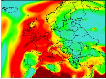
Reference PM10 map including all sources (natural and anthropogenic) and background concentrations.
