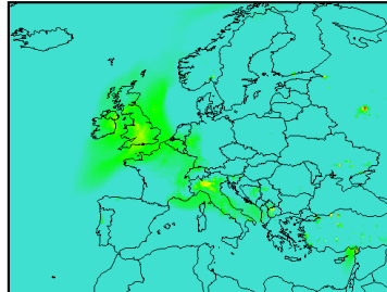
Map of PM10 for a Europe-wide uniform reduction of: Agriculture: 100 %; Traffic: 0 %; Residential: 0 %; Industry: 0 %
