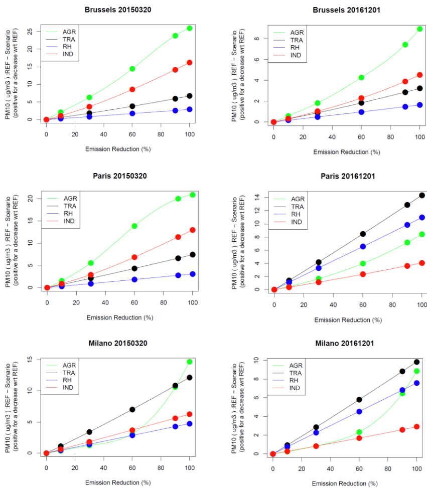
Figure 1 : Modelled PM 10 reduction (y-axis : positive for a decrease with respect to the reference, µg/m 3 ) for a given reduction in Agriculture (green), Industrial (red), Residential Heating (blue), and Traffic (black) emissions (x-axis: in %) in Brussels, Paris and Milano (top to bottom) and for 20150320 (left) and 20161201 (right).
