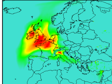
Map of PM10 for a Europe-wide uniform reduction of: Agriculture: 0 %; Traffic: 0 %; Residential: 100 %; Industry: 0 %
