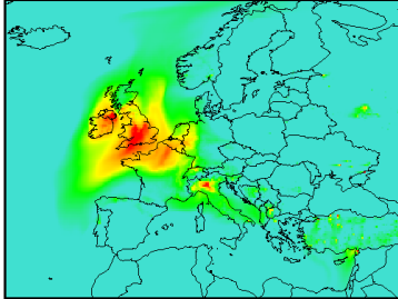
Map of PM10 for a Europe-wide uniform reduction of: Agriculture: 0 %; Traffic: 100 %; Residential: 0 %; Industry: 0 %
