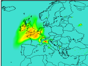
Map of PM10 for a Europe-wide uniform reduction of: Agriculture: 0 %; Traffic: 0 %; Residential: 0 %; Industry: 100 %
