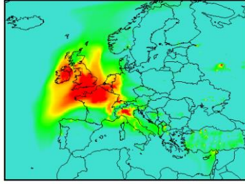
PM10 map including only the main anthropogenic sources: (agriculture, industry, traffic and residential heating; mainly natural dust and sea salt for particulate matter) but also a few anthropogenic sectors such as shipping.
