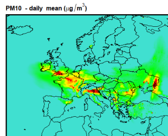
Map of PM10 for a Europe-wide uniform reduction of: Agriculture: 0 % ; Traffic: 100 % ; Residential: 0 % ; Industry: 0 %
