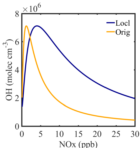
Fig. 1 the localized (blue line) and original (yellow line) parameterization of the NO x –OH concentration curve in the P6 scheme. The input parameters used to calculate the curve were annually averaged.
