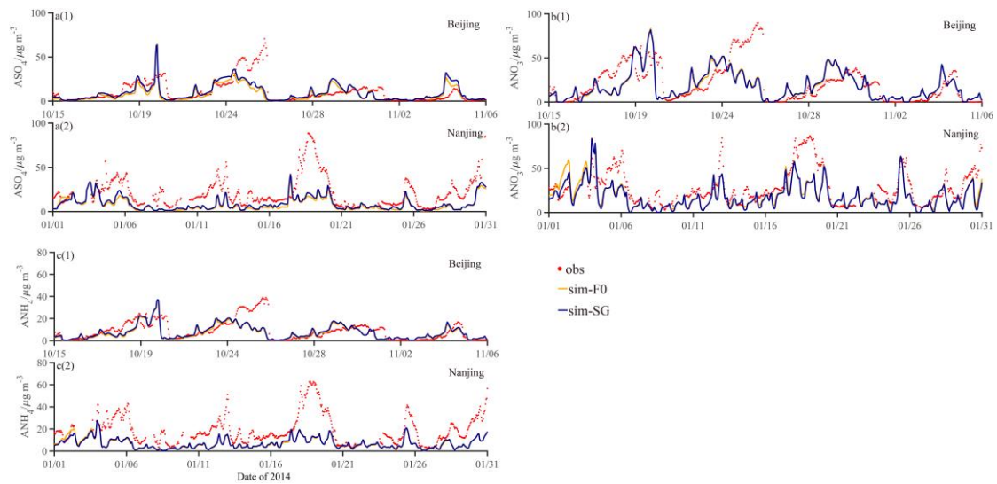
Fig. 7 The same as Fig. 5, but for Beijing and Nanjing in cold seasons.
