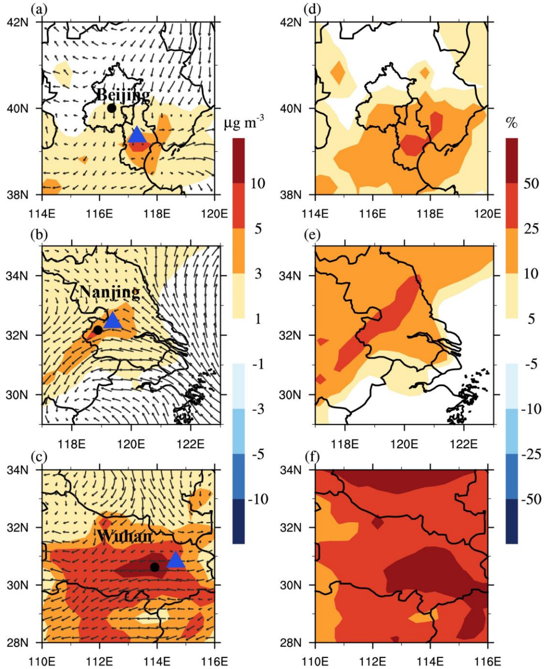
Fig. 10 Daily averaged differences with overlaid overlaid wind field (left column, \mu\text{g m}^{-3} ) and relative change (right column, %) of sulfate concentrations on regional scale between SG and F0 at surface, around: (a, d) Beijing in June 22, (b, e) Nanjing in May 16 and (c, f) Wuhan in October 15. The difference was calculated as the simulation of SG minus F0. Black dots and blue triangles represent locations of the ground sites and plants, respectively.
