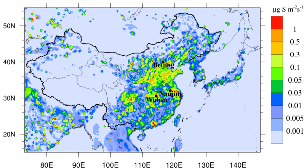
Fig. 2 The nested domain with annual mean SO 2 emission flux (unit : \mu\text{g S m}^{-2}\text{s}^{-1} ) 375 from energy and industry sectors in 2014. The black circles are locations of the observation sites.
