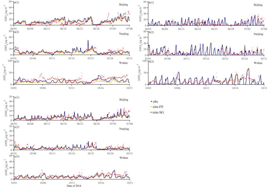
Fig. 5 Comparison of hourly simulated aerosol components against site observations in Beijing, Nanjing and Wuhan in warm seasons: (a1–a3) sulfate, (b1–b3) nitrate, (c1–c3) ammonium. The blue and orange line represent simulations with SG scheme and with constant f_{ox} of 0% (F0), respectively. The red dots represent observations.
