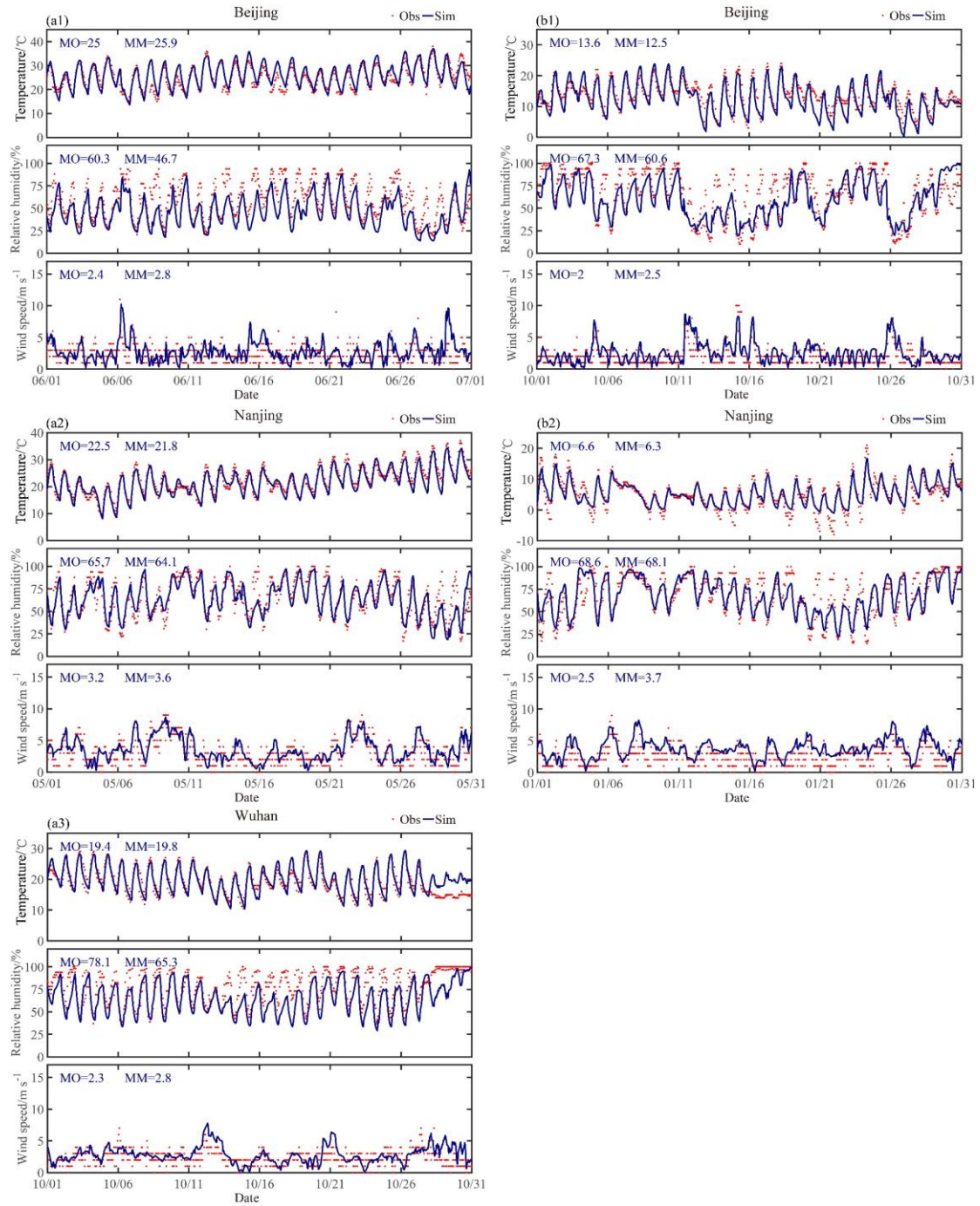
Fig. 3 Comparison between observed and simulated meteorological factors (i.e., temperature, relative humidity and wind speed) in: (a1) Beijing; (a2) Nanjing; (a3) Wuhan in warm seasons and (b1) Beijing; (b2) Nanjing in cold seasons of 2014. The red dots and blue lines represent hourly observations and simulations, respectively. Monthly mean values of the observation and simulation are also given on subplots in blue texts, abbreviated to MO and MM, respectively.
