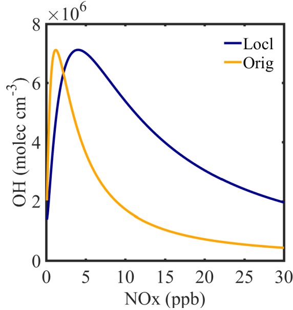
Fig. 1 the localized (blue line) and original (yellow line) parameterization of the \text{NO}_x -OH concentration curve in the P6 scheme. The input parameters used to calculate the curve were annually averaged.
