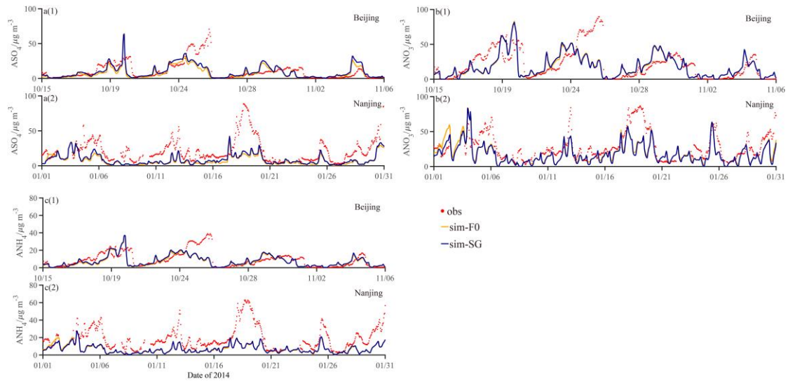
Fig. 7 The same as Fig. 5, but for Beijing and Nanjing in cold seasons.
