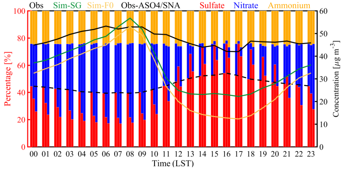
Fig. 6 Averaged diurnal variation for the observed and simulated total SNA concentrations (solid lines), observed ASO4/SNA ratio (black dot line) and the percentage of sulfate, nitrate and ammonium in total SNA concentrations (color bars, i.e., observations, simulations of SG and F0) in Wuhan, October 1-21, 2014.
