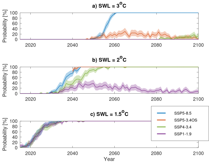
Figure 6: Probability for exceeding a given Surface Warming Level (SWL) in the different scenarios. The SSP5-3.4QS experiment branches off from SSP5-8.5 in 2040 according to the CMIP6 experimental protocol and thus there are no data for this scenario before 2040. The shaded area denotes the 95% confidence interval obtained from bootstrapping with 1000 repetitions.
