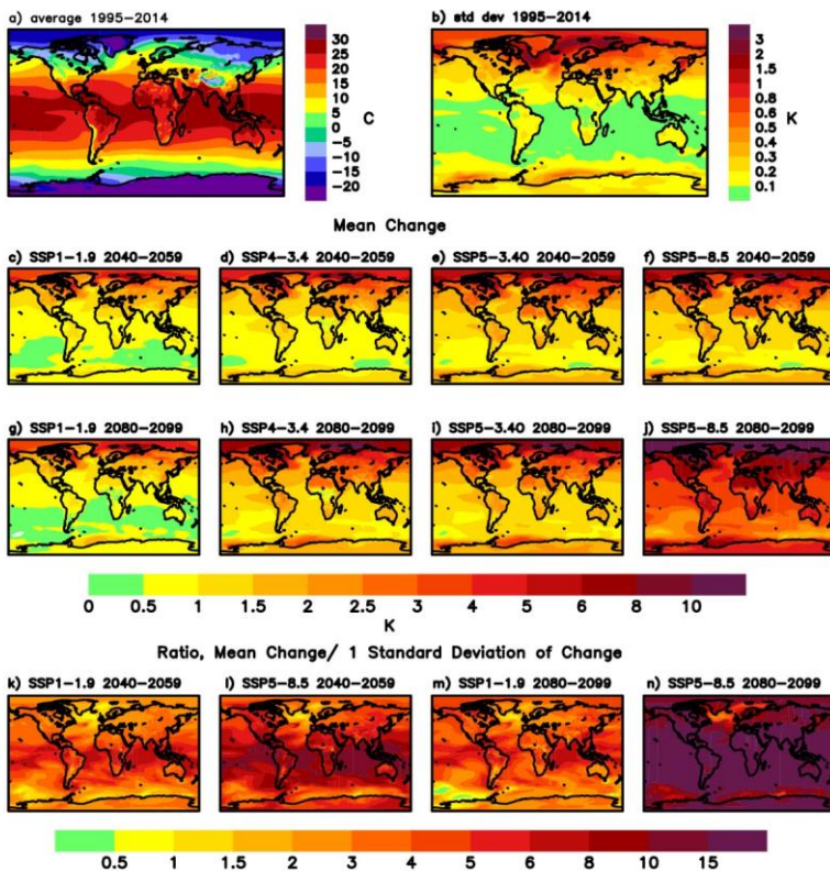
620 Figure 3: a) Ensemble mean annual mean 2m air temperature, averaged over 1995-2014. b) One standard deviation of annual mean 2 m air temperature, averaged over 1995-2014, across ensemble members. c) - f) Ensemble mean 2m air temperature change between 2040-2059 and 1995-2014 for SSP1-1.9, SSP4-3.4, SSP5-3.4-OS and SSP5-8.5. All coloured areas show significant changes at the 95% significance level based on a two-sided student t-test. g)- j) Same as c) - f) but for changes until 2080-2099.
