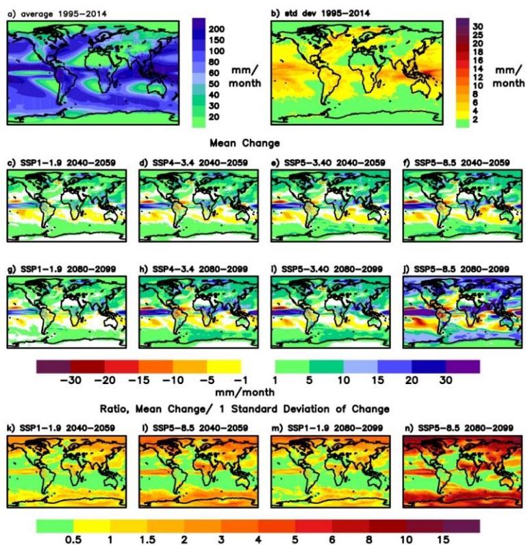
Figure 4: Same as Figure 3 but for annual mean precipitation. Precipitation changes that are not marked coloured are either not significant at the 95% significance level or small (below \pm 1 mm/month).
