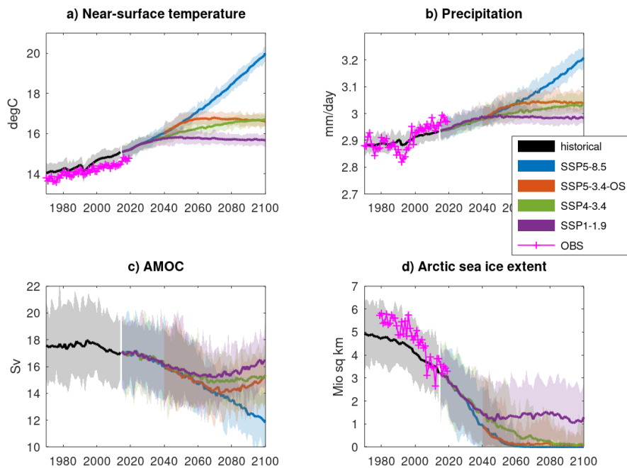
Figure 2: Timeseries of global annual mean near surface temperature ( TAS ), precipitation, AMOC and minimum Arctic sea ice extent in the historical and scenario experiments. Thick lines denote the ensemble means and shaded area the full ensemble width. The scenarios branch off from the historical experiment in 2015 except for SSP5-3.4-OS that branches off from SSP5-8.5 in 2040. The magenta lines marked with plus signs denote the ERA5 re-analysis (Hersbach et al. 2020) for temperature and precipitation, and the OSI-450 sea-ice observations (Lavergne et al. 2019).
