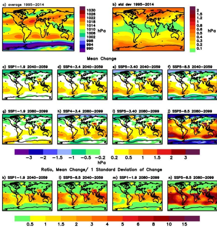
Figure 5: As Figure 3 but for sea level pressure. Sea level pressure changes that are not marked coloured are either not significant at the 95% significance level or small (below \pm 0.2 hPa).
