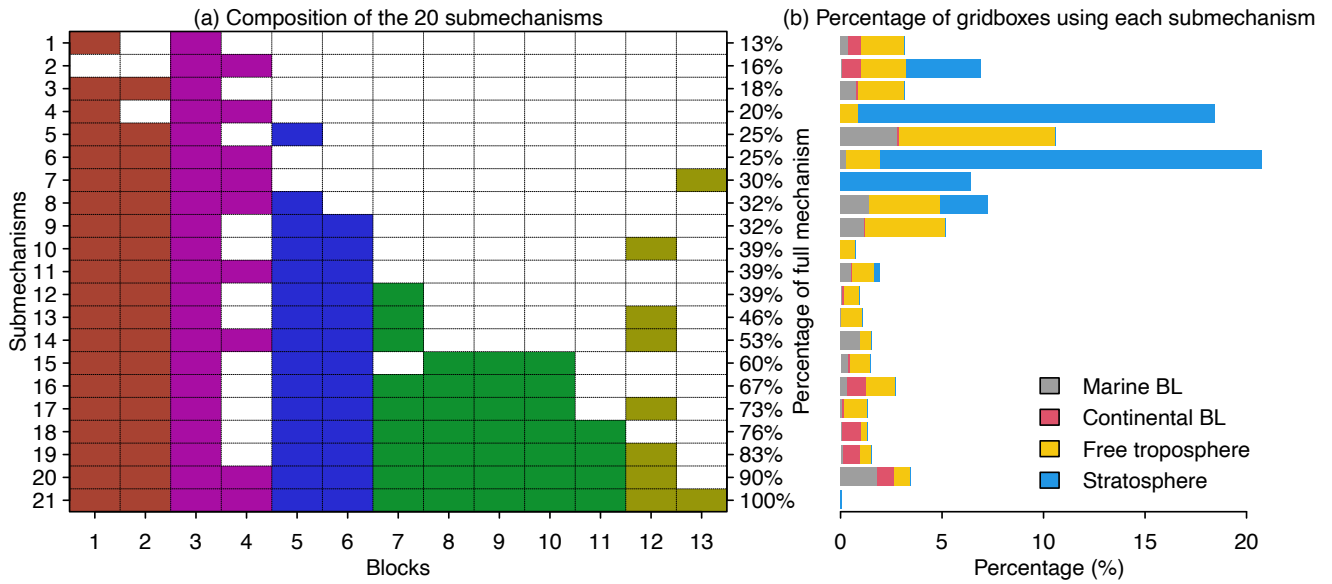
Figure 5. Submechanisms and percentage of gridboxes using each mechanism. Panel (a) shows the composition of the 20 submechanisms and full mechanism (the 21 st one) as well as the percentage of species from the full mechanism that are treated as fast in each of them. Colors denote species block types as defined in Figure 4. Panel (b) shows the percentage of gridboxes using each submechanism in the marine boundary layer (BL, 0-2 km altitude), continental BL, free troposphere (2km to tropopause), and stratosphere.
