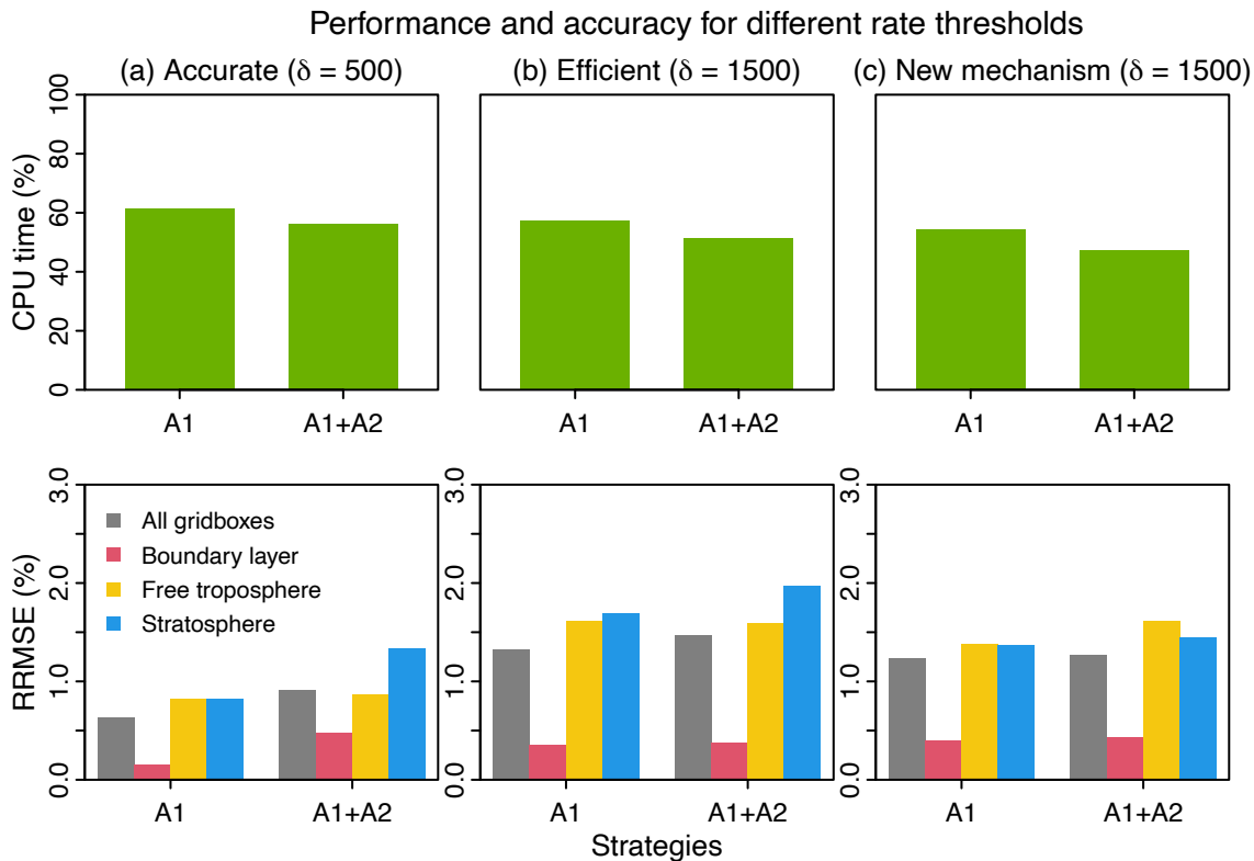
Figure 6. Performance and accuracy of the adaptive chemical mechanism. We test the performance of the adaptive method by (A1) removing slow species ( P_i or L_i > \delta ) and (A2) removing slow reactions (reaction rate < 10 molecules \text{cm}^{-3} \text{s}^{-1} ). Results are shown on the last day of 3-year simulations. The unit of \delta is molecules \text{cm}^{-3} \text{s}^{-1} . The performance is measured by the computing processor unit (CPU) time used by the chemical operator, and the accuracy is measured by the median relative root mean square error (RRMSE) for species concentrations using the full chemical mechanism for all gridboxes, in the boundary layer (0-2 km altitude), free troposphere (2 km to tropopause), and stratosphere. For (a) and (b), we use \delta as 500 and 1500 molecules \text{cm}^{-3} \text{s}^{-1} in GEOS-Chem 12.0.0 that has 228 species and 724 reactions. For (c), we port the algorithm to GEOS-Chem 12.9.1 that has 262 species and 850 reactions. The number of blocks ( N ) is 13 and the number of chemical regimes is 21 (20 submechanisms ( M=20 ) and one full mechanism).
