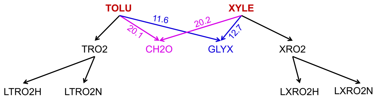
395 Figure 1. Definition of species distances for TOLU (toluene) and XYLE (xylene) using the analysis of family trees in graph theory. The number denotes the distance between species as calculated by Eq. 3. The shortest path from TOLU to XYLE is TOLU-GLYX-XYLE in this graph, where GLYX is glyoxal.
