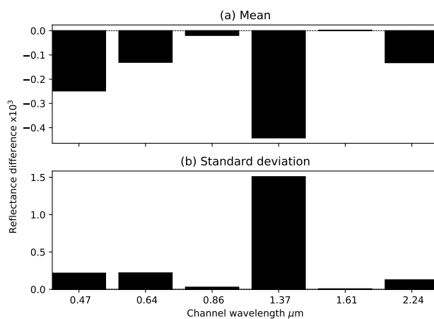
Figure 5. Difference in RTTOV reflectances calculated with v9 and v13 predictors with variable \text{O}_3 and \text{CO}_2 for GOES-16 ABI visible/near-IR channels for 52 independent profiles. Note that the vertical scale is magnified by a factor of 1000.
