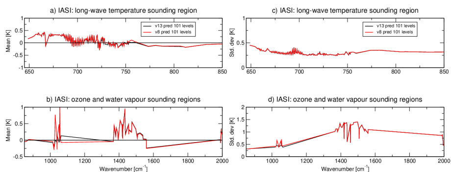
Figure 15. As Fig. 14, but with RTTOV v13 coefficients that are based on the new v13 predictors and the v8 predictors (variable O 3 and CO 2 on 101 levels).
