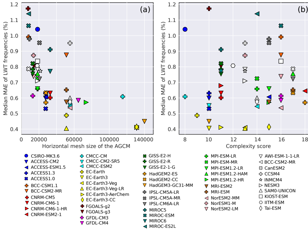
Figure 13. Relationship between the median performance of the coupled model configuration and (a) the horizontal mesh size of the atmospheric component or (b) the coupled model complexity score described in Section 3.3. Model performance is w.r.t. ERA-Interim. CNRM-CM6-1-HR and CNRM-ESM2-1 are out of scale in panel (a) due to their very fine atmospheric resolution.
