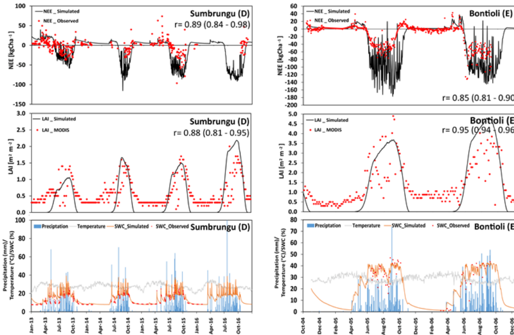
Figure 5 (D-E): Time series of the observed and modelled NEE ( \text{kg ha}^{-1} , negative values represent a flux to the biosphere, positive values a flux to atmosphere), LAI ( \text{m}^2 \text{m}^{-2} ), and soil water content (in 10 cm depth) . In addition, precipitation, and temperature at different grass-dominated sites in Sudanian zone are presented.
