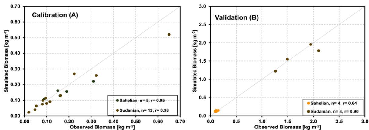
Figure 8: Correlations between the observed and modelled biomass production at different tree-dominated grassland/woodland sites in Sahelian and Sudanian ecological zone through calibration and validation process.
