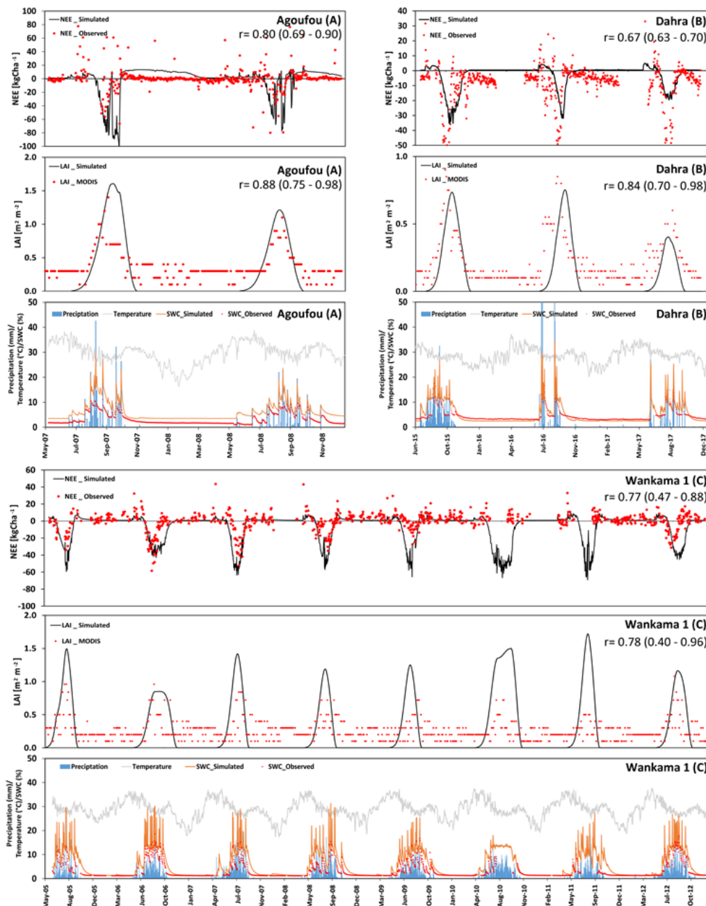
Figure 5 (A-C): Time series of the observed and modelled NEE (kg ha -1 , negative values represent a flux to the biosphere, positive values a flux to atmosphere), LAI (m 2 m -2 ), and soil water content (in 10 cm depth). In addition , precipitation and temperature at different grass-dominated sites in Sahelian zone are presented.
