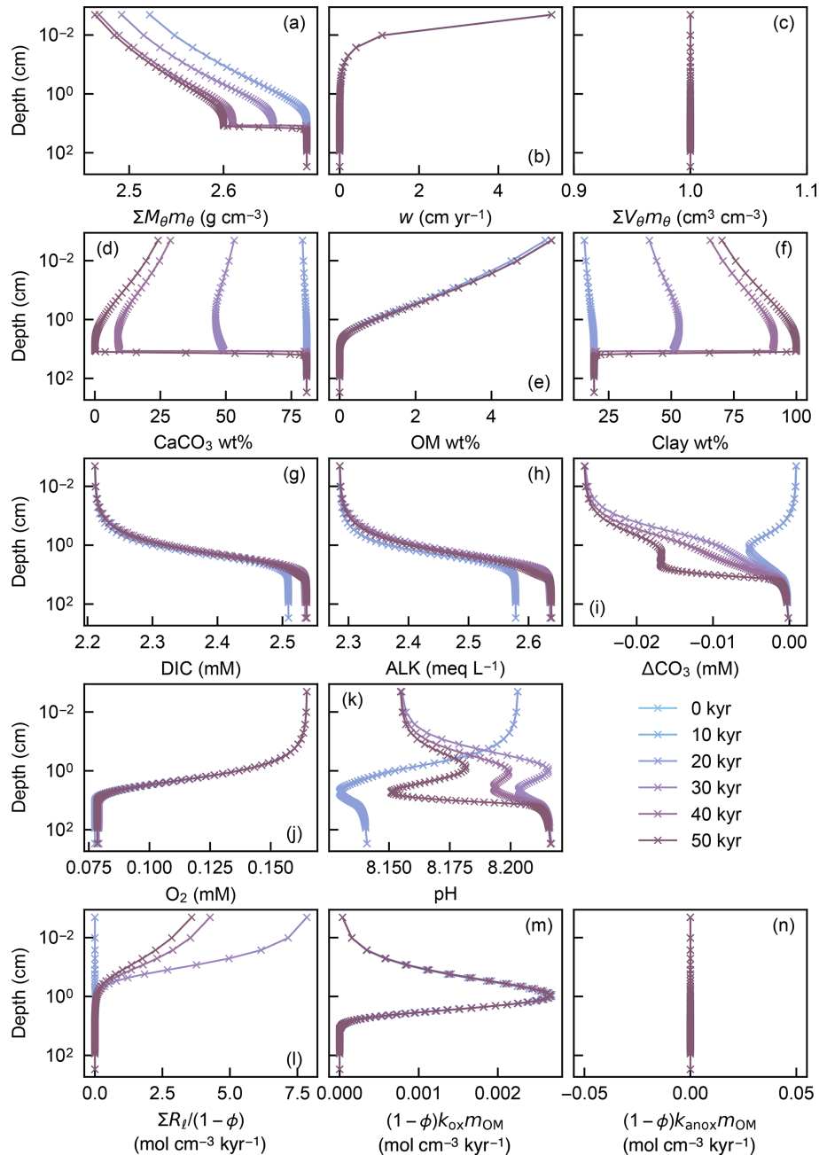
Figure 7. Depth profiles of the density (a) and volume fraction (c) of solid sediment, burial velocity (b), weight fractions of bulk CaCO 3 (d), organic matter (e) and nonreactive detrital materials (f) in solid sediment, porewater concentrations of total dissolved CO 2 species (g), carbonate alkalinity (h) and oxygen (j), deviation of porewater carbonate concentration from that in equilibrium with CaCO 3 (i), porewater pH (k), dissolution rate of CaCO 3 (l), and decomposition rate of organic matter in the oxic (m) and anoxic (n) zone of sediment, as a function of time. The boundary conditions of the model change with time as in dissolution experiment 2 (Sect. 3.2.2, Fig. 12). The calculations assume four classes of CaCO 3 particles and Fickian mixing for bioturbation. Illustrated are the temporal evolutions of the depth profiles which are initially at steady state at 3.5 km of water depth but perturbed by water depth change to 5.0 km between 5 and 45 kyr.
