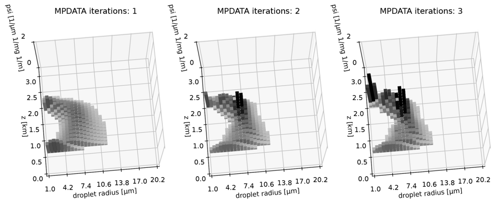
Figure 10. Snapshots of the advected two-dimensional liquid water field at t = t_1 = 600 s for simulations with different number of MPDATA iterations (see text for details). TSS
