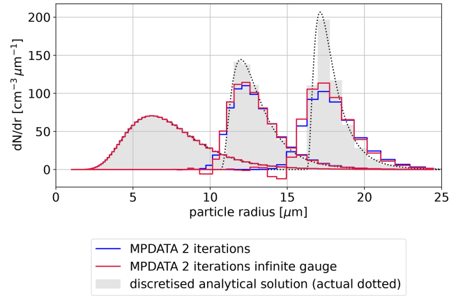
Figure 4. Comparison of analytical, upwind and MPDATA solutions (see plot key for algorithm variant specification) using the set-up from Fig. 1; see Sect. 2.5 for discussion.
