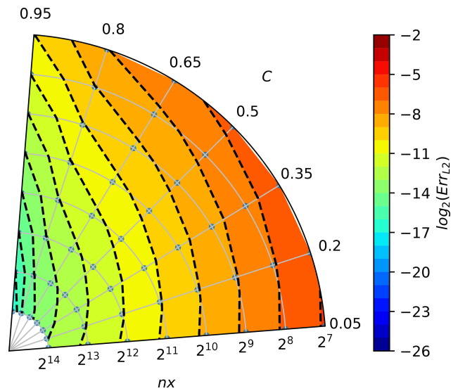
Figure A1. Convergence plot for the upwind scheme (cf. Fig. 1). Angle in the polar plot corresponds to the Courant number C , and the distance from origin denotes the number of grid boxes nx ; see Eq. (A2). Grey dots indicate data point locations – parameter values for which computations were made. Colours and isolines depict the error measure values (interpolated from the data point locations), see Eq. (A1).
