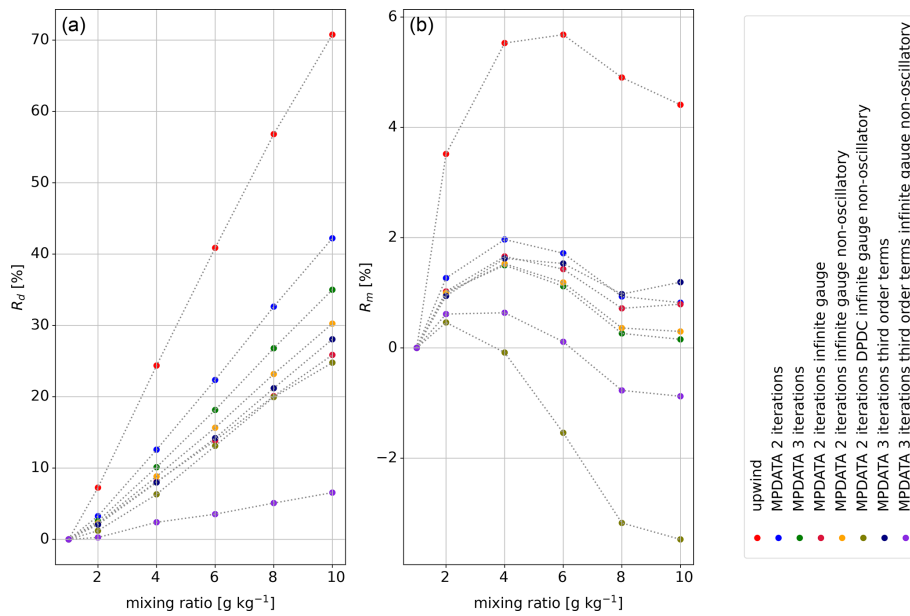
Figure 9. Panel (a) summarises values of the numerical-to-analytical spectral width ratio R_d = d_{\text{numerical}}/d_{\text{analytical}} - 1 (expressed as a percentage) computed for simulations using different discussed variants of MPDATA and plotted as a function of increasing mixing ratio (i.e. each simulation is depicted with a set of line-connected points corresponding to selected time steps); see Sect. 2.11. Panel (b) presents analogous analysis for R_m ; see Sect. 2.12 for discussion. Note: R_m = R_d = 0 corresponds to a perfect match with the analytical solution. TS4
