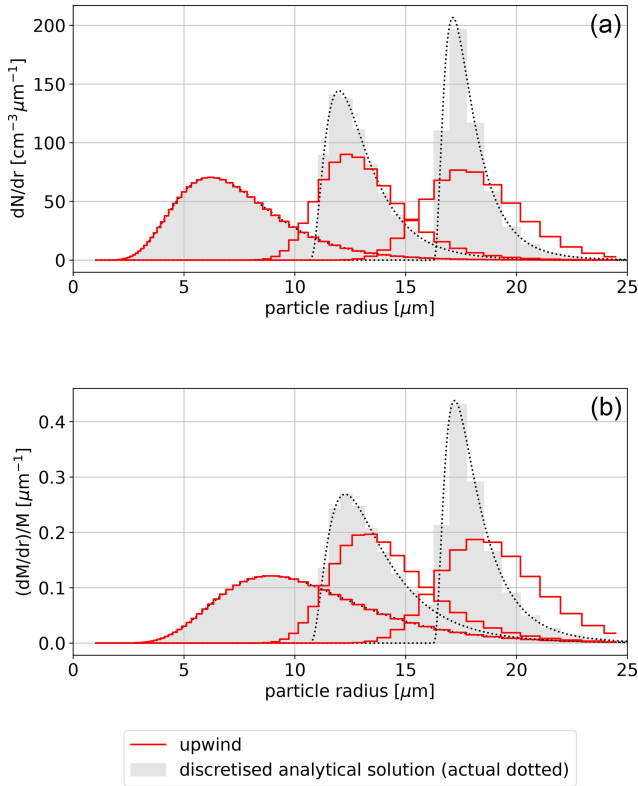
Figure 1. Evolution of the particle number density (a) and normalised mass density (b) with red histograms corresponding to the numerical solution using upwind scheme, black dots depicting analytical solution, and grey-filled histograms representing discretised analytical solution; compare with Fig. 3 in East (1957). Numerical solution was obtained with p = r^2 on a mass-doubling grid, i.e. with x = \ln_2(r^3) .
