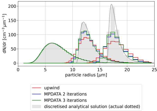
Figure 3. Comparison of analytical, upwind and MPDATA solutions (see plot key for algorithm variant specification) using the set-up from Fig. 1; see Sect. 2.4 for discussion.
