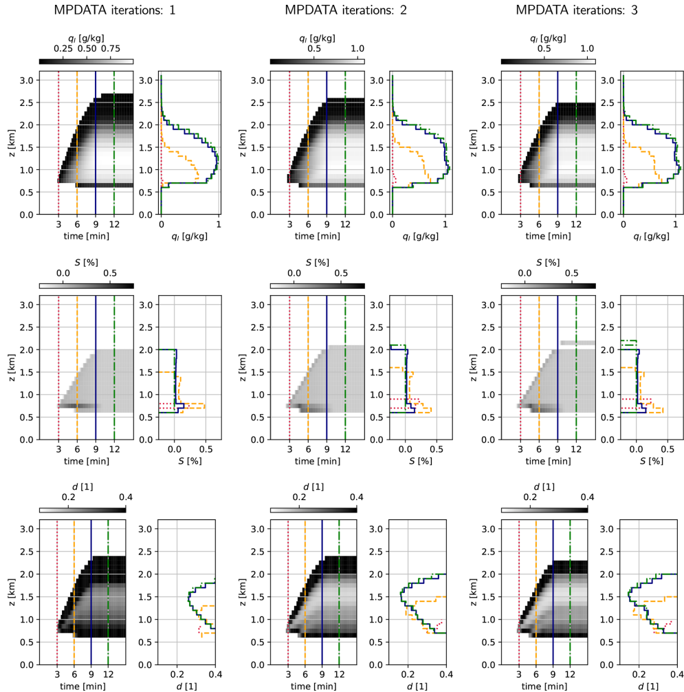
Figure 11. Single-column simulations depicted with three selected variables: liquid water mixing ratio q_l (top row), supersaturation S (middle row) and relative dispersion d (bottom row); for three settings of the iteration count in MPDATA (one iteration corresponding to the basic upwind scheme, left-hand column). Each of nine datasets (three iteration settings, three variables) is plotted with a greyscale time vs. altitude map (left-hand panels with the colour scale above) and a set of four profiles (right-hand panels). Profiles are plotted for t = 3 min (dotted, red), 6 min (dashed, orange), 9 min (solid, navy) and 12 min (dash-dot, green), with vertical lines of corresponding line style plotted at given times in the left-hand panels. For plotting, the model state is resampled by averaging in the time dimension to reduce the number of plotted steps by a factor of 50 (from 3600 down to 72).
