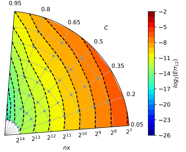
Figure A1. Convergence plot for the upwind scheme (cf. Fig. 1). Angle in the polar plot corresponds to the Courant number C ; the distance from origin denotes the number of grid boxes nx , see eq. (A2). Grey dots indicate data point locations – parameter values for which computations were made. Colours and isolines depict the error measure values (interpolated from the data point locations), see eq. (A1).
