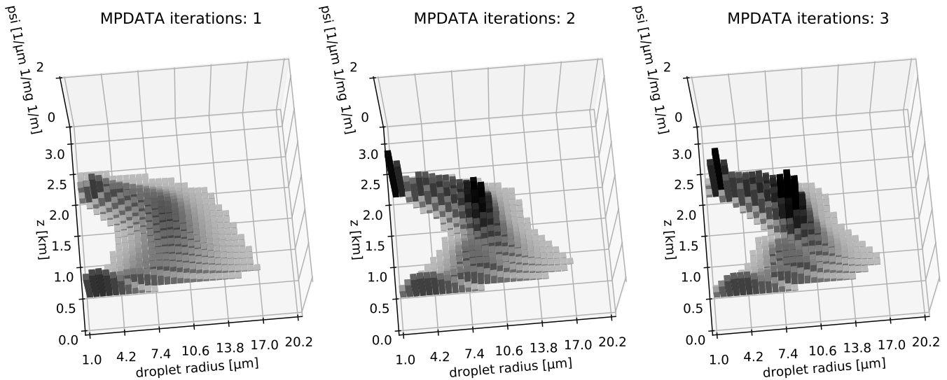
Figure 10. Snapshots of the advected two-dimensional liquid water field at t = t_1 = 600\text{s} for three simulations with different number of iterations settings of MPDATA iterations (with the non-oscillatory option enabled see text for details).
