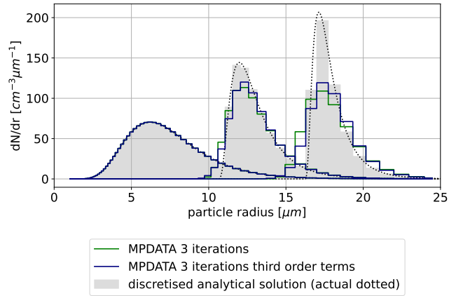
Figure 7. Comparison of analyticanalytical , upwind and MPDATA solutions (see plot key for algorithm variant specification) using the setup from Fig. 1, see sec. 2.9 for discussion.
