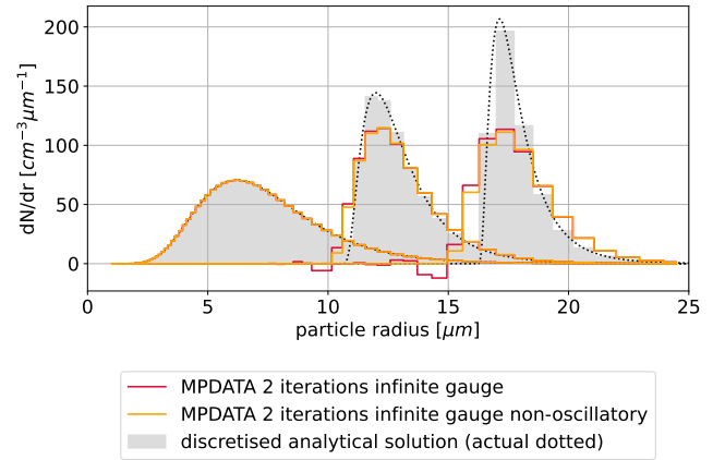
Figure 5. Comparison of analytical , upwind and MPDATA solutions (see plot key for algorithm variant specification) using the setup from Fig. 1, see sec. 2.6 for discussion.
