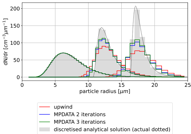
Figure 3. Comparison of analytic analytical, upwind and MPDATA solutions (see plot key for algorithm variant specification) using the setup from Fig. 1, see sec. 2.4 for discussion.
