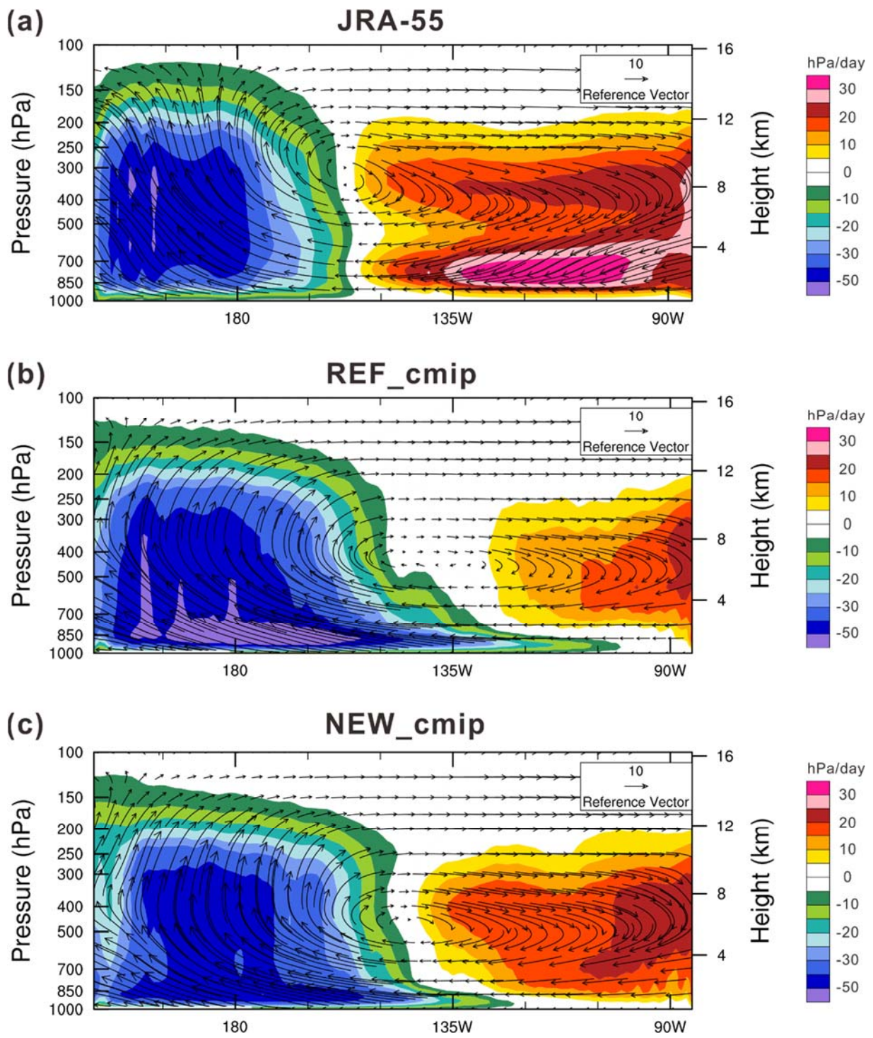
770 Figure 10. Annual mean vertical pressure velocity ( \text{hPa day}^{-1} ; shaded) and wind vectors (arrows) in the longitude-height cross section averaged over 5^{\circ}\text{S} - 10^{\circ}\text{S} for (a) the JRA-55 reanalysis, (b) REF_cmip, and (c) NEW_cmip.
