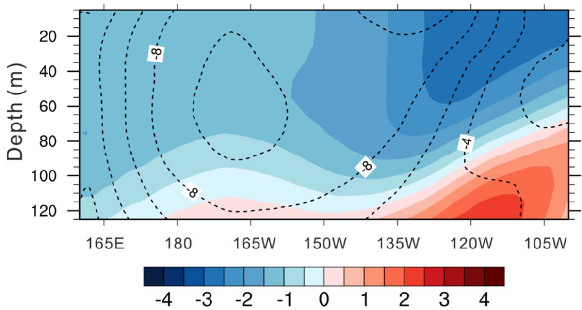
Figure 12. Longitude-depth cross section of zonal ocean current (contours; \text{cm s}^{-1} ) and temperature (shaded; ^{\circ}\text{C} ) averaged over over 5^{\circ}\text{S} - 10^{\circ}\text{S} for the difference between NEW_cmip and REF_cmip.
