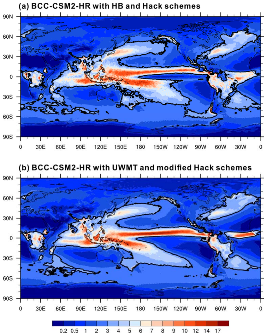
785 Figure 14. Annual mean precipitation rate ( \text{mm day}^{-1} ) from (a) intermediate version of BCC-CSM2-HR with original boundary-layer turbulence and shallow convection schemes, and (b) frozen version of BCC-CSM2-HR with new boundary-layer turbulence and shallow convection schemes. The 3 \text{ mm day}^{-1} contour is included in bold for reference.
