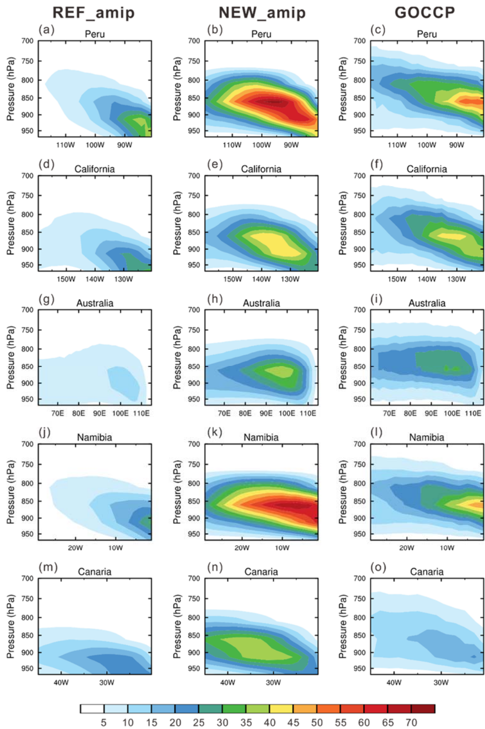
Figure 3. Cross sections of cloud fraction from five locations for (left) REF_amp, (center) NEW_amp, and (right) GOCCP. Refer to the boxes in Fig. 2 for the locations of the cross sections.
