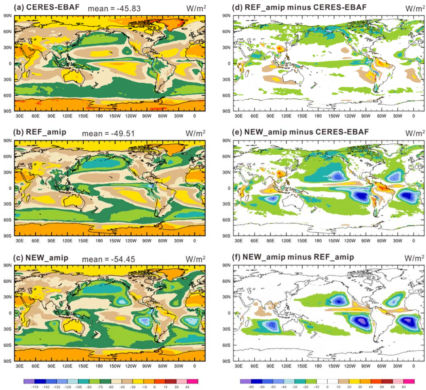
730 Figure 1. Annual mean climatologies of TOA SWCRF ( W m^{-2} ) from (a) CERES-EBAF observations (from 2001 to 2010), (b) REF_ampie, (c) NEW_ampie, and the differences between (d) REF_ampie and observations, (e) NEW_ampie and observations, (f) NEW_ampie and REF_ampie. Shown atop panels (a), (b) and (c) are global mean values.
