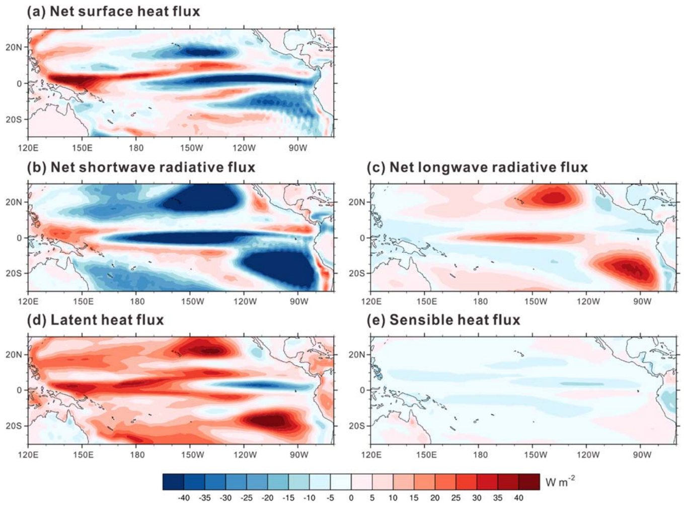
765 Figure 9. The differences between the NEW_cmip and REF_cmip simulations ( \text{W m}^{-2} ) for (a) net surface heat flux \Delta Q_{atm} , (b) net shortwave radiative flux \Delta Q_{SW} , (c) net longwave radiative flux \Delta Q_{LW} , (d) latent heat flux \Delta Q_{LH} , and (e) sensible heat flux \Delta Q_{SH} .
