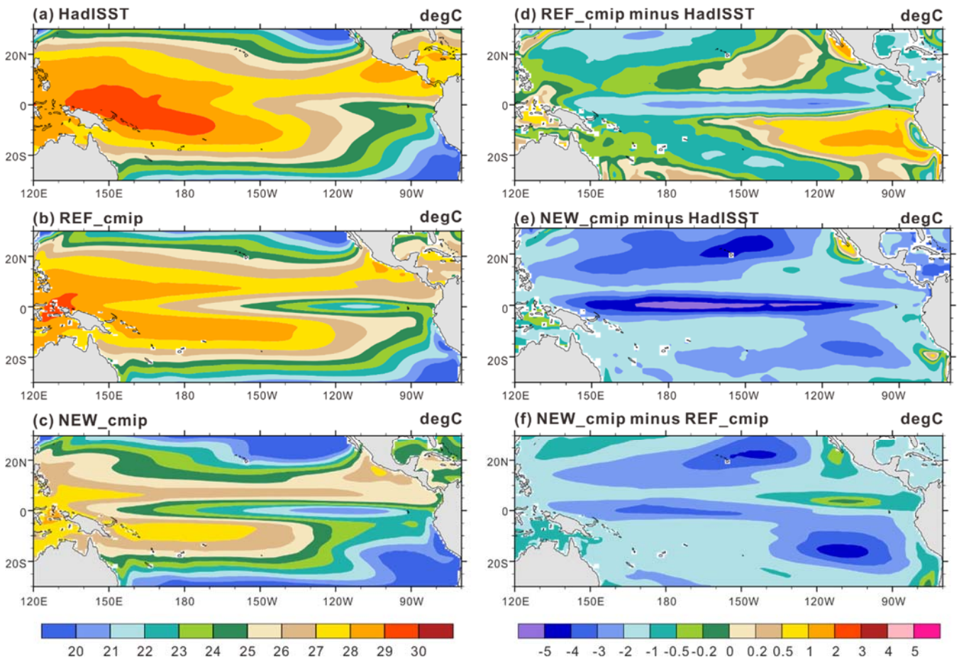
Figure 8. Annual mean sea surface temperature ( ^{\circ}\text{C} ) from (a) HadISST, (b) REF_cmip, and (c) NEW_cmip, and the difference between (d) REF_cmip and HadISST, (e) NEW_cmip and HadISST, and (f) NEW_cmip and REF_cmip.
