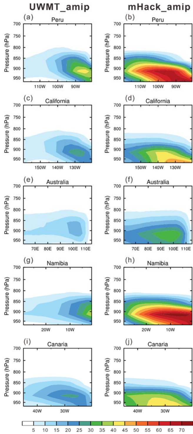
Figure 13. Cross sections of cloud fraction from five locations for (left) UWMT_ami, and (right) mHack_ami. Refer to the boxes in Fig. 2 for the locations of the cross sections.
