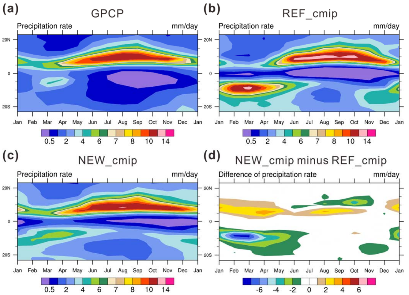
760 Figure 7. Seasonal cycle of precipitation rate (mm day -1 ) averaged over eastern Pacific (90° - 160°W) for (a) GPCP, (b) REF_cmip, (c) NEW_cmip, and (d) the difference between NEW_cmip and REF_cmip.
