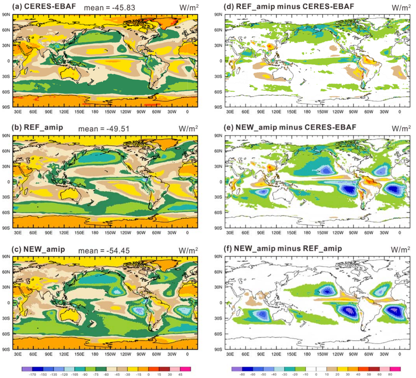
Figure 1. Annual mean climatologies of TOA SWCRF ( \text{W m}^{-2} ) from (a) CERES-EBAF observations (from 2001 to 2010), (b) REF_amip, (c) NEW_amip, and the differences between (d) REF_amip and observations, (e) NEW_amip and observations, (f) NEW_amip and REF_amip. Shown atop panels (a), (b) and (c) are global mean values.
