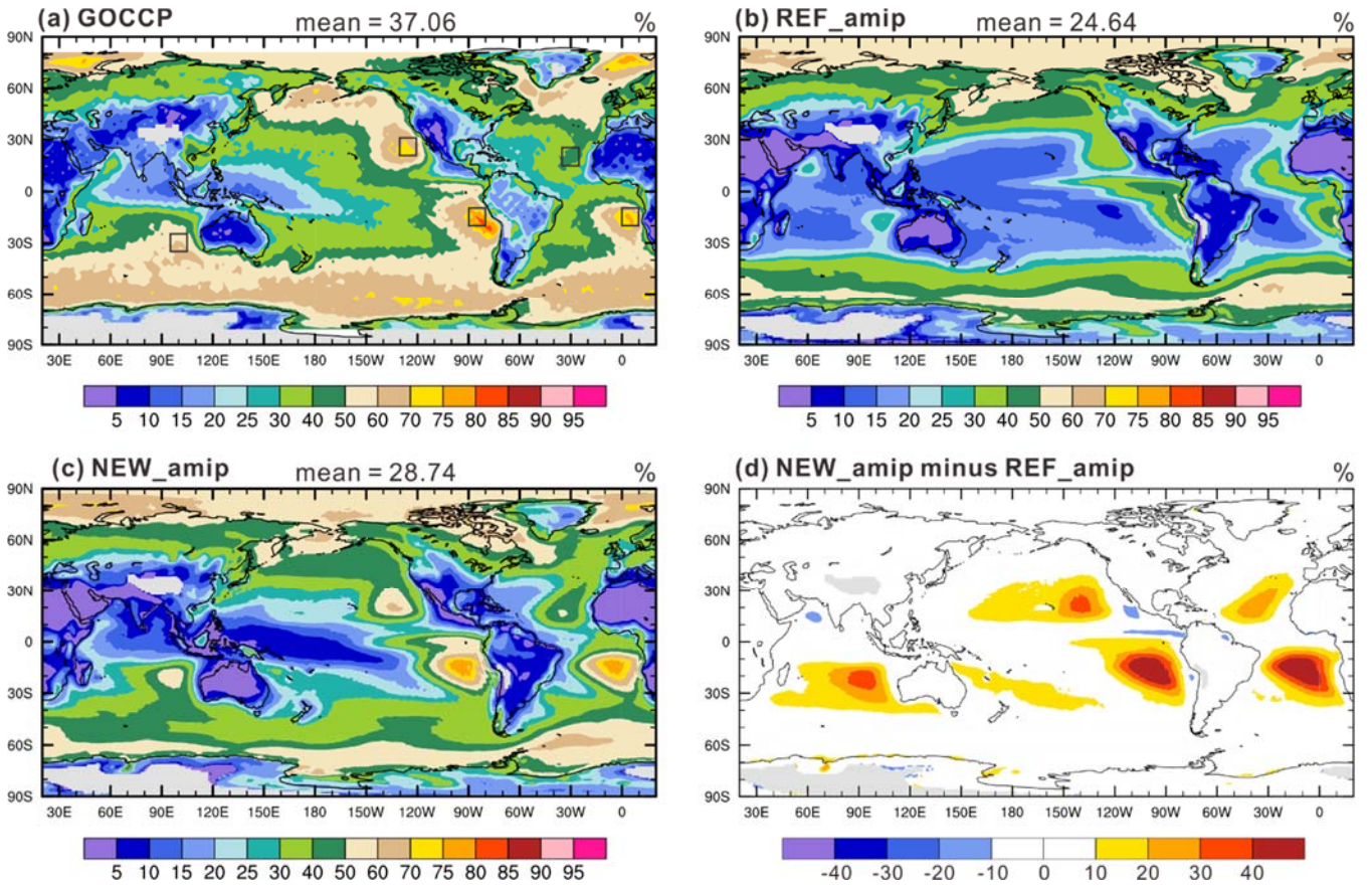
Figure 2. Annual mean low-level cloud fraction (%) from (a) GOCCP (from 2007 to 2012), (b) REF_amip, (c) NEW_amip, and (d) the difference between NEW_amip and REF_amip. Shown atop panels (a), (b) and (c) are global mean values. Boxes in panel (a) indicate the five main subtropical marine stratocumulus regions, namely, Peru (10°-20°S, 80°-90°W), California (20°-30°N, 120°-130°W), Australia (25°-35°S, 95°-105°E), Namibia (10°-20°S, 0°-10°E), and Canaria (15°-25°N, 25°-35°W).
