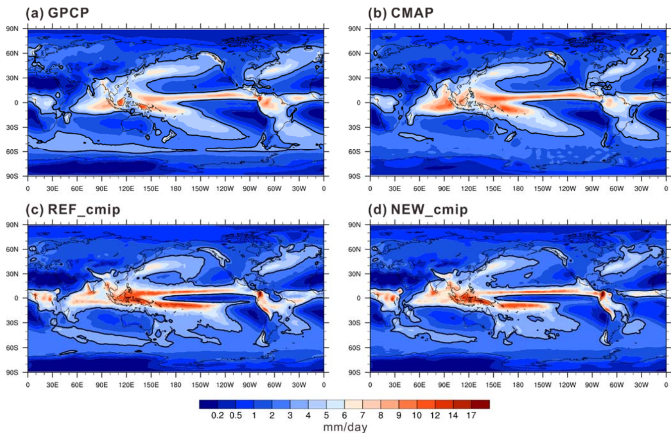
Figure 4. Annual mean precipitation rate (mm day -1 ) from (a) GPCP, (b) CMAP, (c) REF_cmip, and (d) NEW_cmip. The 3 mm day -1 contour is included in bold for reference.
