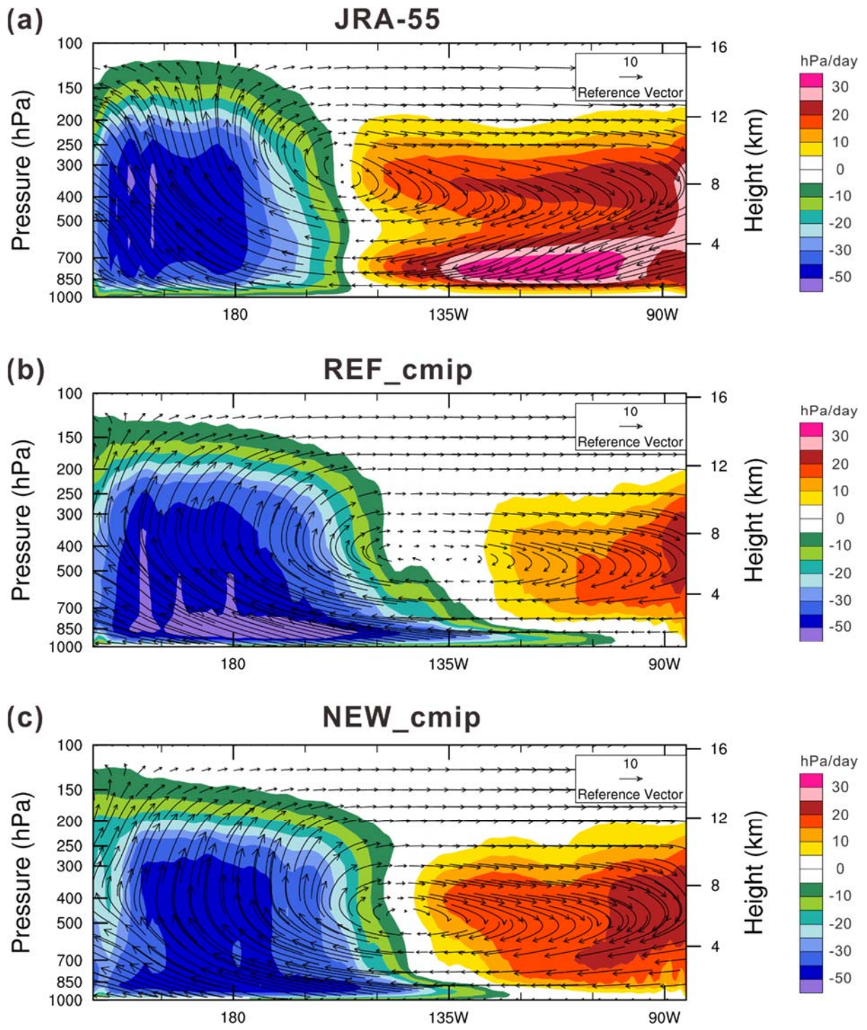
Figure 10. Annual mean vertical pressure velocity ( \text{hPa day}^{-1} ; shaded) and wind vectors (arrows) in the longitude-height cross section averaged over 5°S – 10°S for (a) the JRA-55 reanalysis, (b) REF_cmip, and (c) NEW_cmip.
