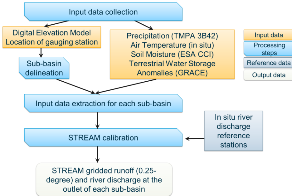
Figure 2. Processing steps of the STREAM v1.3 model.
