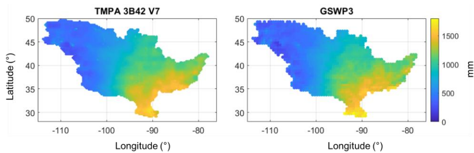
Figure S1. Mean annual precipitation data over the period 2003-2014 obtained by TMPA 3B42 V7 and GSWP3 datasets over the Mississippi river basin.
