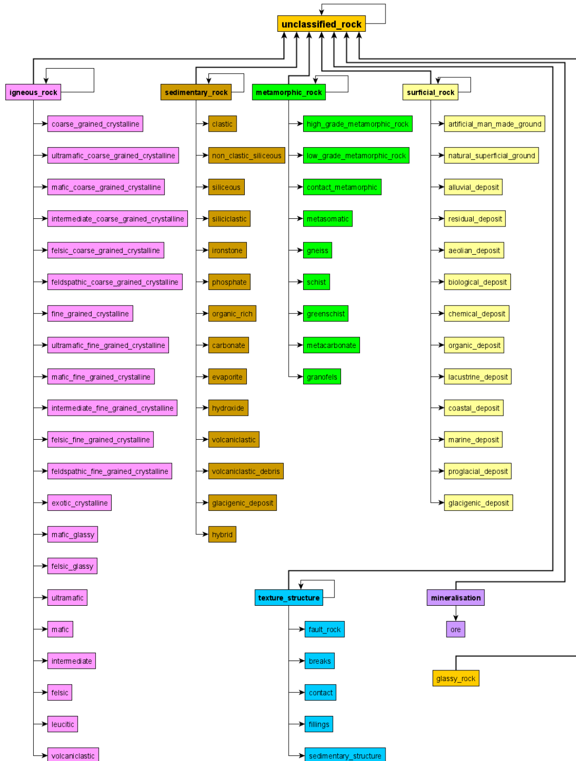
200 Figure 1. Lithology Hierarchical Thesaurus showing the 7 major Lithology_Groups: Igneous rocks (pink), Sedimentary rocks (light brown), Metamorphic rocks (green), Surficial Rocks (light yellow), Texture and Structure (blue), Mineralisation (purple) and Unclassified Rocks (dark yellow) and their corresponding Lithology_Subgroups .
