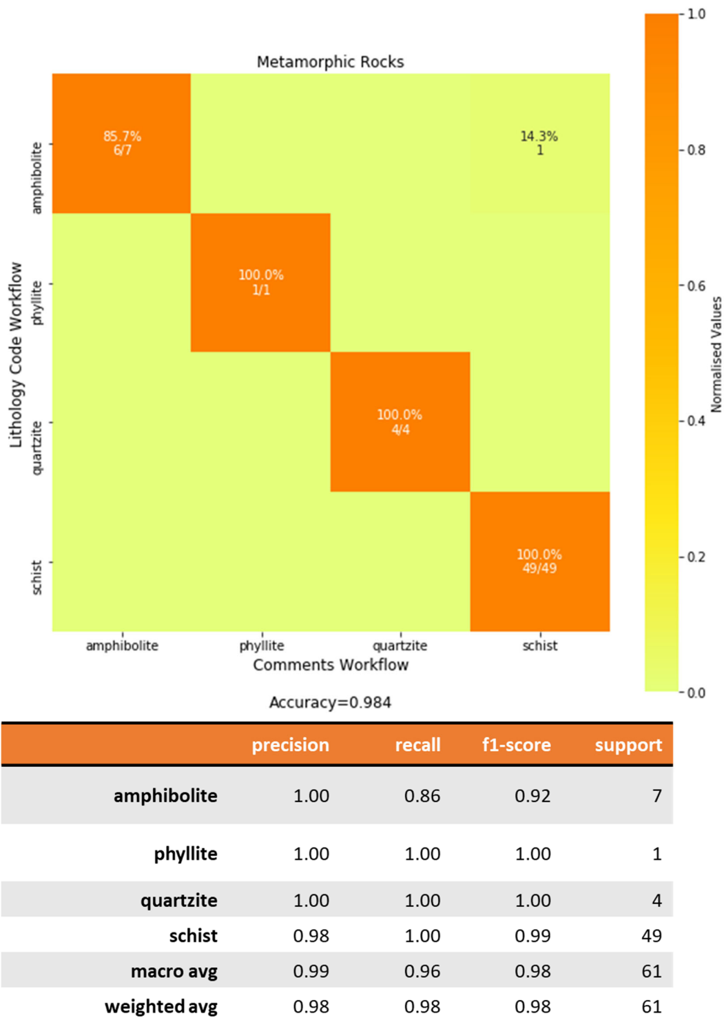
575 Figure 10. Confusion matrix for metamorphic rocks comparing the fuzzy string matching results from the Lithology Code workflow (vertical axis) and Comments workflow (horizontal axis). The heatmap shows the values normalised to the support size to address the imbalance between classes. The values shown in the cells indicate the number of samples classified for the class. Empty cells indicate zero samples.
