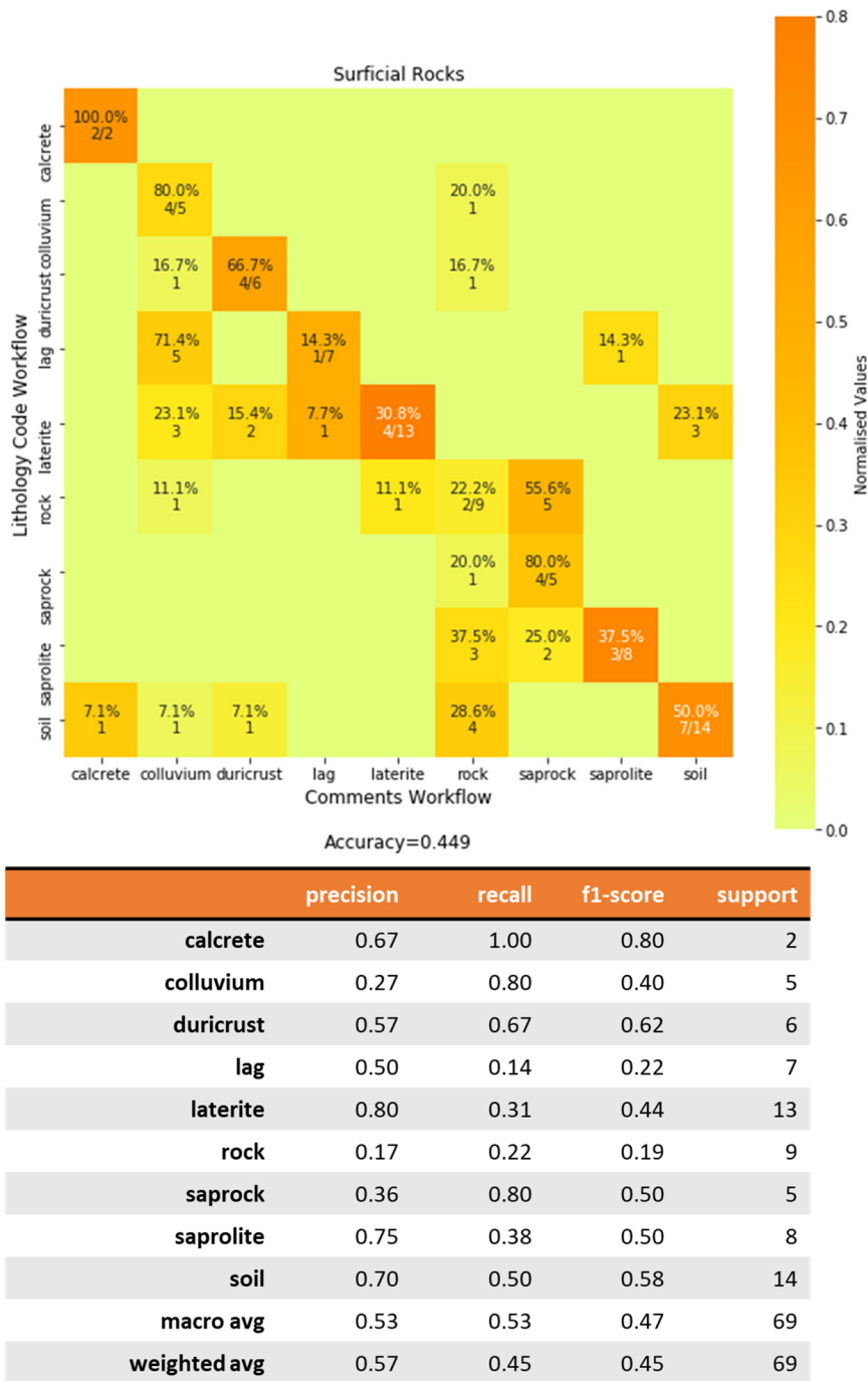
Figure 11. Confusion matrix for surficial comparing the fuzzy string matching results from the Lithology Code workflow (vertical axis) and Comments workflow (horizontal axis). The heatmap shows the values normalised to the support size to address the imbalance between classes. The values shown in the cells indicate the number of samples classified for the class. Empty cells indicate zero samples
