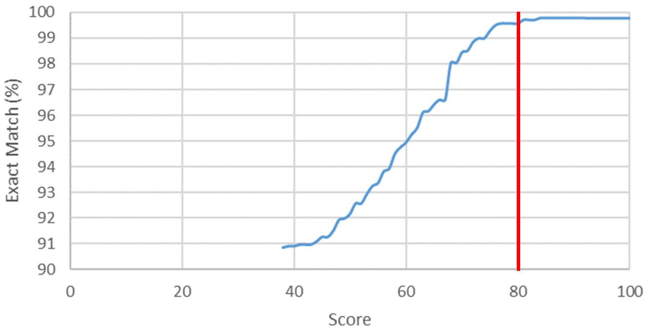
415 Figure 6. The user-defined cut-off score of 80 is chosen based on the results of the testing different cut-offs on a smaller dataset within the YSGB area. As seen in this figure, the number of exact matches plateau at a score of 80.
