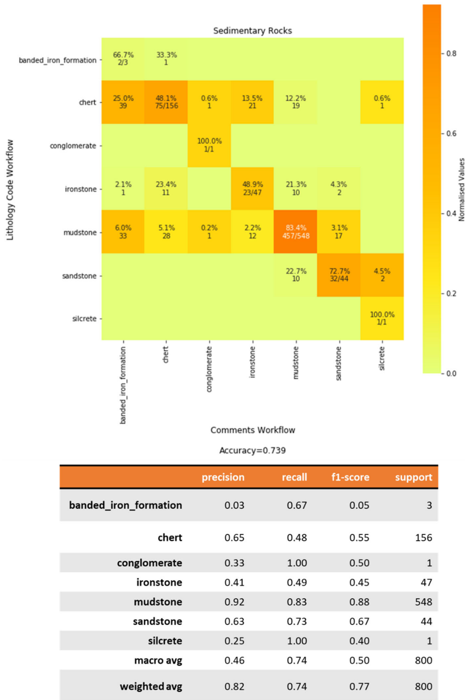
725 Figure 13. Confusion matrix for sedimentary rocks comparing the fuzzy string matching results from the Lithology Code workflow (vertical axis) and Comments workflow (horizontal axis). The heatmap shows the values normalised to the support size to address the imbalance between classes. The values shown in the cells indicate the number of samples classified for the class. Empty cells indicate zero samples. The accuracy is 73.9%, with a weighted average precision of 82% and recall of 74%. These results are taken from a subset of 800 samples across 7 classes.
