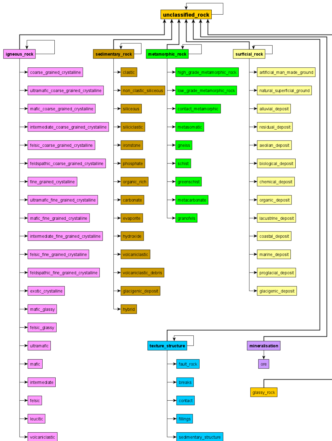
255 Figure 3. Lithology Hierarchical Thesaurus showing the 7 major Lithology_Groups: Igneous rocks (pink), Sedimentary rocks (light brown), Metamorphic rocks (green), Surficial Rocks (light yellow), Texture and Structure (blue), Mineralisation (purple) and 260 Unclassified Rocks (dark yellow) and their corresponding Lithology_Subgroups. Many of the Lithology_Subgroups listed have parent-child relationships e.g. 'mafic_fine_grained_crystalline' is a child of 'mafic'. Parents in parent-child relationships are 265 included in their children as catch-all groups to capture free text descriptions that do not include details that would be captured by only using the child terms alone. Igneous rocks Lithology_Subgroups are further classified to 12 lithology subgroups, 270 considering grain size, composition and a combination of both. Sedimentary rocks are subclassified to 16 Lithology_Subgroups based on genetic source and composition (carbonate, clastic, evaporate, hybrid, hydroxide, ironstone, non-clastic siliceous, organic-rich, phosphate, siliceous, siliciclastic, volcaniclastic, glacigenic). Metamorphic rocks are subdivided into Lithology_Subgroups based on the degree and type of metamorphism (metasomatic, contact, low-grade, schist, gneiss, high-grade, granofels, greenschist, metacarbonate). Surficial rocks are subdivided into 13 Lithology_Subgroups based on the depositional environment and composition. The residual deposit Lithology_Subgroup includes the regolith detailed lithologies. Mineralisation is considered as a separate classification to be able to classify ore zones. Structure and texture addresses situations that structures are logged as lithologies in geological logging. Structure and Texture is divided into five Lithology_Subgroups: fault rock, breaks, contact, fillings and sedimentary structures. The final classification is a catch-all for unclassified rocks. The matching is done at the Detailed_Lithology level, thus not causing confusion in the Lithology_Subgroup and Lithology_Group level. Volcaniclastics are present in both lithological groups as although volcaniclastics are volcanic in origin and are categorized as igneous rocks, ambiguous lithologies such as “metavolcaniclastic_sandstone” is more sedimentary than igneous.
