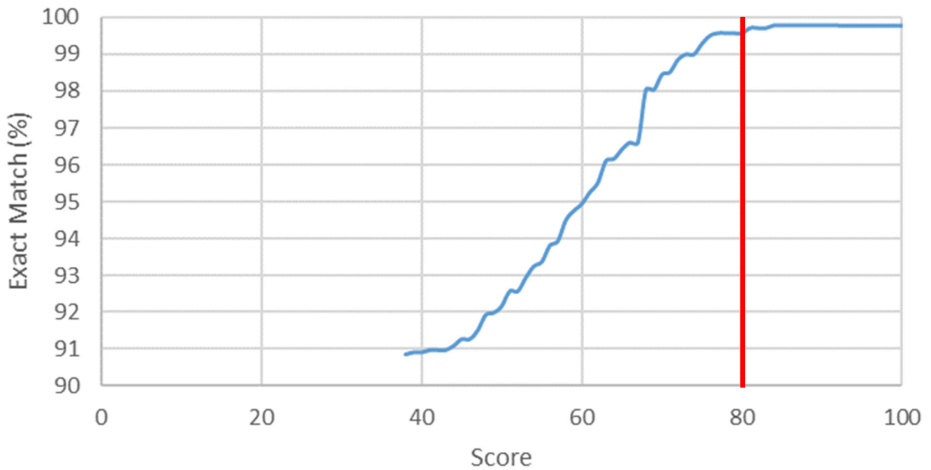
575 Figure 10. The user-defined cut-off score of 80 is chosen based on the results of the testing different cut-offs on a smaller dataset within the YSGB area. As seen in this figure, the number of exact matches plateau at a score of 80. This relationship may vary depending on the datasets available in the area. Thus, this cut-off value is user-defined and is best to test the matching performance on a subset in the user's area. The number of exact matches plateau at a score of 80 giving a realistic cut-off and avoids an overly stringent threshold of 100, where useful matches may not be captured.
