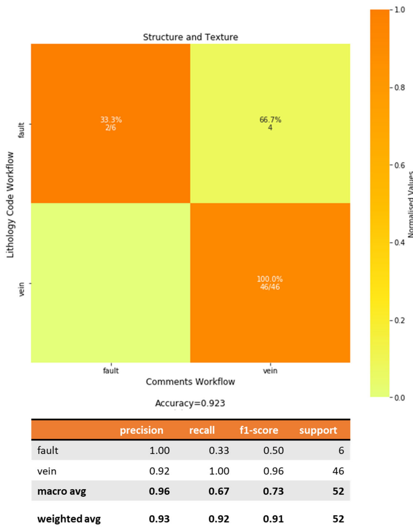
680 Figure 11. Confusion matrix for structure and texture comparing the fuzzy string matching results from the Lithology Code workflow (vertical axis) and Comments workflow (horizontal axis). The heatmap shows the values normalised to the support size to address the imbalance between classes. The values shown in the cells indicate the number of samples classified for the class. Empty cells indicate zero samples. The Structures and Texture Lithology_Group had an accuracy of 92.3% across 52 samples, 46 for veins and 6 for faults.
