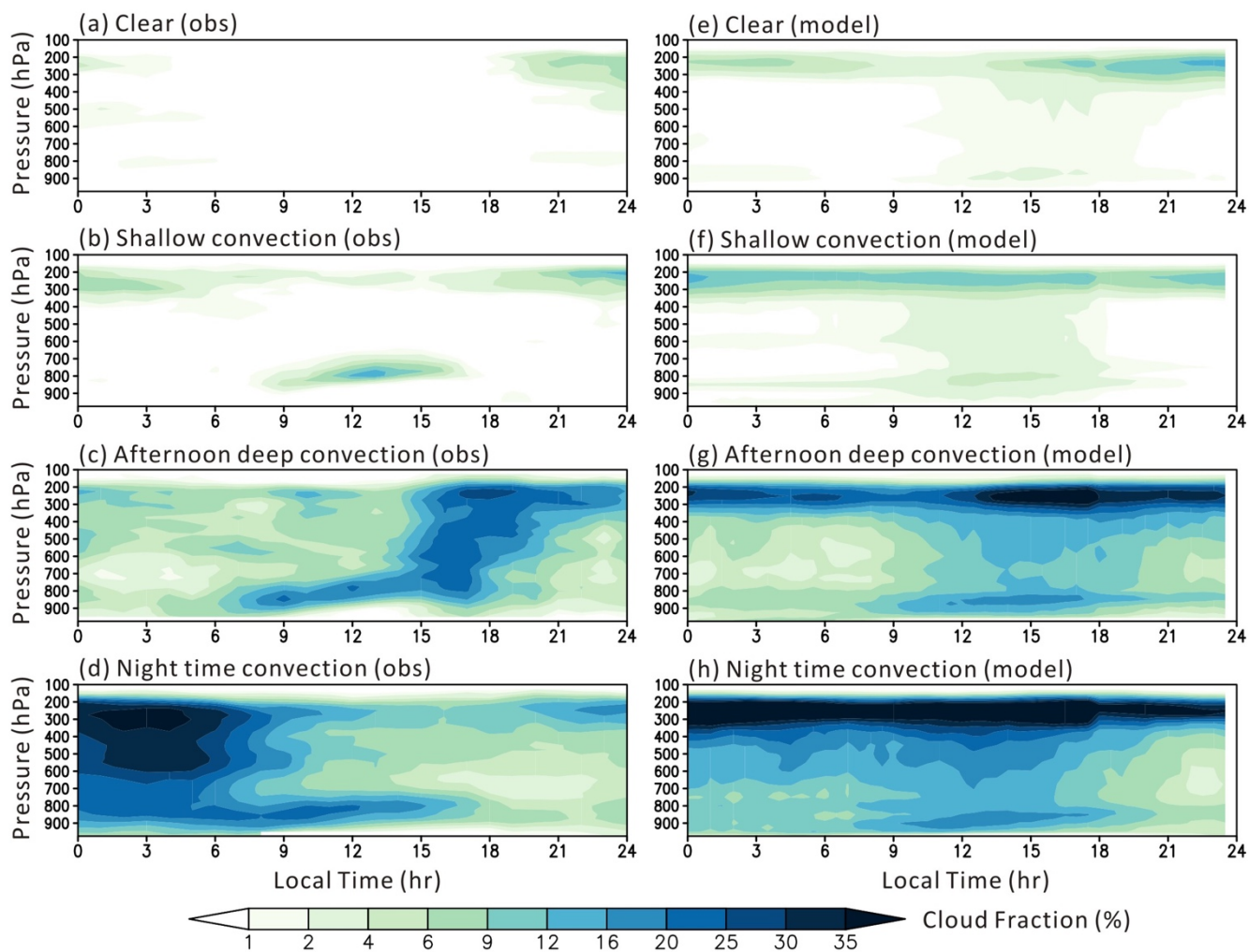
Figure 3: Diurnal cycle of cloud fraction composites (%) from May to August in the years of 1997 to 2007 from (a)–(d) ARMBE ARSCL and (e)–(h) Day 2 hindcasts for different convection regimes: (a)(e) clear-sky regime, (b)(f) fair-weather shallow cumulus regime, (c)(g) late-afternoon deep convection regime, and (d)(h) nighttime deep convection regime. Figures (a)–(d) were modified from Figure 3 in Zhang and Klein (2010).
