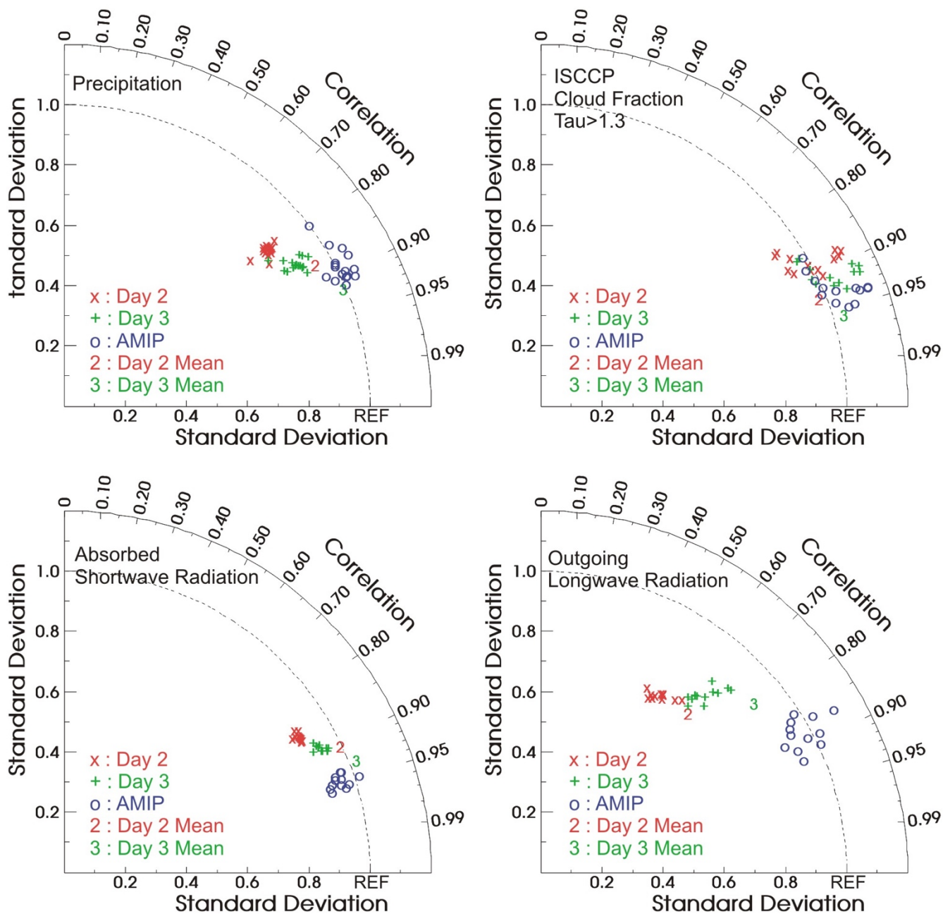
Figure 8: Spatial pattern statistics of the bias errors (with respect to observations) of annual mean precipitation, ISCCP total cloud fraction (with tau > 1.3), absorbed shortwave radiation, and outgoing longwave radiation from the multi-year CAM5 hindcasts and an AMIP simulation. These statistics are illustrated with a Taylor diagram (Taylor et al. 2001) that shows the level of agreement of a given field to a common reference. The reference fields (REF) are the correspondent multi-year mean bias errors from the AMIP simulation. Each “x”, “+”, or “o” represents the Day 2, Day 3 or AMIP annual mean bias for individual years between 1997 and 2012 whenever the observations are available, and “2” and “3” represents the Day 2 and Day 3 hindcast mean biases averaged over all available years, respectively.
