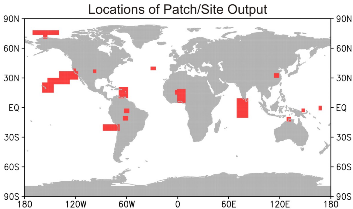
Figure 2: Locations of model patch/site output associated with major field campaigns or U.S. Department of Energy Atmospheric Radiation Measurement (ARM) sites. See Table 1 for detailed longitude and latitude information.
