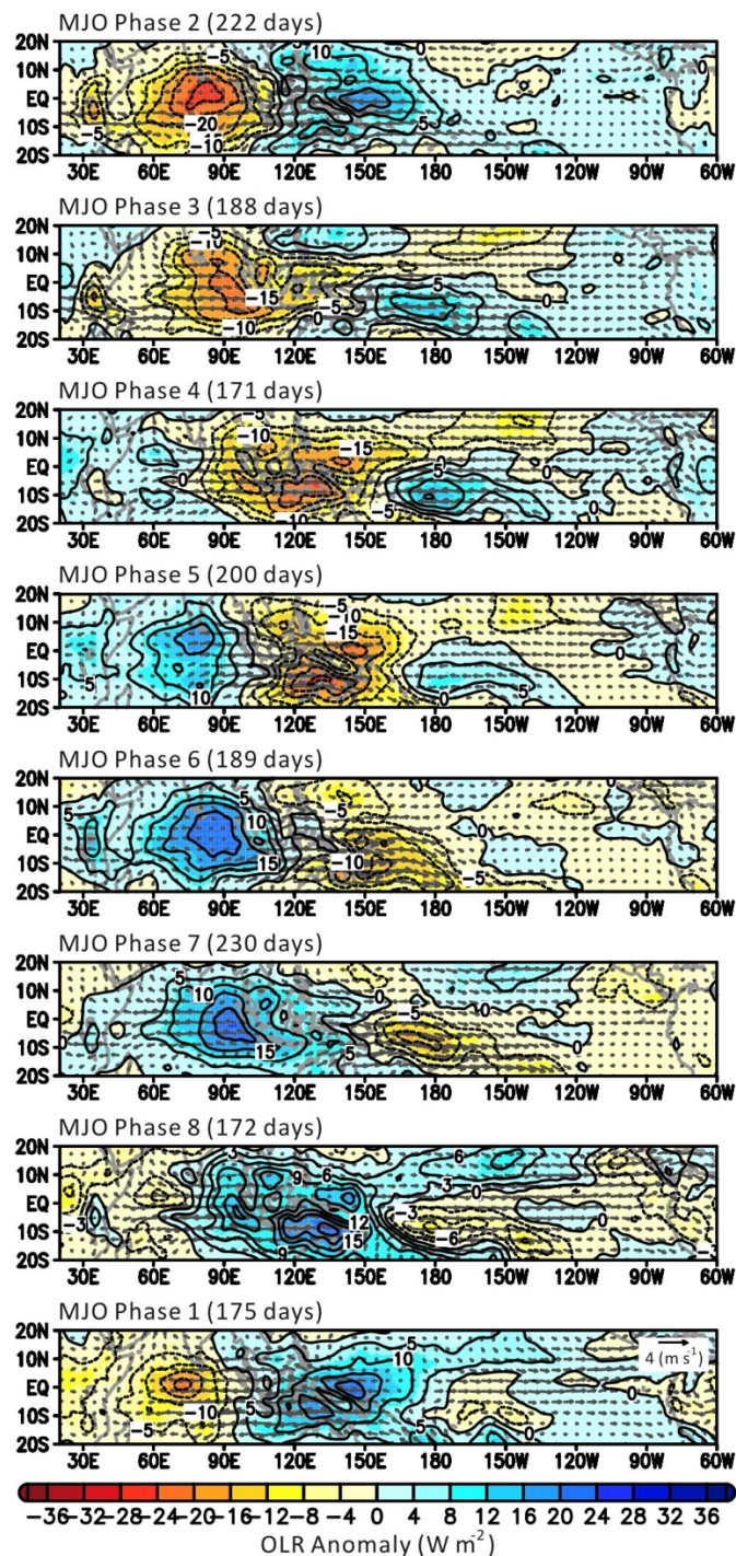
650 Figure 4: Composites of November to April 20-100 day band-pass filtered NOAA Interpolated Outgoing Longwave Radiation anomalies (color shades and contours, \text{W m}^{-2} ) and horizontal wind anomalies (vectors, \text{m s}^{-1} ) at 850mb from ERA-Interim, as a function of the eight phases of the MJO (Wheeler and Hendon 2004). Number of days for composites are indicated on the top of each panel. Years of analysis are from 1997 to 2012.
