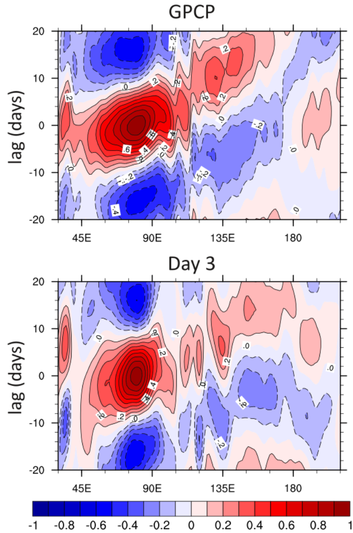
Figure 6: Time-longitude anomalous rainfall correlation Homvöller diagram along the Equator (10°S - 10°N) based on GPCP and Day3 hindcasts. The rainfall anomalies associated with the MJO are derived based on lag-correlation over an Indian Ocean box (75°-85°E; 5°S-5°N) for northern winter (November-April) of 1997 to 2012.
