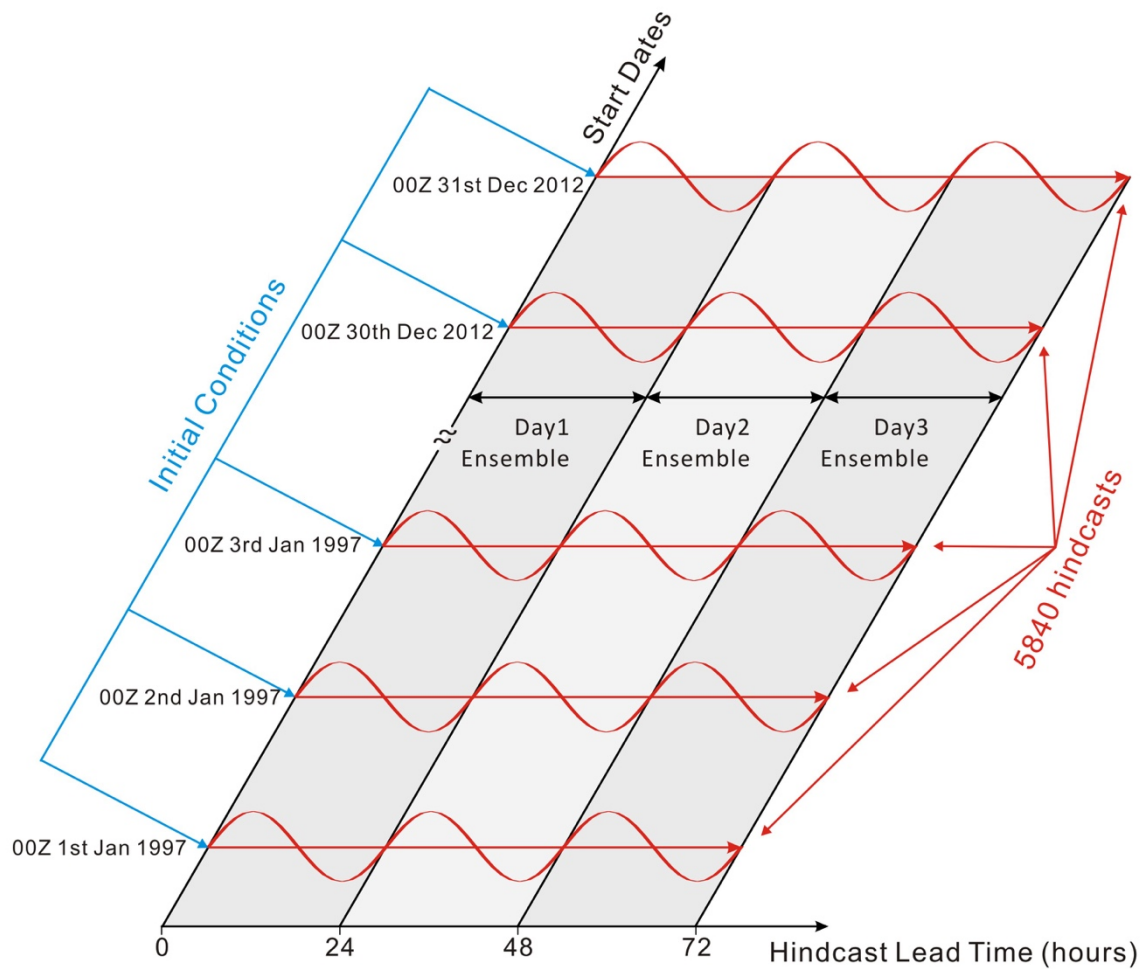
Figure 1: Schematic diagram for the multi-year hindcast procedure (modified from Ma et al. 2015) applied to series of three-day 635 hindcasts from 1997 to 2012. Each hindcast is initialized with ERA Interim Reanalysis and the starting time is 00Z every day.
