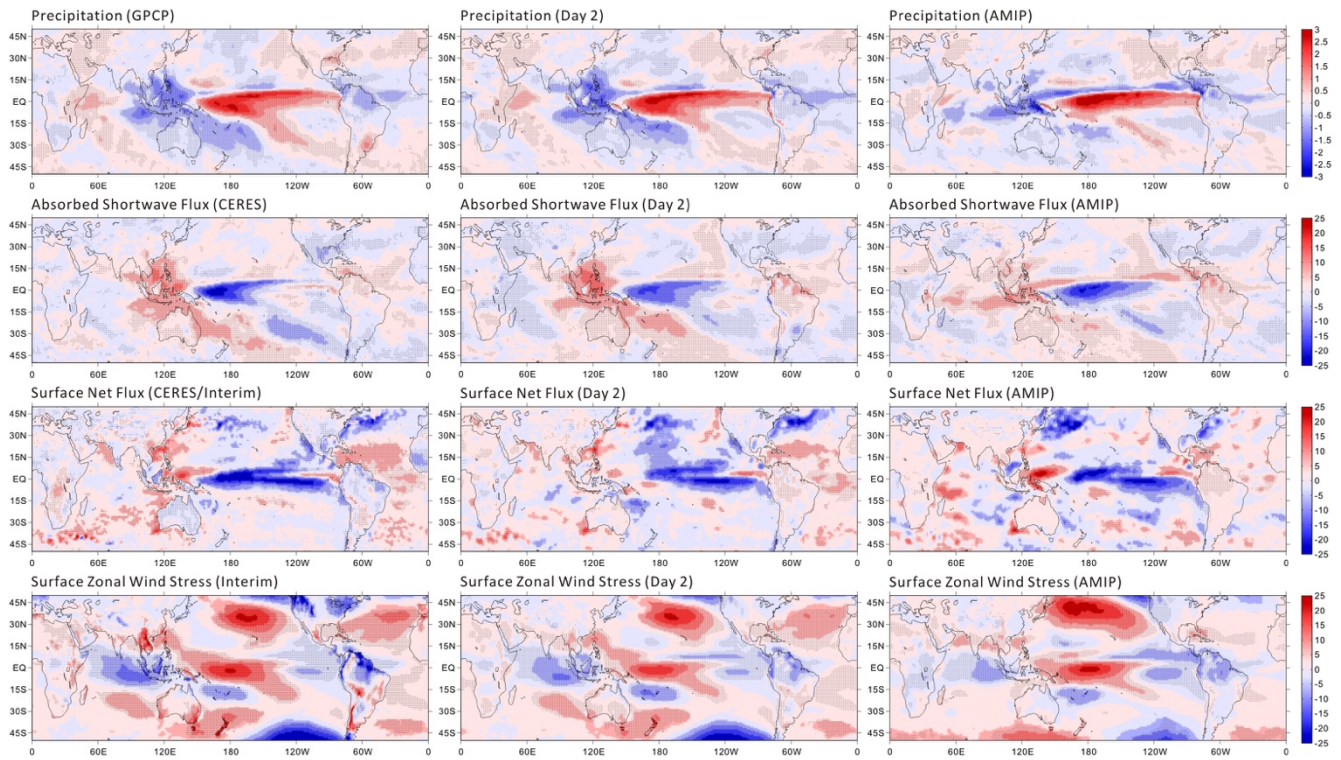
Figure 7: Regression maps of precipitation ( \text{mm day}^{-1} \text{K}^{-1} ), absorbed shortwave radiation ( \text{W m}^{-1} \text{K}^{-1} ), net surface heat flux ( \text{W m}^{-1} \text{K}^{-1} ), surface zonal wind stress ( \text{N m}^{-2} \text{K}^{-1} ) onto the Niño 3.4 index from observations (left panels), Day 2 hindcasts (middle panels), and AMIP simulation (right panels).
