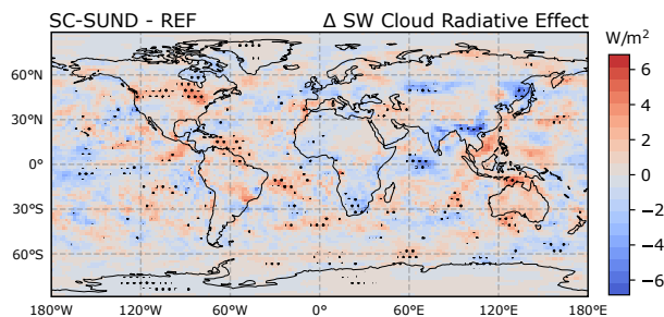
Figure 10. SW CRE difference between the REF and SC-SUND simulations. Stippling indicates statistically significant differences at the 95 % significance level; the false discovery rate is controlled following Wilks (2016).
