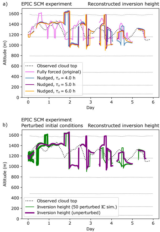
Figure B1. Reconstructed inversion heights in modified EPIC SCM experiments, (a) with different nudging relaxation timescales \tau_x ; (b) with \tau_x = 5\text{h} and perturbed initial conditions.
