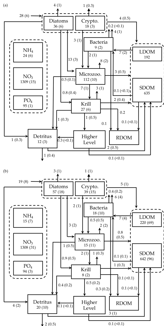
Figure 7. Depth-integrated (0–60 m) carbon stocks (mmol C m -3 ), flows (mmol C m -3 d -1 ), and POC export flux at 60 m (mmol C m -2 d -1 ) averaged over the modeled austral growth season (October 2002–March 2003) before (a) and after optimization (b). Values in parentheses as uncertainties from season averaging (a) and as uncertainties propagated from season averaging and depth integration of the Monte Carlo errors for panel (b).
