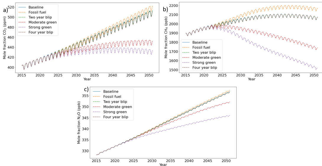
Figure 1. Concentrations for the three persistent GHGs, a) CO 2 , b) CH 4 , c) N 2 O. In each case the baseline data is very similar to 2-year blip after 2025: two and four year blips, hence the difficulty distinguishing the lines.
