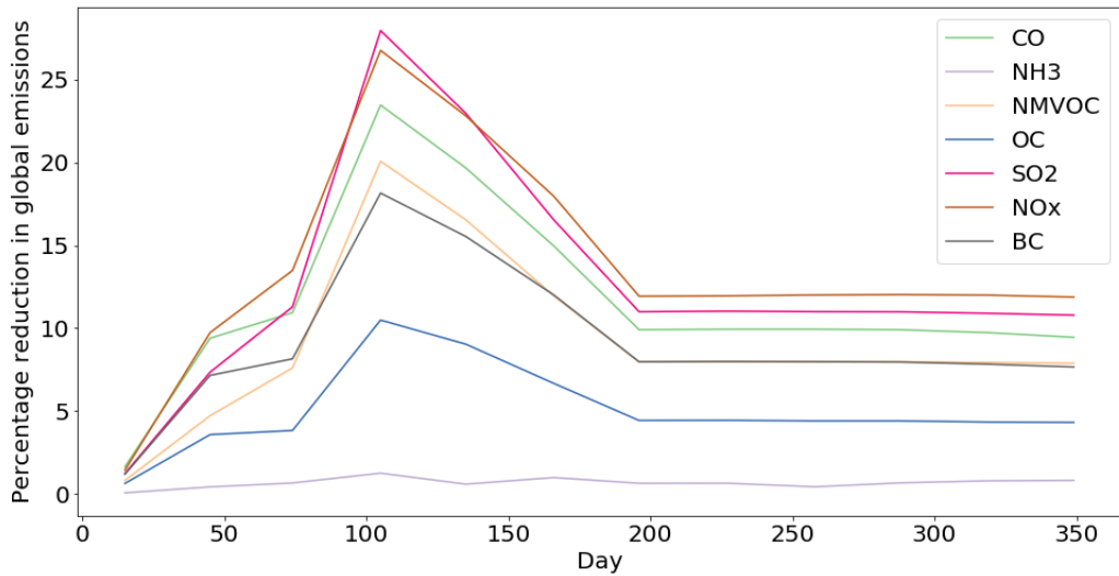
Figure 3. Monthly global emissions reduction estimates for 2020.
