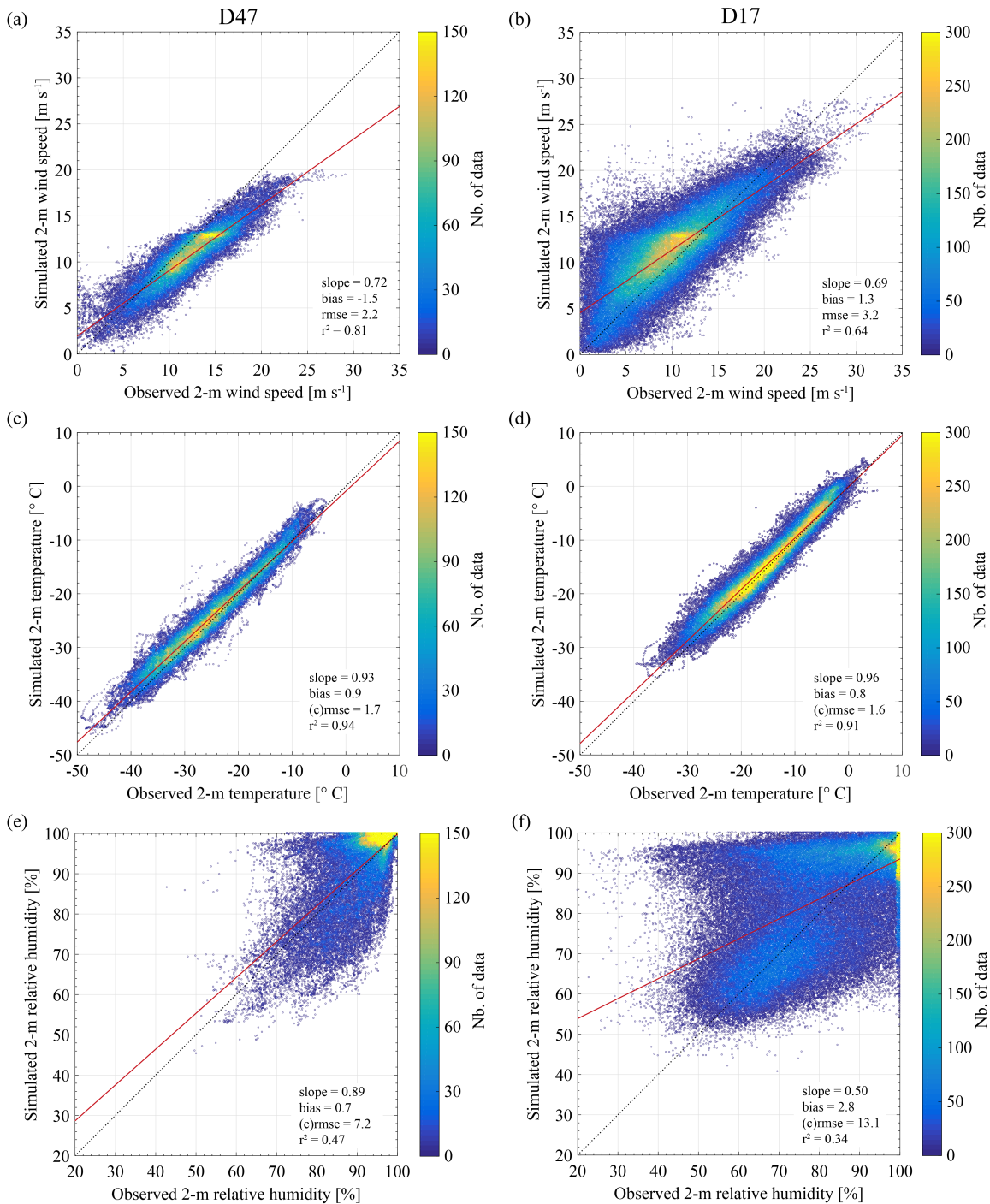
Figure 3. Scatter-Density scatter plots of observed vs. simulated half-hourly wind speed (top), air temperature (middle) and air relative humidity with respect to ice (bottom) at 2 m height for stations D47 (left) and D17 (right). The coloured lines show the 1:1 line (dashed black) and the best linear fit (red).
