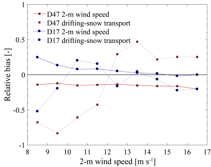
Figure 8. Relative bias in mean wind-speed-wind speed (solid curves) and cumulated snow transport (dashed curves) during drifting-snow events. Relative biases are expressed as the ratio of the difference between model and observation to the observation and shown as median values within wind-speed-observed wind speed bins of 1 \text{ m s}^{-1} at D47 (red curves) and D17 (blue curves).
