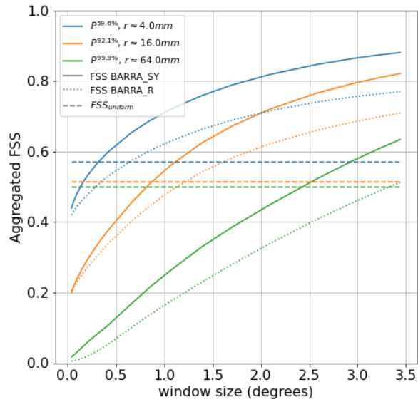
Figure 10: Aggregated FSS across 1323 6-hour storm events as a function of neighbourhood distance (degrees) for 6-hour rainfall above three percentile thresholds (distinguished by colours, percentile values, and observed amount in mm). The solid curves indicate the score for BARRA-SY, dotted curves for BARRA-R, and the dashed horizontal lines the uniform score ( FSS_{uniform} ) for each threshold as specified by Roberts and Lean (2007).
