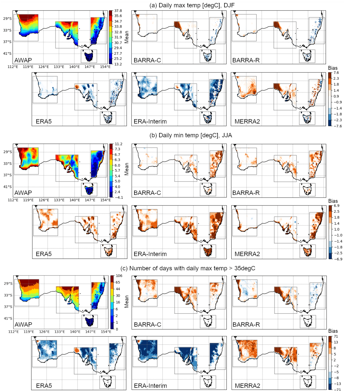
820 Figure 3: Mean difference in (a) summer (DJF) daily maximum temperature, (b) winter (JJA) daily minimum temperature and (c) number of days with temperature exceeding 35 °C, in various models during 1990-2018, with respect to AWAP. The models are regridded onto the AWAP grid using nearest-neighbour interpolation.
