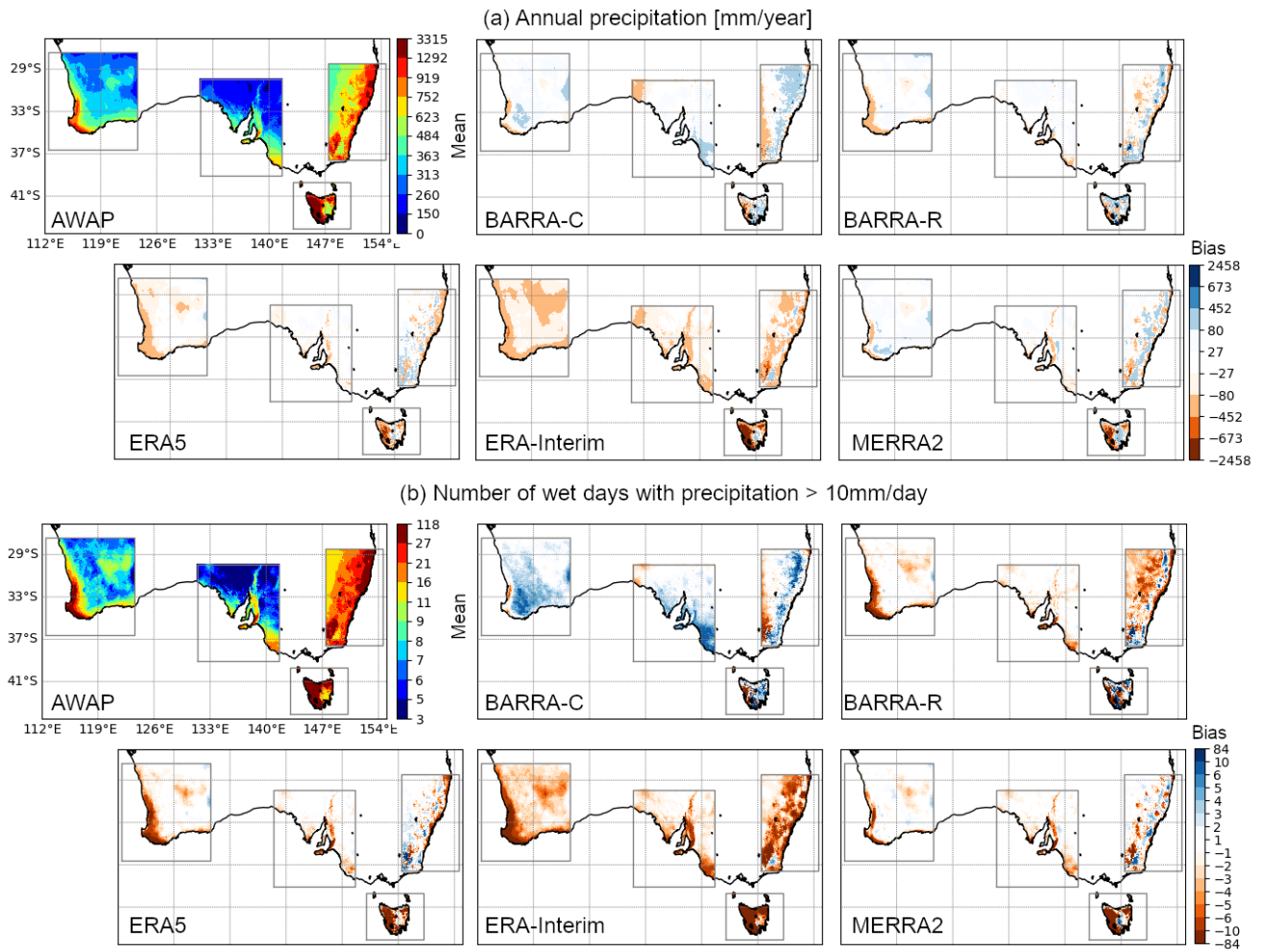
835 Figure 7: Mean difference in (a) annual precipitation and (b) annual count of wet days with depth \geq 10 mm. The models are regrided onto the AWAP grid using nearest-neighbour interpolation.
