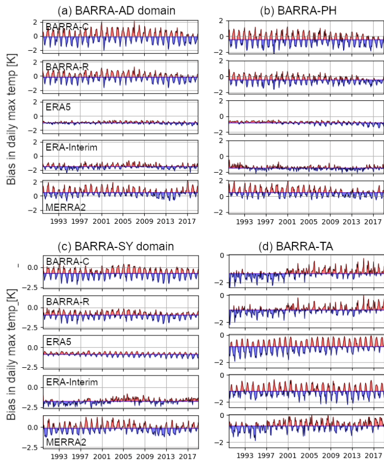
825 Figure 4: Timeseries of monthly mean difference in daily maximum temperature averaged over various BARRA-C domains with respect to AWAP. The timeseries are shaded around their individual 1990-2018 means.
