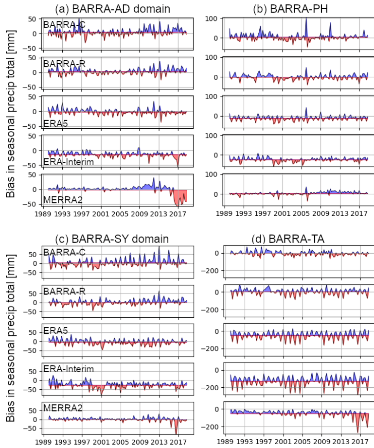
840 Figure 8: Mean difference in seasonal precipitation totals over various BARRA-C domains with respect to AWAP. Black curves are shaded around the 1990-2018 means. Note that the y-axes in (a)-(d) are different.
