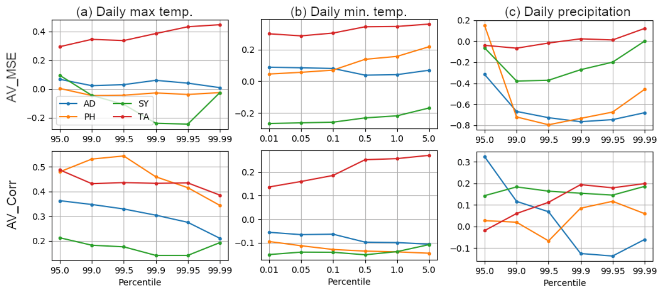
Figure 11: Added value (AV) analysis of the (a) warm extreme of daily maximum temperature, (b) cold extreme of daily minimum temperature, and (c) wet extreme of daily precipitation, for all four BARRA-C domains.
