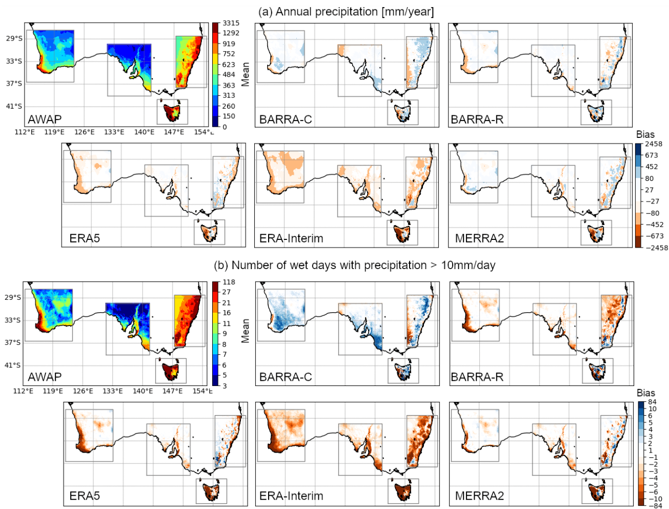
Figure 7: Mean difference in (a) annual precipitation and (b) annual count of wet days with depth \geq 10 mm. The models are regridded onto the AWAP grid using nearest-neighbour interpolation.
