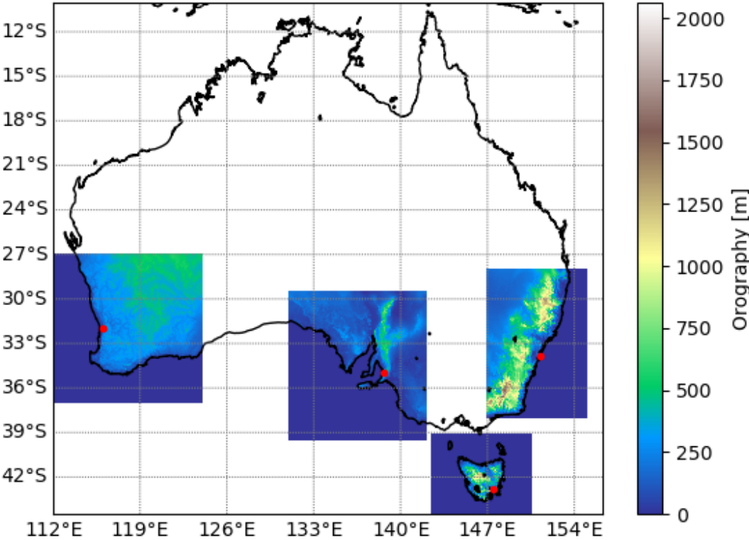
805 Figure 1: Domains of BARRA-C, (left to right) BARRA-PH (over Perth), BARRA-AD (Adelaide), BARRA-TA (Tasmania), and BARRA-SY (Sydney), showing the modelled orography. Red circles indicate the locations of the state capital cities.
