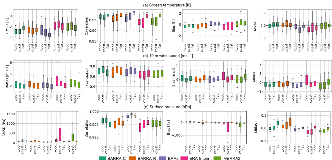
810 Figure 2: Box plots showing the distribution of evaluation scores of various models for (a) screen-level temperature, (b) 10 m wind speed, and (c) surface pressure across the four BARRA-C domains. Three regions are analysed separately: coastal ('coast'), complex topography ('topo'), and flat, and the models distinguished by colours. The scores are calculated on model hindcasts valid between 05-07 UTC, and 17-19 UTC against observations during 2010–2012.
