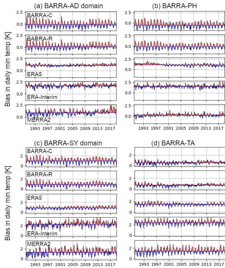
Figure 5: As with Figure 4 but for daily minimum temperature.
