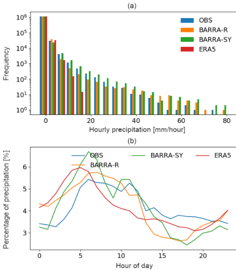
830 Figure 6: Distribution of (a) hourly rain rate (mm/h) and (b) rain over 24 hours in UTC over Sydney during November to February of 2006-2018.
