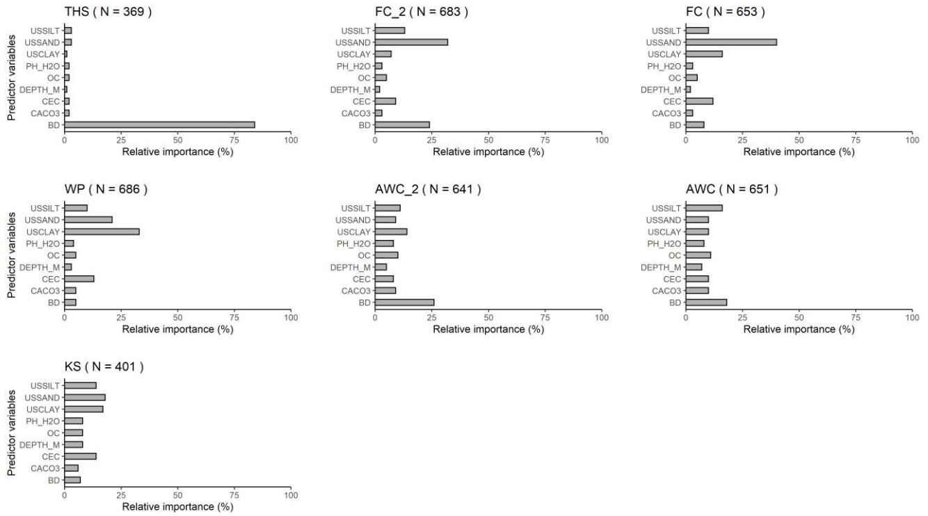
1 2 Figure 3. Relative variable importance computed with the random forest algorithm for the prediction of water content with 3 PTF32 at saturation (THS), at field capacity; -100 (FC_2) and -330 (FC) matric potential head, at wilting point (WP), of the 4 plant available water content based on FC_2 (AWC_2) and FC (AWC), and the saturated hydraulic conductivity (KS). 5 USSILT: silt content (2–50 \mu\text{m} (mass %)); USSAND: sand content (50–2000 \mu\text{m} (mass %)); USCLAY: clay content (<2 \mu\text{m} 6 (mass %)); PH_H2O: pH in water (-); OC: organic carbon content (mass %); DEPTH_M: mean soil depth (cm); OC: organic 7 carbon content (mass %); CEC: cation exchange capacity (cmol (+) \text{kg}^{-1} ); CACO3: calcium carbonate content (mass %); BD: 8 bulk density ( \text{g cm}^{-3} ).
