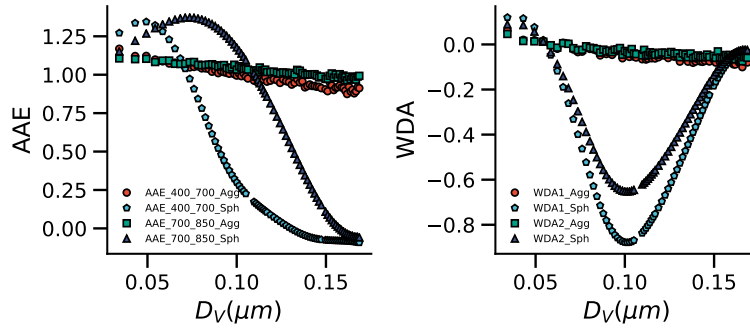
Figure 6. Comparison of AAE and WDA between BC sphere and aggregates ( D_f=1.8 , m = 1.95 + 0.79i ). Here WDA1 represents the AAE difference between the 400 - 700 nm wavelength pair and the 700 - 850 nm wavelength pair; WDA2 represents the difference between the 400 - 850 nm wavelength pair and the 700 - 850 nm wavelength pair. "Agg" and "Sph" denote the fractal BC aggregates and spherical BC, respectively.
