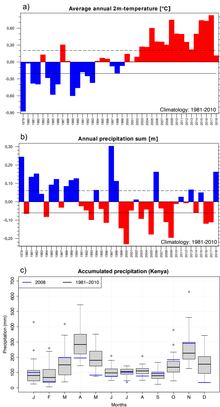
Figure 2. Annual mean 2m-temperature (a) and precipitation (b) anomalies from ERA5 (Copernicus Climate Change Service (C3S), 2017). The anomalies are calculated with respect to the climatological mean of the years 1981 to 2010. The stippled (straight) lines illustrate plus (minus) one standard deviation. Monthly accumulated values of precipitation (in mm) for the selected year 2008 (in blue), compared to the climatology (1981-2010, in grey, using a Box-Whiskers plot) are shown in (c). All values are means over the territory of Kenya in each subplot. The whiskers extend to the value that is no more than 1.5 times the inter-quartile range away from the box. The values outside this range are defined as outliers and are plotted with dots.
