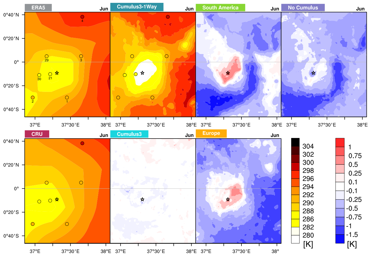
Figure 11. Same as Figs. 9 and 10 but for June 2008.
