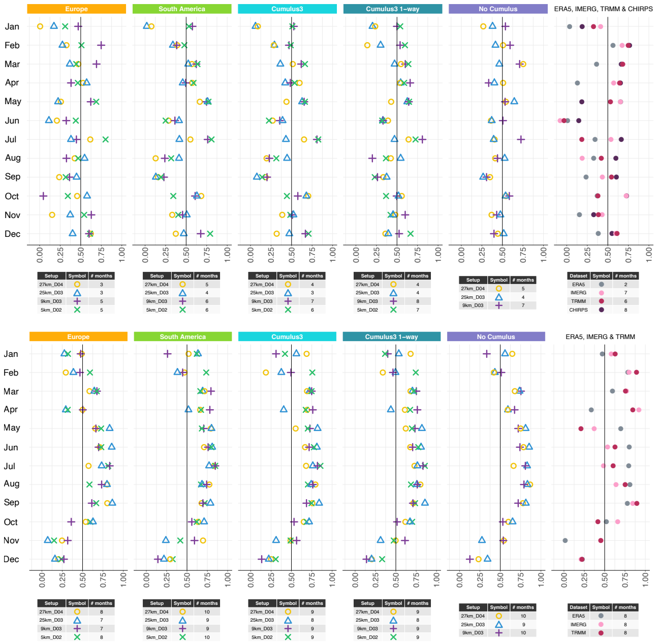
Figure 4. Pattern correlation of monthly precipitation sums between weather station data and the respective WRF simulation (upper row), and between CHIRPS (interpolated onto the respective WRF domain) and the respective WRF simulation (lower row). The different panels indicate the different parameterization options (Table 1), and the symbols stand for the different nesting options. The labelling of the symbols is given in the table below each panel, along with the number of months (# months) in which the nesting option obtain correlation patterns above the reference value of 0.50 (a moderate correlation used to visually evaluate the performance of nesting options). The last panel on each row represents the gridded data sets used throughout the paper. Even if the gridded data sets are interpolated onto different domains for each independent set-up, here only one setting is shown (27 km_D4). The rest was omitted as only marginal changes can be observed.
