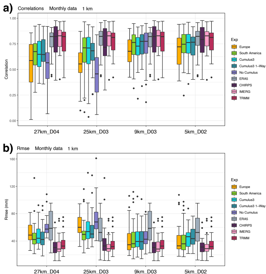
Figure 3. The temporal correlation (a) and root mean square error (RMSE) (b) between the annual cycle of measured and simulated monthly precipitation sums at the nearest grid point to the station’s location are shown for the different parameterization options (see legend to the right, Table 1), grouped by the different nesting options and number of nests. The box and whisker plots show the values in relation to 28 stations for the different domains with 1 km spatial resolution. The whiskers extend to the value that is no more than 1.5 times the inter-quartile range away from the box. The values outside this range are defined as outliers and are plotted with dots.
