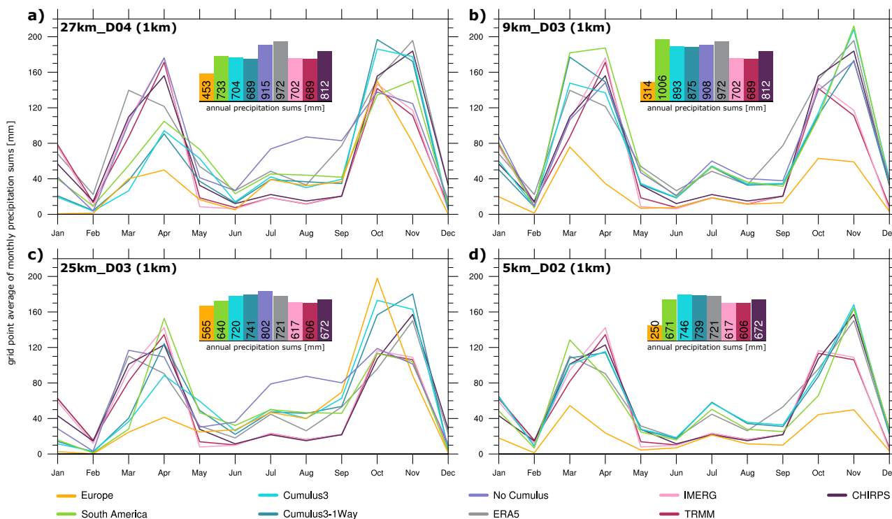
Figure 5. Grid point averages of monthly precipitation sums of the innermost domain (1 km) for each of the tested set-ups: 27 km (a), 9 km (b), 25 km (c) and 5 km (d). The 5 tested parameterization options are included, along with the driving reanalysis ERA5 and the three observational gridded data sets (IMERG, TRMM and CHIRPS). All the gridded data sets are plotted with different shades of pink, while ERA5 is colored in grey. The inset of a bar plot in each panel indicates the grid point average annual precipitation sum for each parameterization option and gridded data set.
