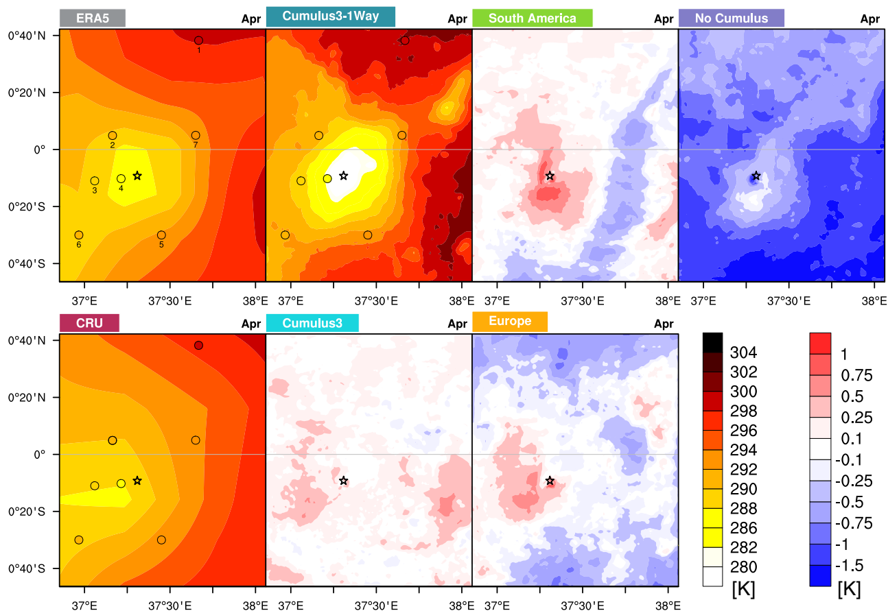
Figure 9. Monthly 2-metre temperature averages for April 2008 (‘long rains’) in K are shown for the innermost domain (1 km) of the 4 nested domain setup, with the outermost domain of 27 km resolution and a nesting ratio 1:3 for the different parameterization setups (Table 1). Absolute values are given for ERA5, CRU and the ‘Cumulus3 1-way’ option. The others depict anomalies compared to the ‘Cumulus3 1-way’ option. Weather station data are described in Table 2. The black star indicates the summit of Mount Kenya.
