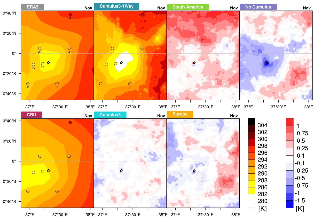
Figure 10. Same as Fig. 9 but for November 2008 ('short rains').
