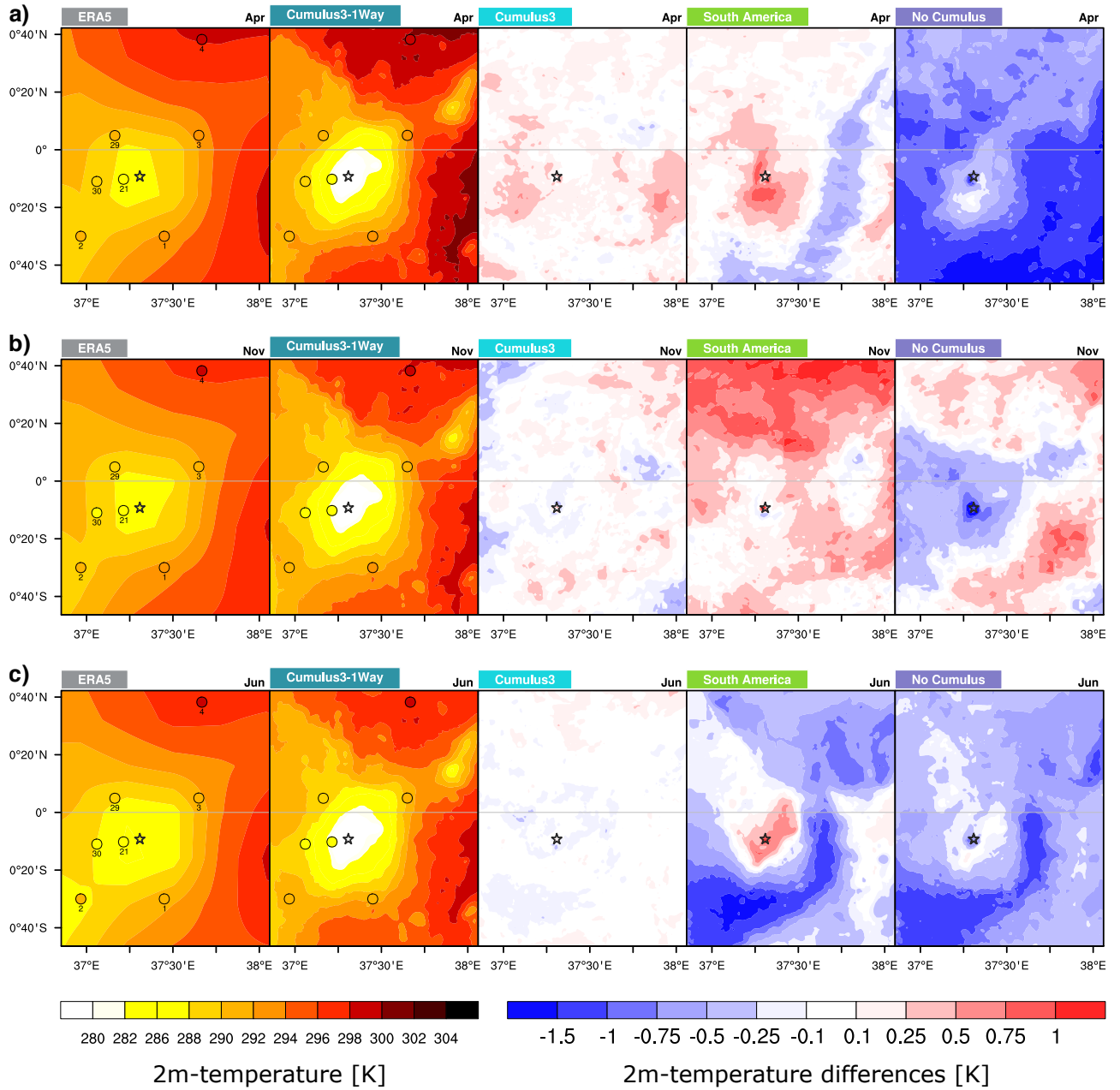
Figure 7. Same as Fig. ?? but Monthly 2-metre temperature averages for a) April 2008 ('long rains'), b) November 2008 ('short rains') and c) June 2008 (dry season) in K are shown for the innermost domain (1 km) of the 4 nested domain setup, with the outermost domain of 27 km resolution and a nesting ratio 1:3 for the different parameterization setups (Table 1). Absolute values are given for ERA5 and the "Cumulus3 1-way" option. The others depict differences compared to the "Cumulus3 1-way" option. Weather station data are described in Table 2. The black star indicates the summit of Mount Kenya.
