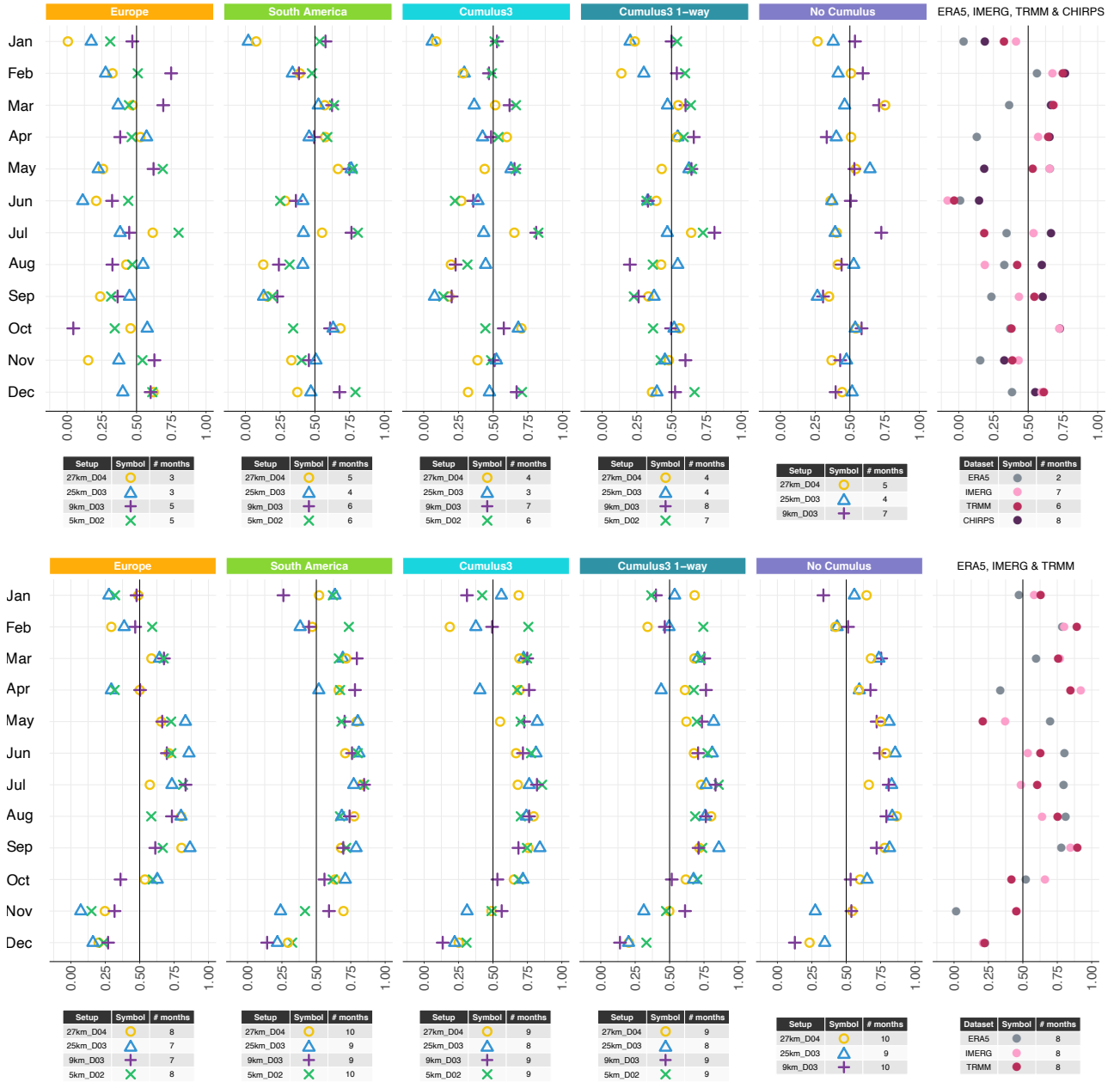
Figure 4. Pattern correlation of monthly precipitation sums of year 2008 between weather station data and the respective WRF simulation (upper row), and between CHIRPS ( interpolated onto the respective WRF domain ) and the respective WRF simulation ( interpolated onto the CHIRPS grid , lower row). The different panels indicate the different parameterization options (Table 1), and the symbols stand for the different nesting options. The labelling of the symbols is given in the table below each panel, along with the number of months (# months) in which the nesting option obtain correlation patterns above the reference value of 0.50 (a moderate correlation used to visually evaluate the performance of nesting options). The last panel on each row represents the gridded data sets used throughout the paper. Even if the gridded data sets are interpolated onto different domains for each independent set-up, here only one setting is shown (27 km_D4). The rest was omitted as only marginal changes can be observed.
