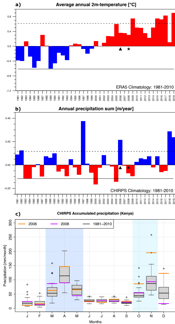
Figure 2. Annual anomalies of mean 2m-temperature (in °C) from ERA5 (Copernicus Climate Change Service (C3S), 2017) (a) and of precipitation (bin m/year) anomalies from ERA5 (Copernicus Climate Change Service (C3S), 2017) CHIRPS (Funk et al., 2015) (b). The anomalies are calculated with respect to the climatological mean of the years 1981 to 2010. The stippled (straight) lines illustrate plus (minus) one standard deviation. Monthly accumulated values of precipitation (in mm/month) for the selected year 2008 (in bluepurple ), and 2006 (in orange) compared to the climatology (1981-2010, in grey, using a Box-Whiskers plot) are shown in (c). All values are means over the territory of Kenya in each subplot. The whiskers extend to the value that is no more than 1.5 times the inter-quartile range away from the box. The values outside this range are defined as outliers and are plotted with dots. The dark and light blue shading indicates the 'long rains' and 'short rains', respectively.
