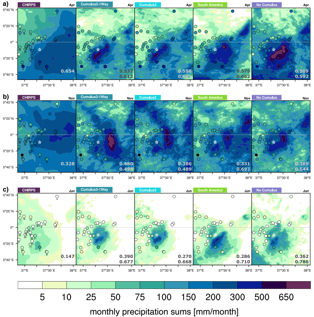
Figure 6. Monthly precipitation sums for a) April 2008 ('long rains') , b) November 2008 ('short rains') and c) June 2008 (dry season) in mm/month for the innermost domain (1 km) of the 4 nested domain setup, with the outermost domain of 27 km resolution and a nesting ratio 1:3 for the different parameterization setups (see Table 1). Weather station data are described in Table 2. The white star indicates the summit of Mount Kenya, and missing values are marked in black. The numbers in the lower right corner of each panel indicate the spatial correlation with respect to the stations (upper line) and CHIRPS (lower line).
