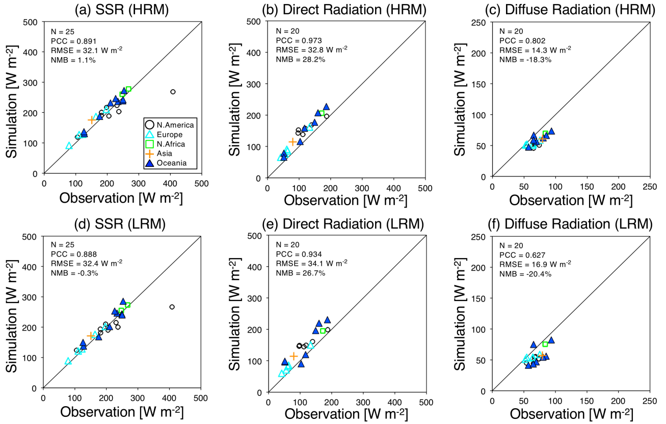
Figure 4: Scatterplots of the (a,d) surface solar radiation (SSR), (b,e) direct and (c,f) diffuse radiation fluxes between the BSRN measurements and NICAM simulations (HRM and LRM) for global annual averages. The different colors and marks reflect the sites in the different regions explained in panel (a). The numbers located in the upper-left corner in each panel represent the statistical metrics: the sampling number (N), PCC, RMSE and NMB. All units are in W m -2 .
