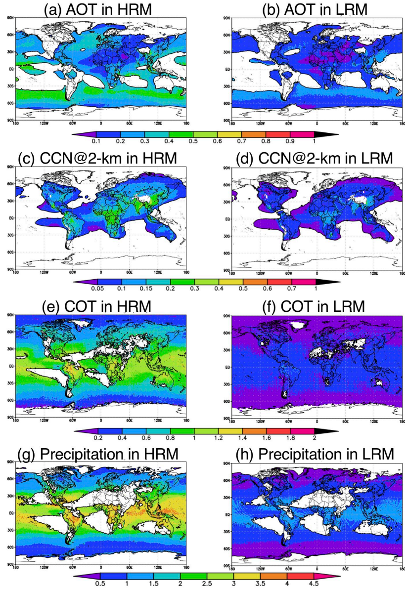
Figure 11: Global distributions of the ratio of the standard deviation to the average for the (a,b) AOT, (c,d) CCN at a height of approximately 2 km, (e,f) COT and (g,h) precipitation on 1^\circ \times 1^\circ grids using the 6-hourly output of both the HRM and LRM for a 1-year integration period. All units are in %. The transparency represents lower absolute values of each parameter: AOTs of <0.1 in panels (a,b), CCN of <40 \text{ cm}^{-3} in panels (c,d), COTs of <5 in panels (e,f), and precipitation fluxes of <1 \text{ mm day}^{-1} in panels (g,h).
