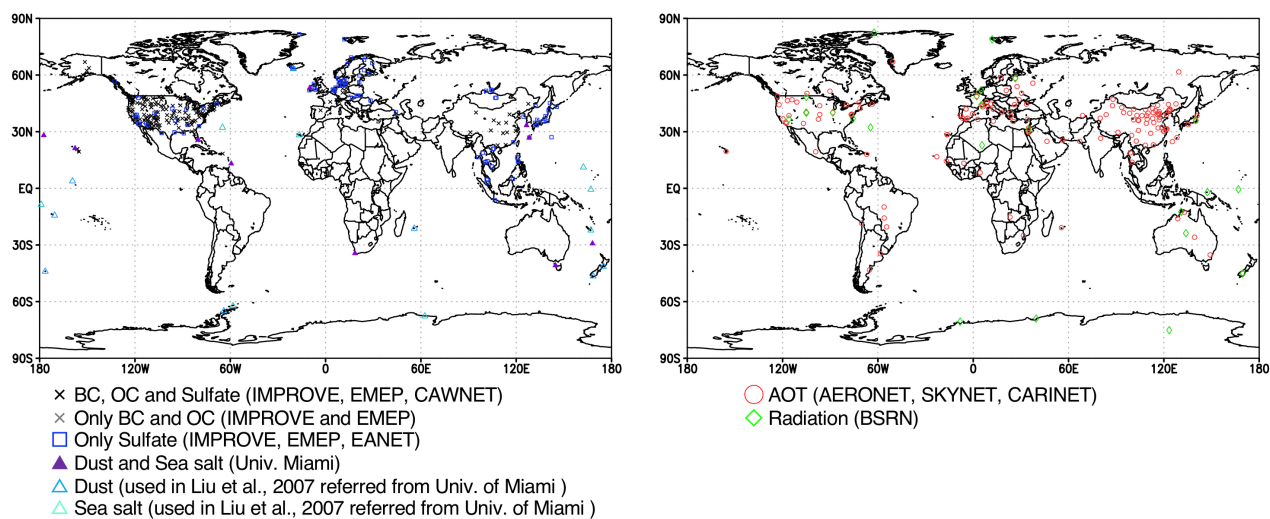
Figure 1: Global distribution of observation sites used in the model evaluation. Detailed information on these sites is provided in Tables S1-S4 in the supplementary material.
