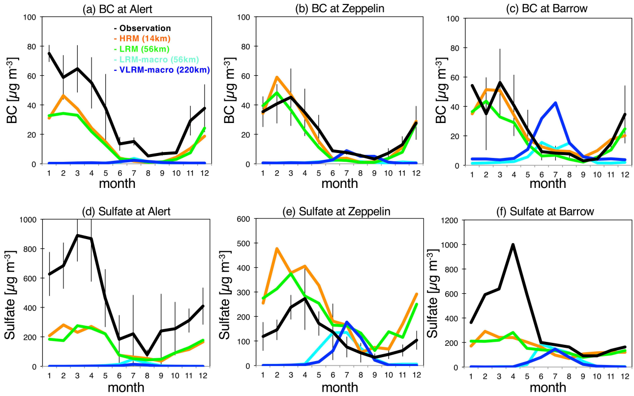
Figure 12: Monthly averages of BC and sulfate concentrations simulated by the HRM, LRM, LRM with a cloud macrophysics module (LRM-macro, which is defined in section 2.1) and VLRM-macro (NICAM simulations using a 5 horizontal grid spacing of 220 km with the cloud macrophysics module, which is defined in section 2.1) at three Arctic sites: Alert (62.3°W, 82.5°N), Zeppelin (11.9°E, 78.9°N) and Barrow (157.0°W, 71.3°N). The BC is measured as the equivalent BC at 530 nm by a particle soot absorption photometer (PSAP) for 2007-2011 under the EMEP and WDCS databases ( http://ebas.nilu.no ). The sulfate concentrations are averaged at Alert for 2000-2006 by the Canadian Aerosol Baseline Measurement (CABM) program, at Zeppelin for 2005-2013 by EMEP, and at Barrow for 10 2008-2009 by Eckhardt et al. (2015).
