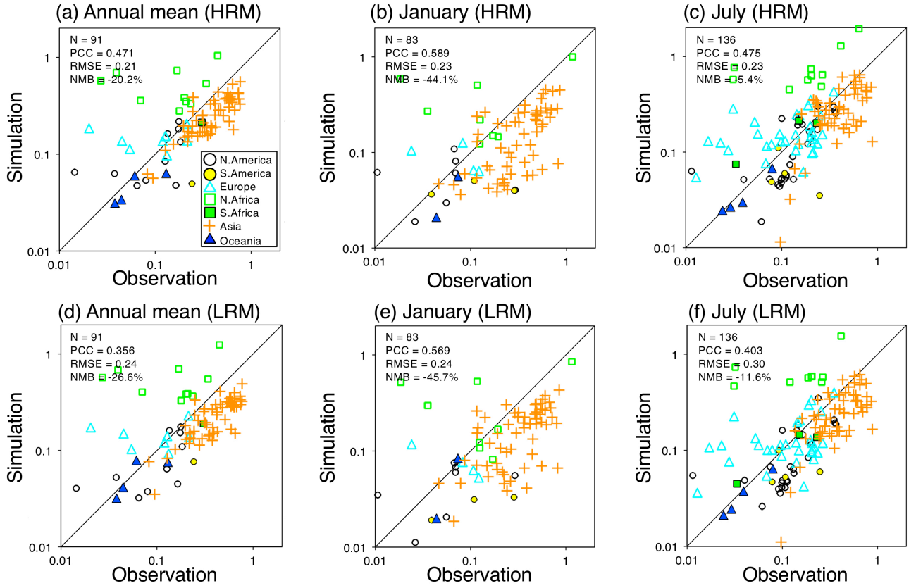
Figure 6: Scatterplot of the AOT at a wavelength of 500 nm between satellite measurements (AERONET, SKYNET, and CARSNET) and the NICAM (HRM and LRM) simulations for the annual, January and July averages. The different colors and marks reflect the sites in the different regions explained in panel (a). The numbers located in the upper-left corner in each panel represent the statistical metrics: N, PCC, RMSE and NMB. The statistical metrics are also shown in Table S5. The sites used for the comparison are shown in Figure 1.
