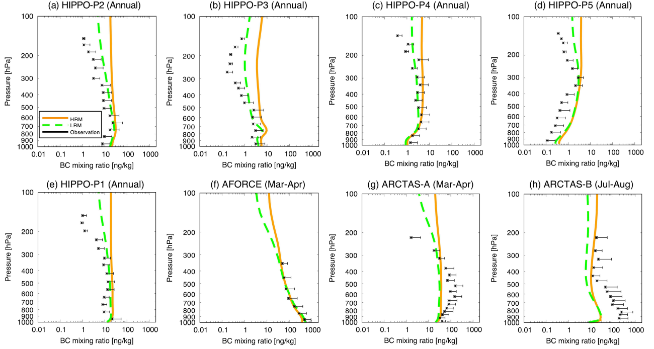
Figure 14: Vertical distribution of the BC mass concentrations from the NICAM simulations (HRM in orange and LRM in green) and from flight campaign measurements (the groups by NOAA and the University of Tokyo) in various regions and seasons. The definitions of the target domain and period in each panel are as follows: (a) 20°N-60°N, 160°E-150°W, (b) 20°S-20°N, 160°E-150°W, (c) 60°S-20°S, 160°E-150°W, (b) 60°S-80°S, 160°E-150°W, and (e) 60°N-90°N, 160°E-150°W in annual averages of 2009, (f) 32°N-37°N, 122°E-126°E in March 2012 and 26°N-32°N, 126°E-132°E in April 2012, (g) 60°N-80°N, 165°W-70°W in March-April 2008 and (h) 45°N-87°N, 135°W-45°W in July-August 2008. The abscissa shows the mass concentration in units of \mu\text{g m}^{-3} , and the ordinate shows the air pressure in units of hPa.
