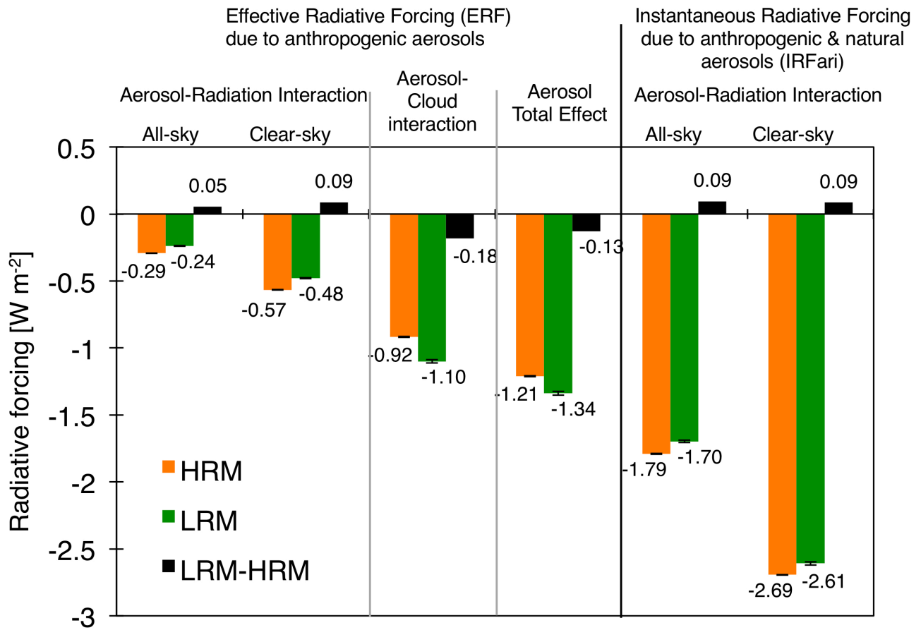
Figure 15: Annual global average ARFs for both ARIs and ACIs, i.e., IRFari, ERFari, and ERFaci, against anthropogenic and total aerosols, i.e., anthropogenic and natural sources, under all-sky and clear-sky conditions at the TOA using the HRM (orange), the LRM (green) and the difference (LRM minus HRM in black). All units are in \text{W m}^{-2} . The uncertainties are given as the global confidence intervals with a significance threshold of 95%.
