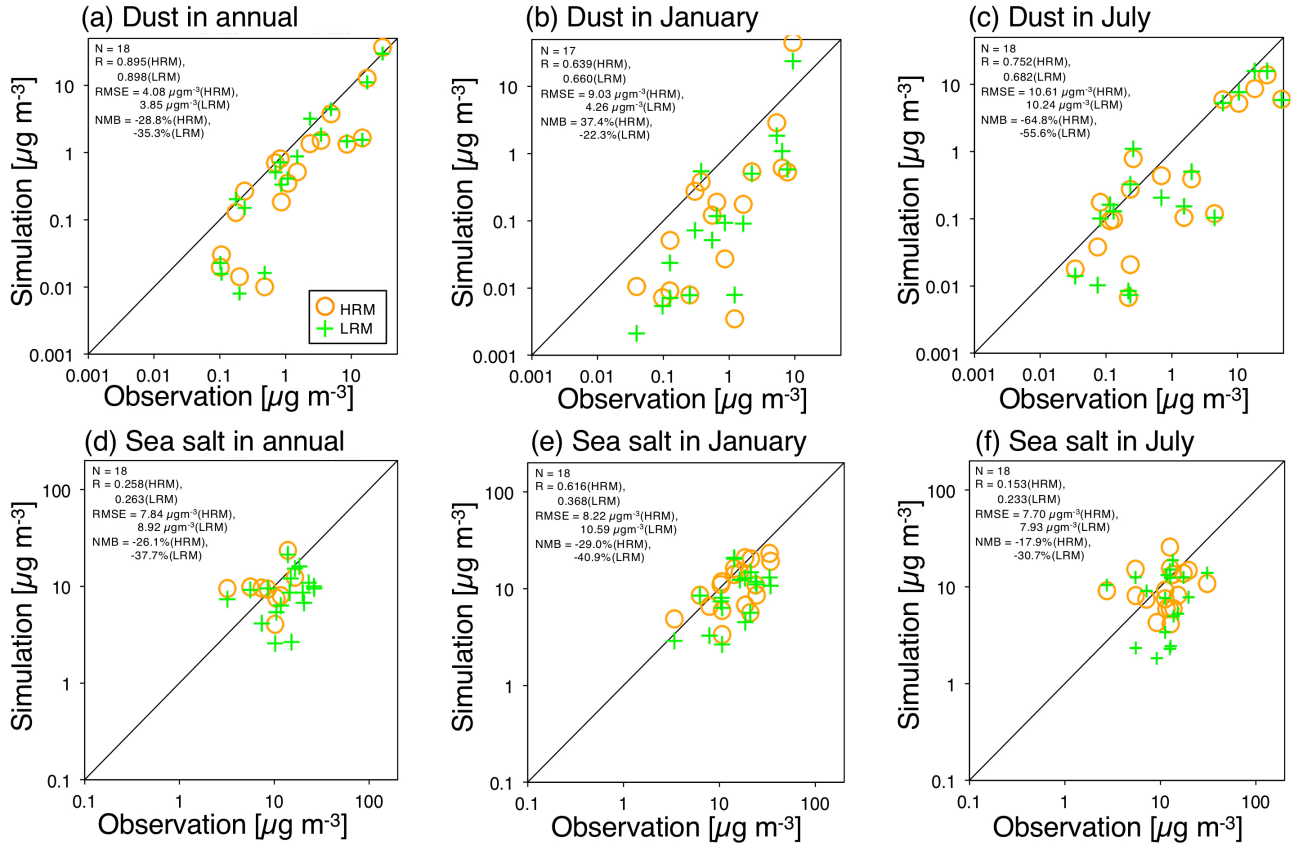
Figure 9: Scatterplots of the surface aerosol mass concentrations (dust and sea salt) between the measurements (the network managed by the University of Miami) and NICAM simulations (HRM in orange and LRM in green) for the annual, January and July averages. All units are in \mu\text{g m}^{-3} . The numbers located in the upper-left corner in each panel represent the statistical metrics: N, PCC, RMSE and NMB. The statistical metrics are also shown in Tables S7 and S8. The sites employed for the comparison are shown in Figure 1.
