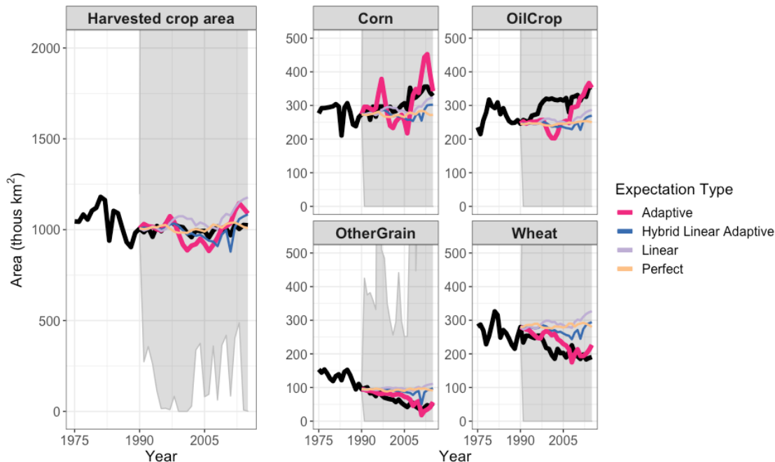
375 Figure 4: Harvested crop area (total and by crop) over time by expectation type. Black line is observations (FAO). Colored lines are gcamlan results for the models that minimize NRMSE. The expectation type with the minimum NRMSE (Adaptive) is shown with a thicker line. Gray area is the range of all gcamlan simulations. Note that fodder crops are included in gcamlan but are excluded from total cropland area in this figure due to data limitations. Figure S6 shows this same information for all 12 GCAM crop types and Figure S9 shows this for land cover types.
