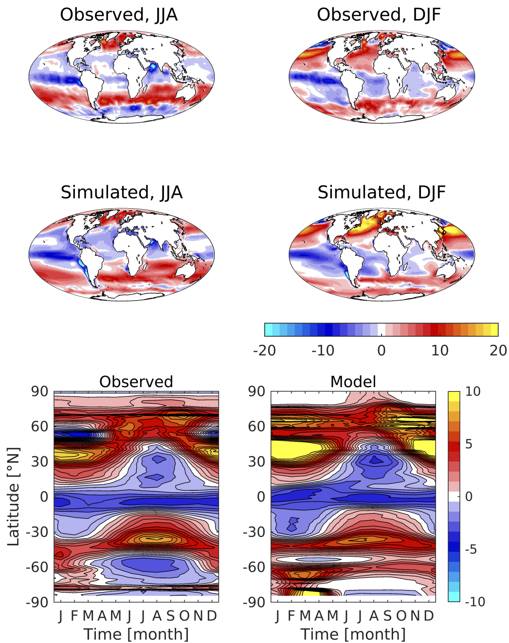
Figure 16. Observed (top; Rödenbeck et al. (2013)) and simulated (middle) air-sea \text{CO}_2 flux, shown geographically for northern (left; JJA) and southern summer (right; DJF), and as zonal Hovmöller diagrams (bottom). Red colours indicate \text{CO}_2 flux into the ocean, while blue colours denote outgassing \text{CO}_2 . Flux in \text{mmol C m}^{-2} \text{d}^{-1} .
