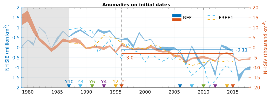
Figure 3. Anomalies of SIC (SIT) on 1 November aggregated for the NH sea ice extent (volume) in blue (red) during 1979-2018. The ensemble spread (between min and max) of REF is presented by filled area, while anomalies of FREE1 are presented by dashed lines. For AI2, the 20-year averages of anomalies taken from REF for lead year 1 (Y1, between two red triangles) are -0.11 million \text{km}^2 for SIE and -3.0 thousand \text{km}^3 for SIV (red and blue straight lines), respectively. Note that the skill assessment period is from 1997 to 2016 (see Table 2), where Y1 denotes forecast initialized from 1996, ..., 2015 and Y10 denotes the 10th year forecast initialized from 1987, ..., 2006. Thus the anomalies are more positive for predictions with longer lead years assessed, as can be seen when compared to those in Y1.
