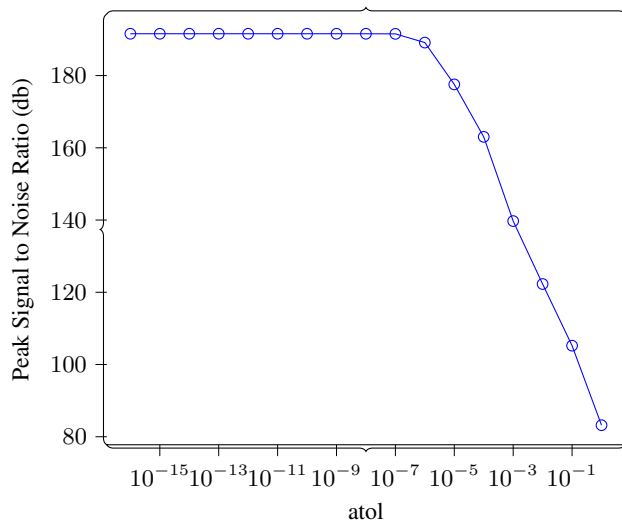
Figure 9. Gradient computation: In this experiment we carry out the full forward-reverse computation to get a gradient for a single shot, while compressing the checkpoints at different atol settings. This plot shows the PSNR of true-reference vs lossy gradient as a function of atol on the lossy checkpoints. We can see that the PSNR remains unchanged until about atol = 10^{-6} and is very high even at very high values of atol .
